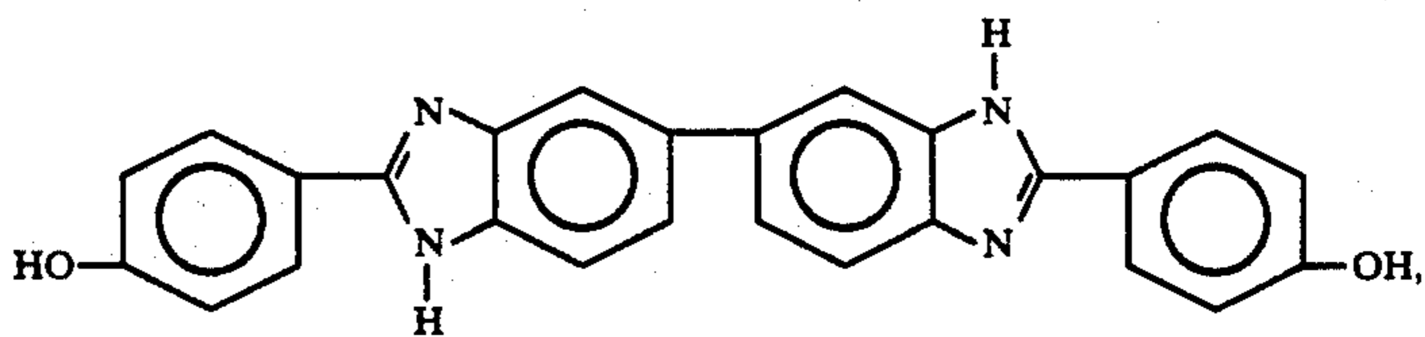
5,5'-Bis[2-(4-hydroxyphenyl)benzimidazole] a)
