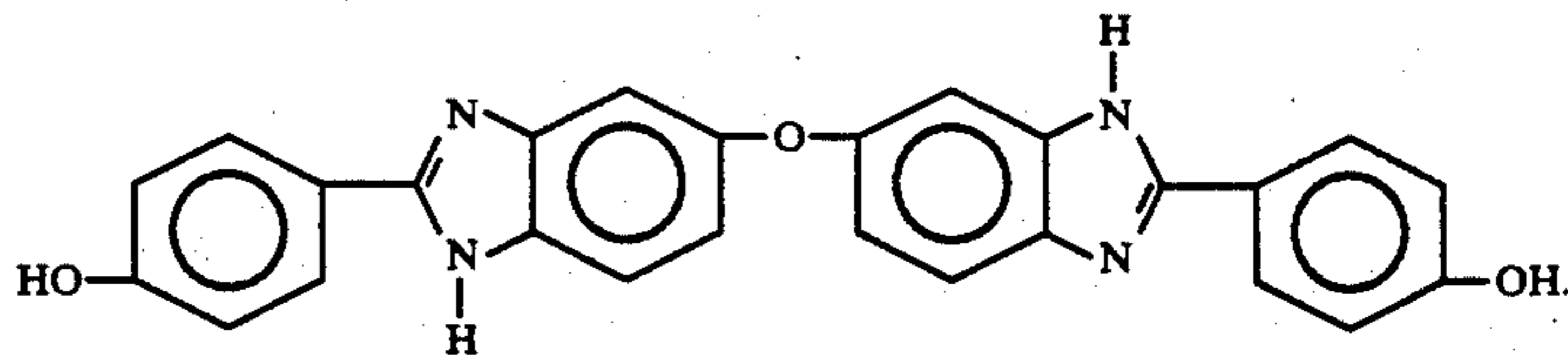
5,5'-Oxy-bis[2-(4-hydroxyphenyl)benzimidazole] c)
