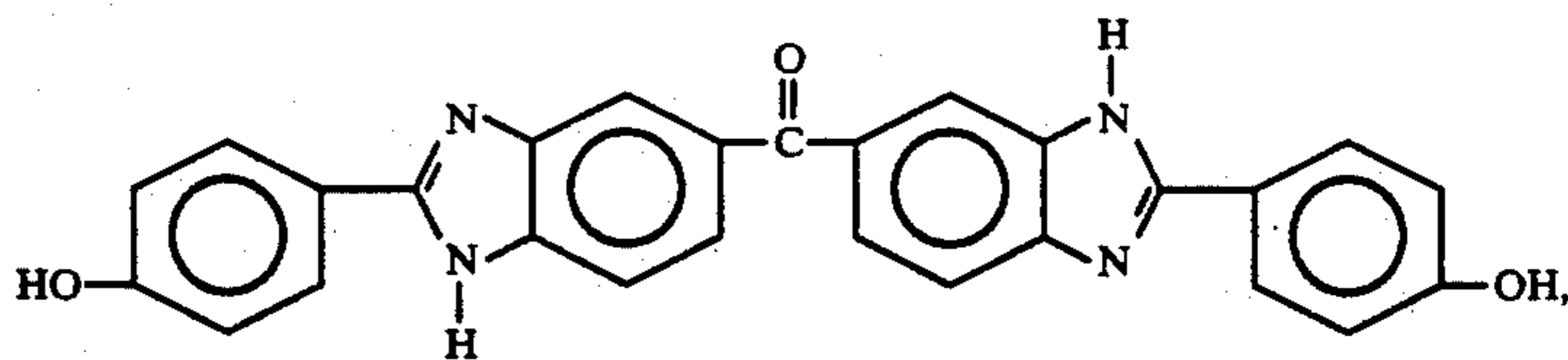
5,5'-Carbonyl-bis[2-(4-hydroxyphenyl)benzimidazole] b)
