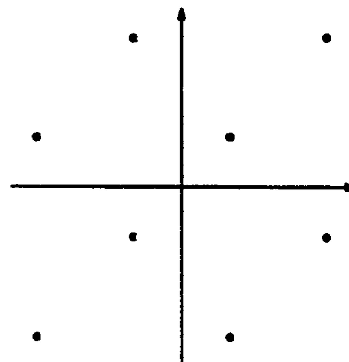
8 QAM SIGNAL CONSTELLATION
