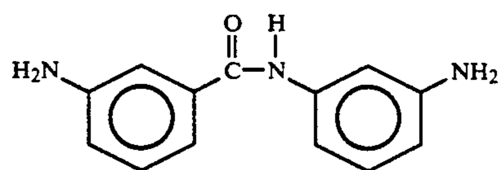
3,3'-DABA
