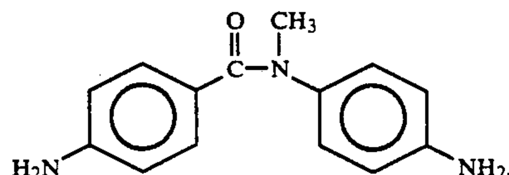
4,4'-DANMBA
