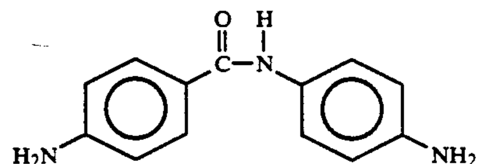
4,4'-DABA
