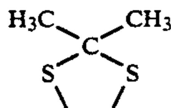
and acetonyl:
