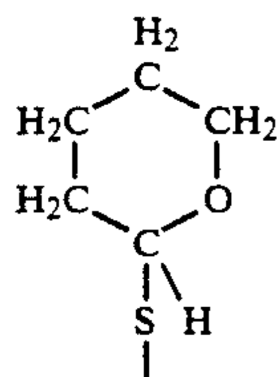
Tetrahydropyranyl
