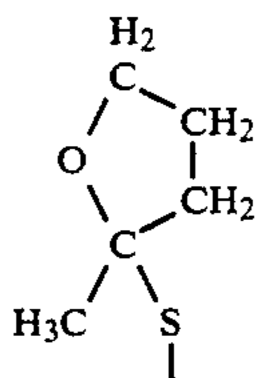
2-methyl tetrahydrofuranlyl
