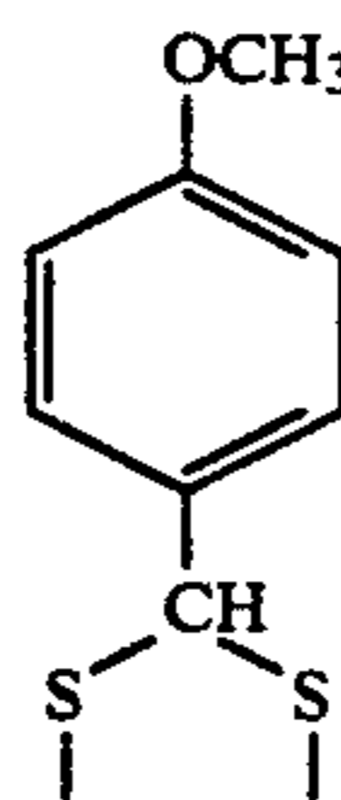
and acetonyl:
