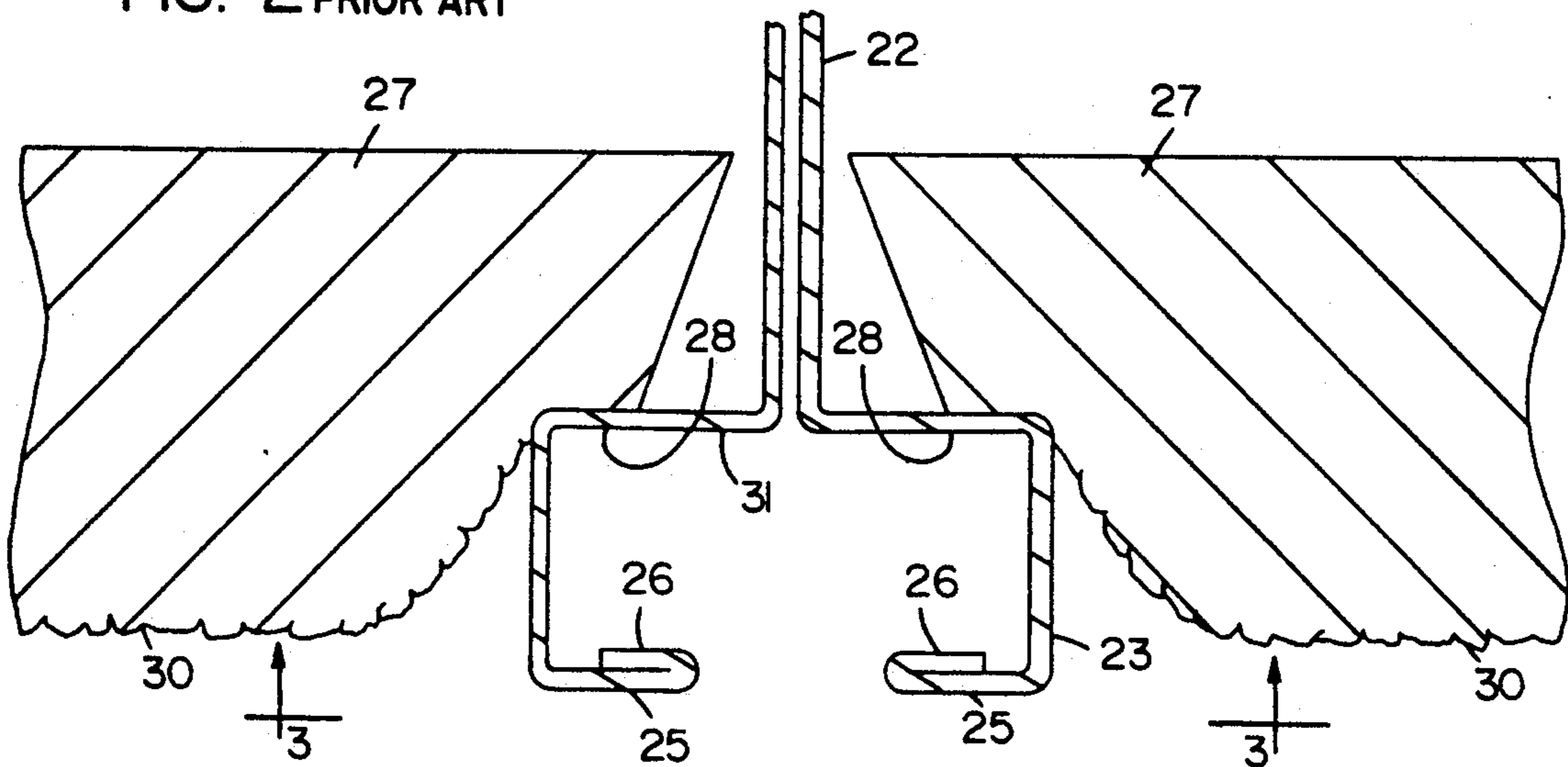
FIG. 3 PRIOR ART
