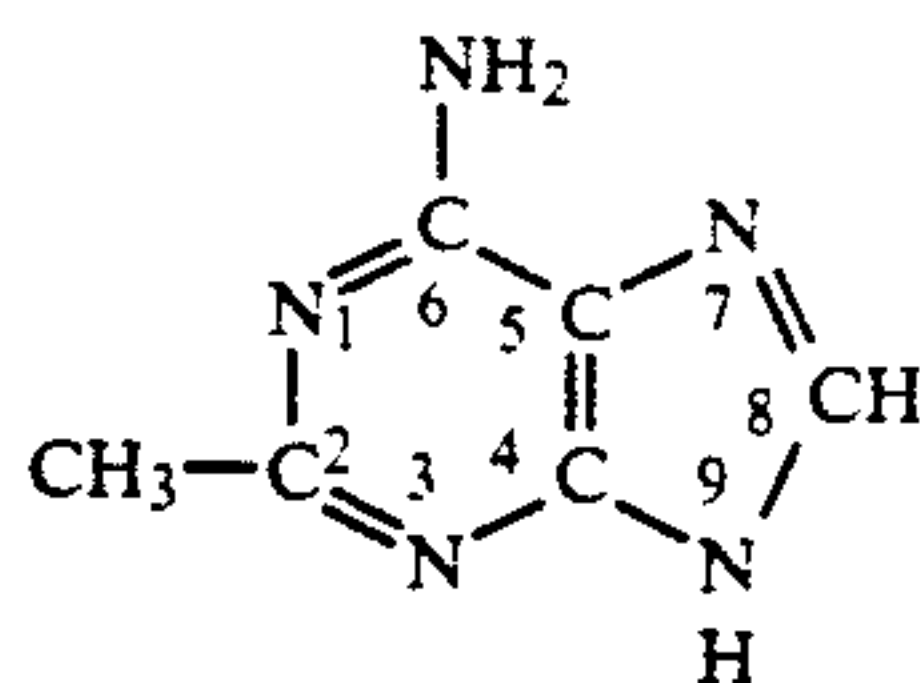
2-Methyladenine
