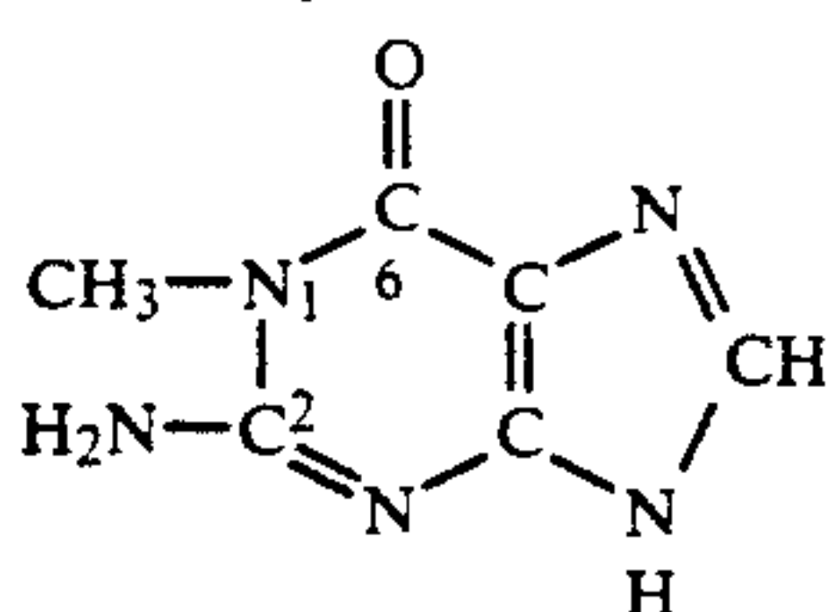
1-Methylguanine
