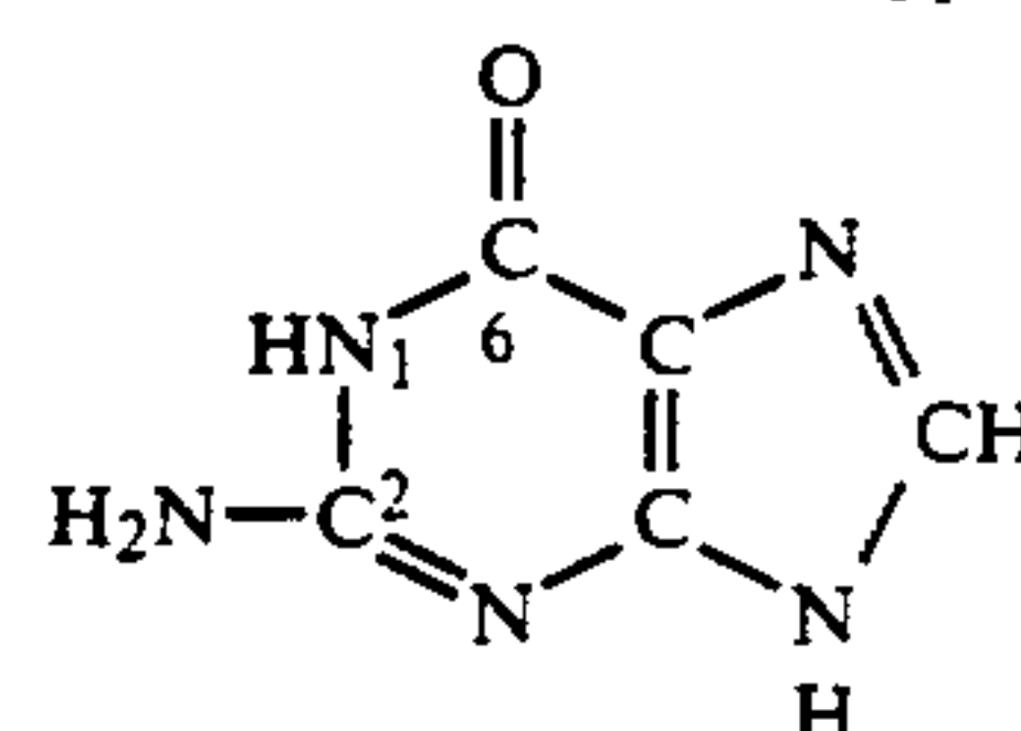
Guanine (2-amino-6-oxypurine)
