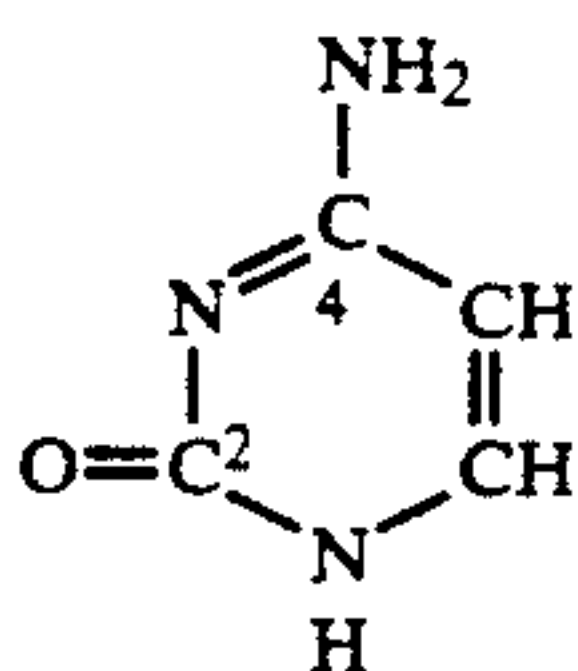
Thymine (5-methyl-2,4-dioxypyrimidine)
