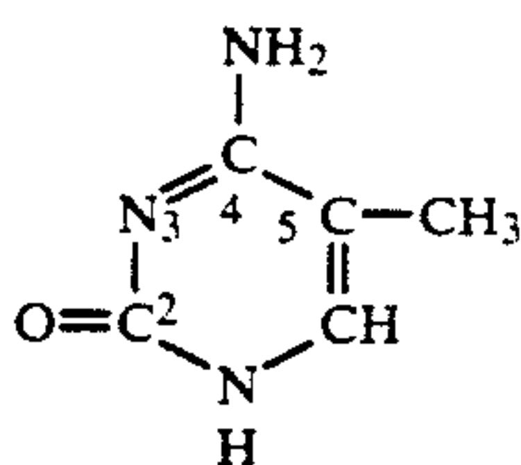
5-Methylcytosine
