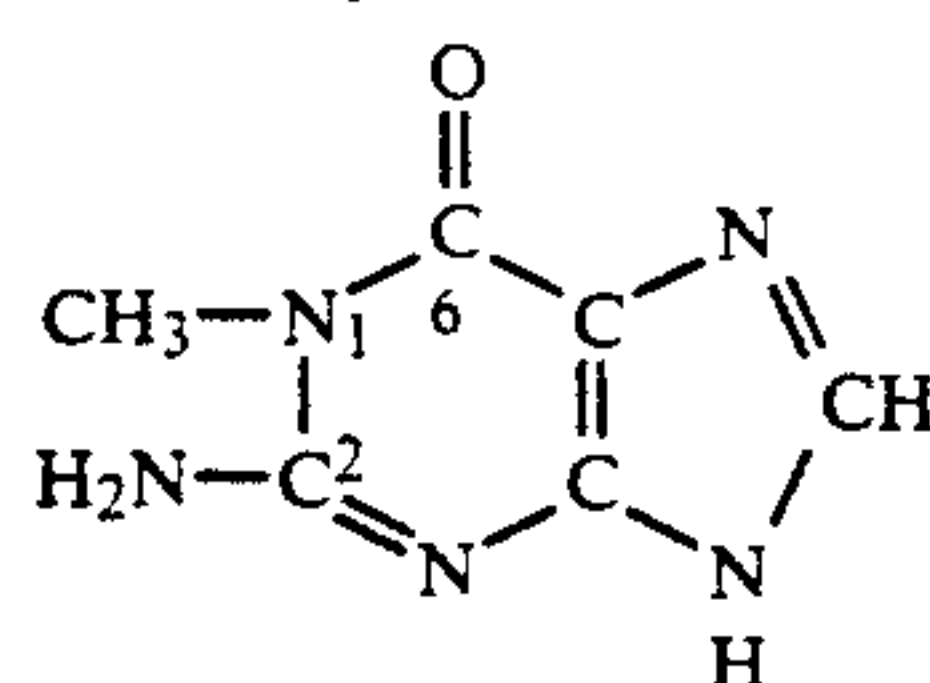
1-Methylguanine
