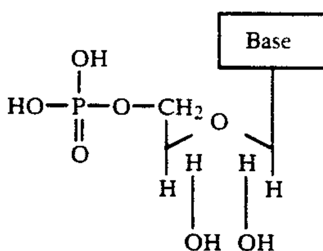
Ribonucleoside 5'-monophosphates
