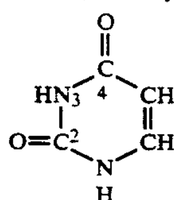
Uracil (2,4-dioxypyrimidine)
