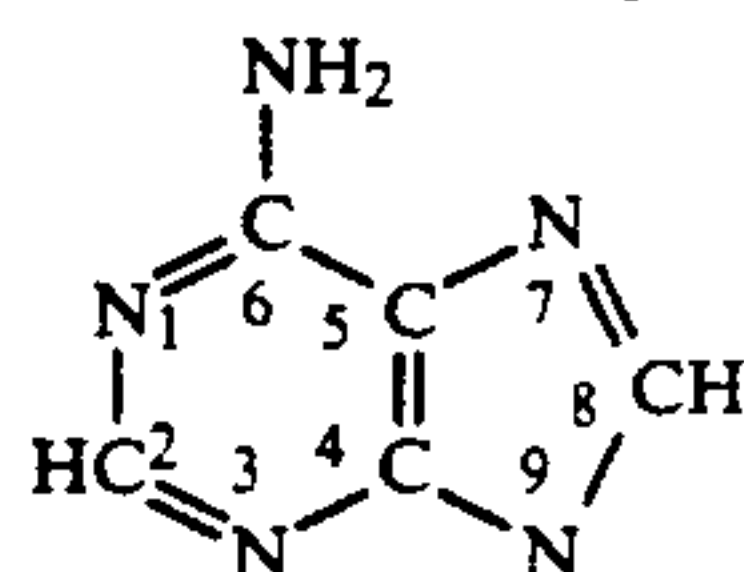
Adenine (6-aminopurine)
