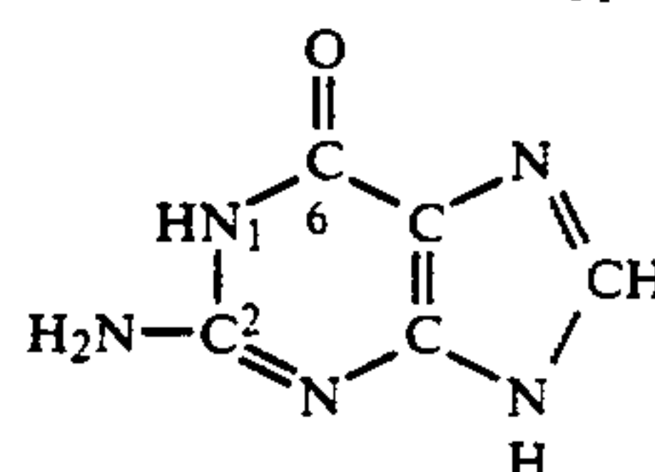
Guanine (2-amino-6-oxypurine)
