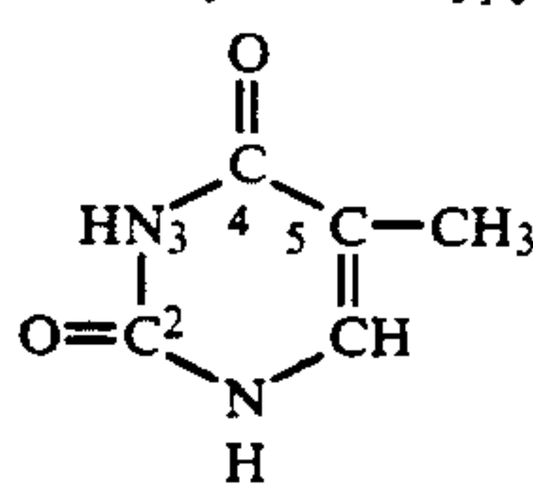
Thymine (5-methyl-2,4-dioxypyrimidine)
