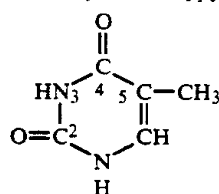
Thymine (5-methyl-2,4-dioxypyrimidine)
