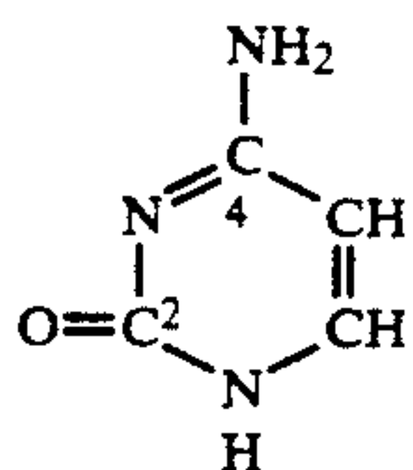
Thymine (5-methyl-2,4-dioxypyrimidine)
