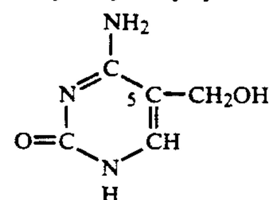
5-Hydroxymethylcytosine
