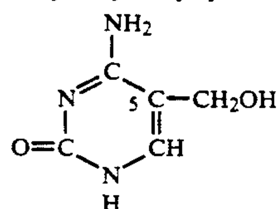
5-Hydroxymethylcytosine
