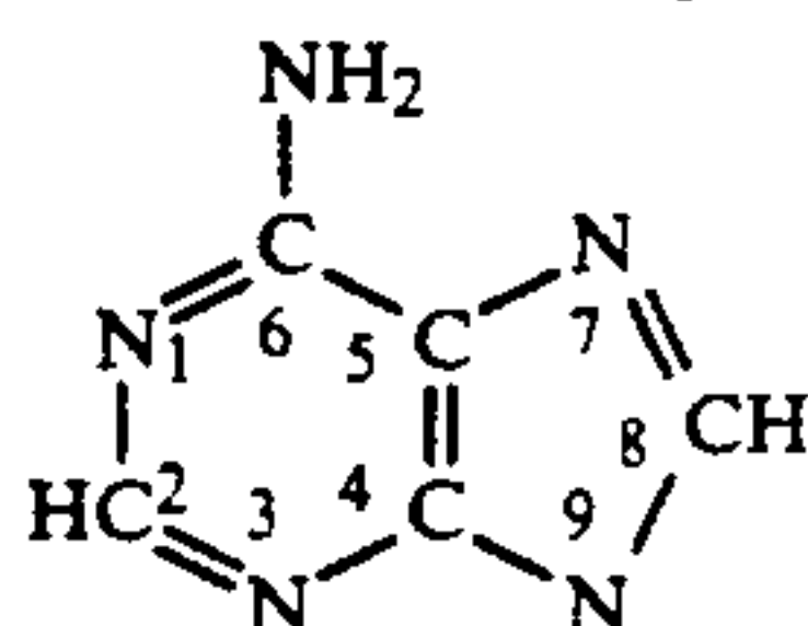
Adenine (6-aminopurine)
