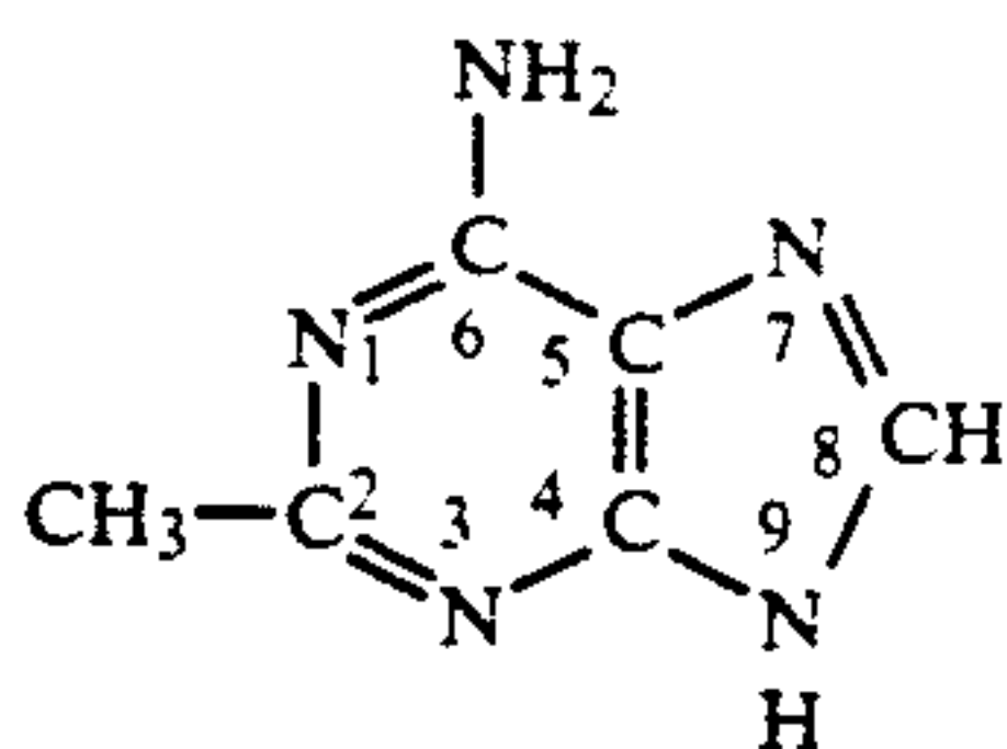
2-Methyladenine
