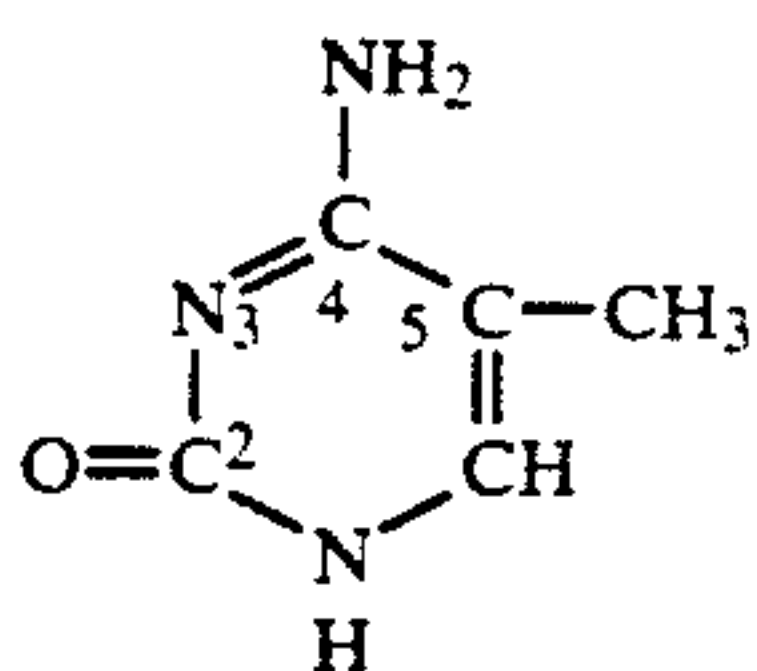
5-Methylcytosine
