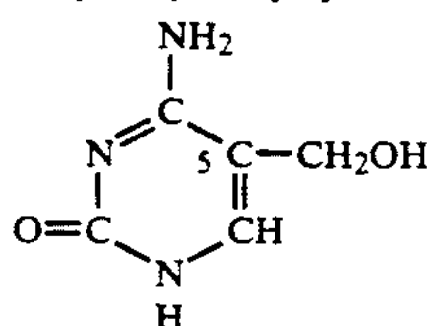
5-Hydroxymethylcytosine
