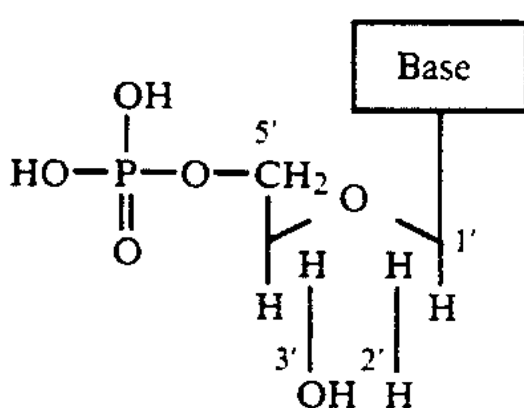
2'-Deoxyribonucleoside 5'-monophosphates
