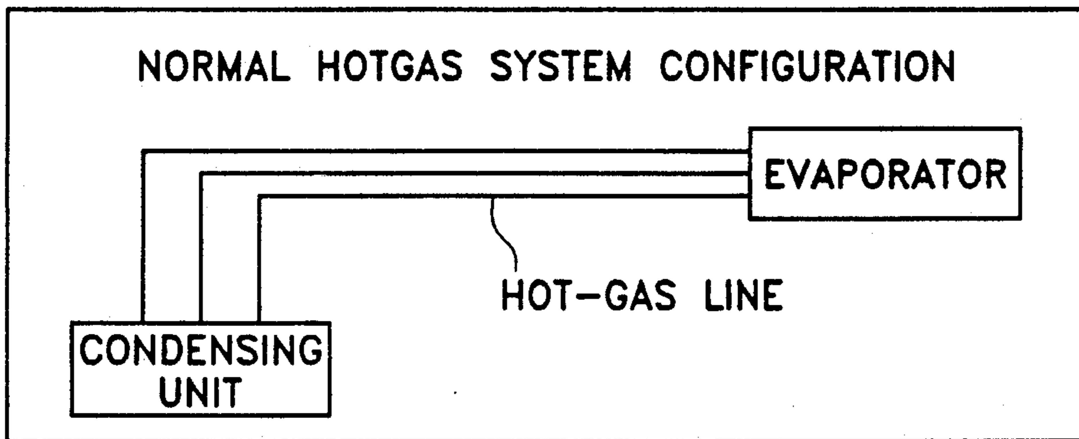
Fig. 4 (PRIOR ART)
