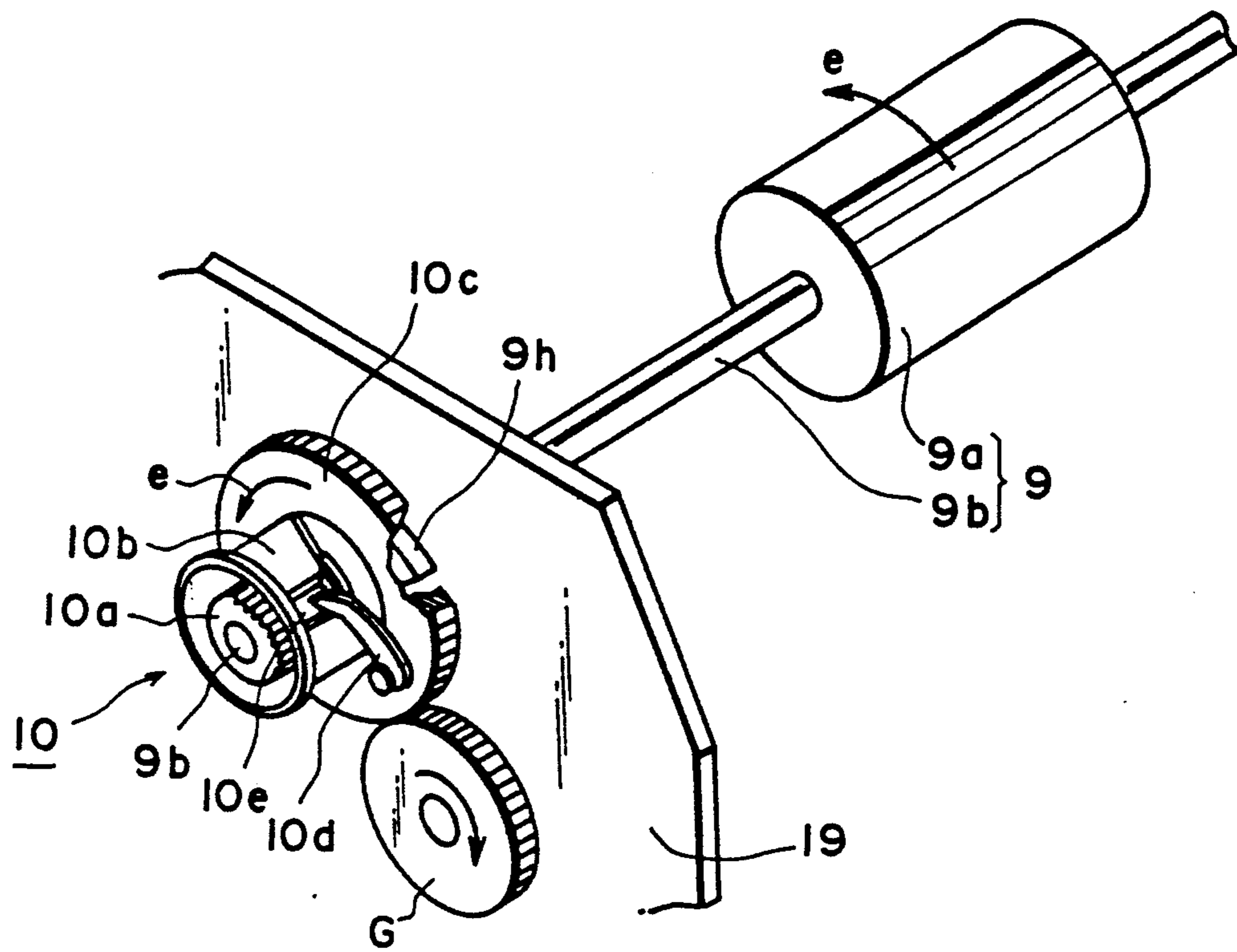
CLUTCH ON
