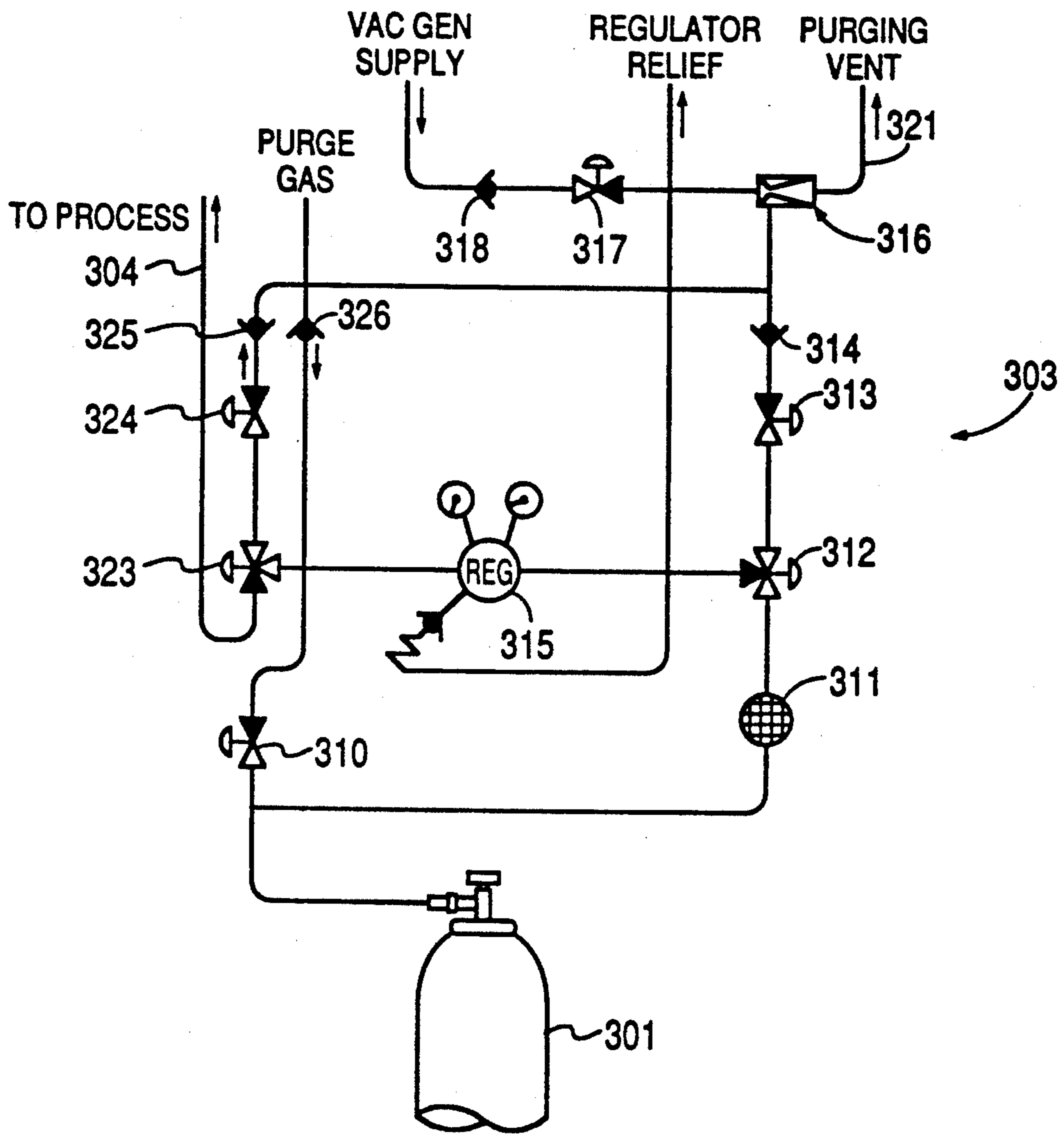
FIG. 3 (PRIOR ART)
