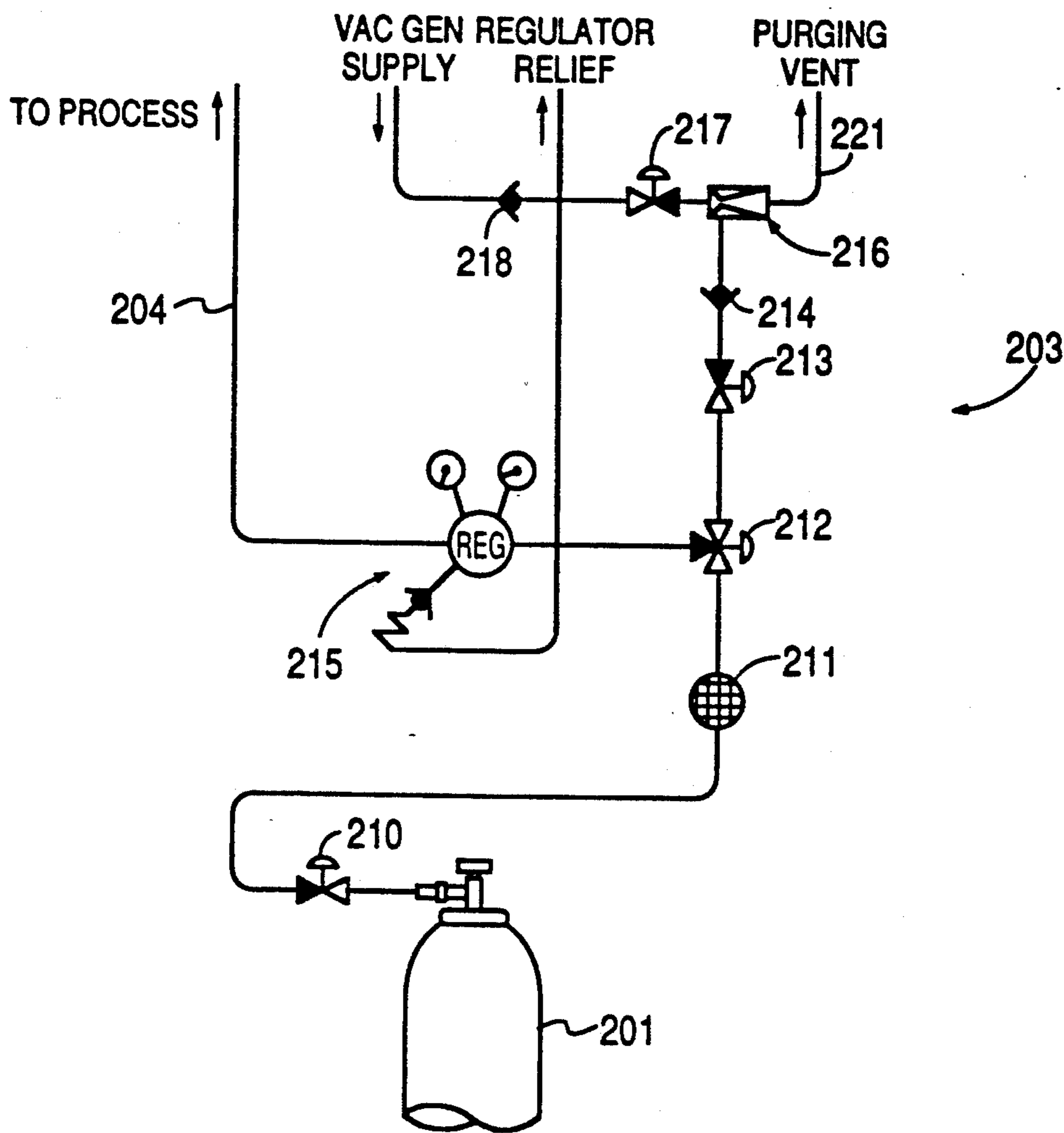
FIG. 2 (PRIOR ART)
