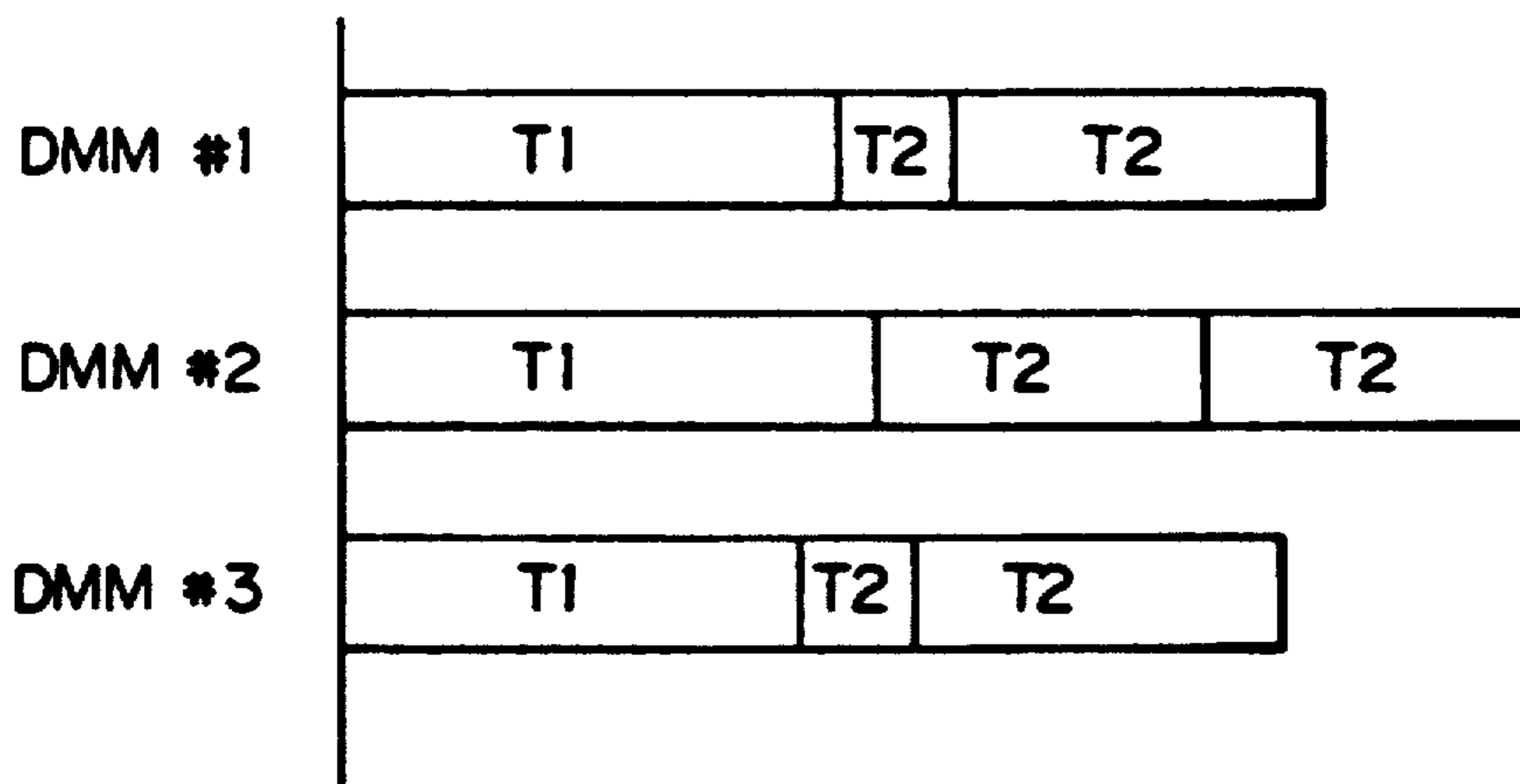
OPERATION EXAMPLE OF DMM
