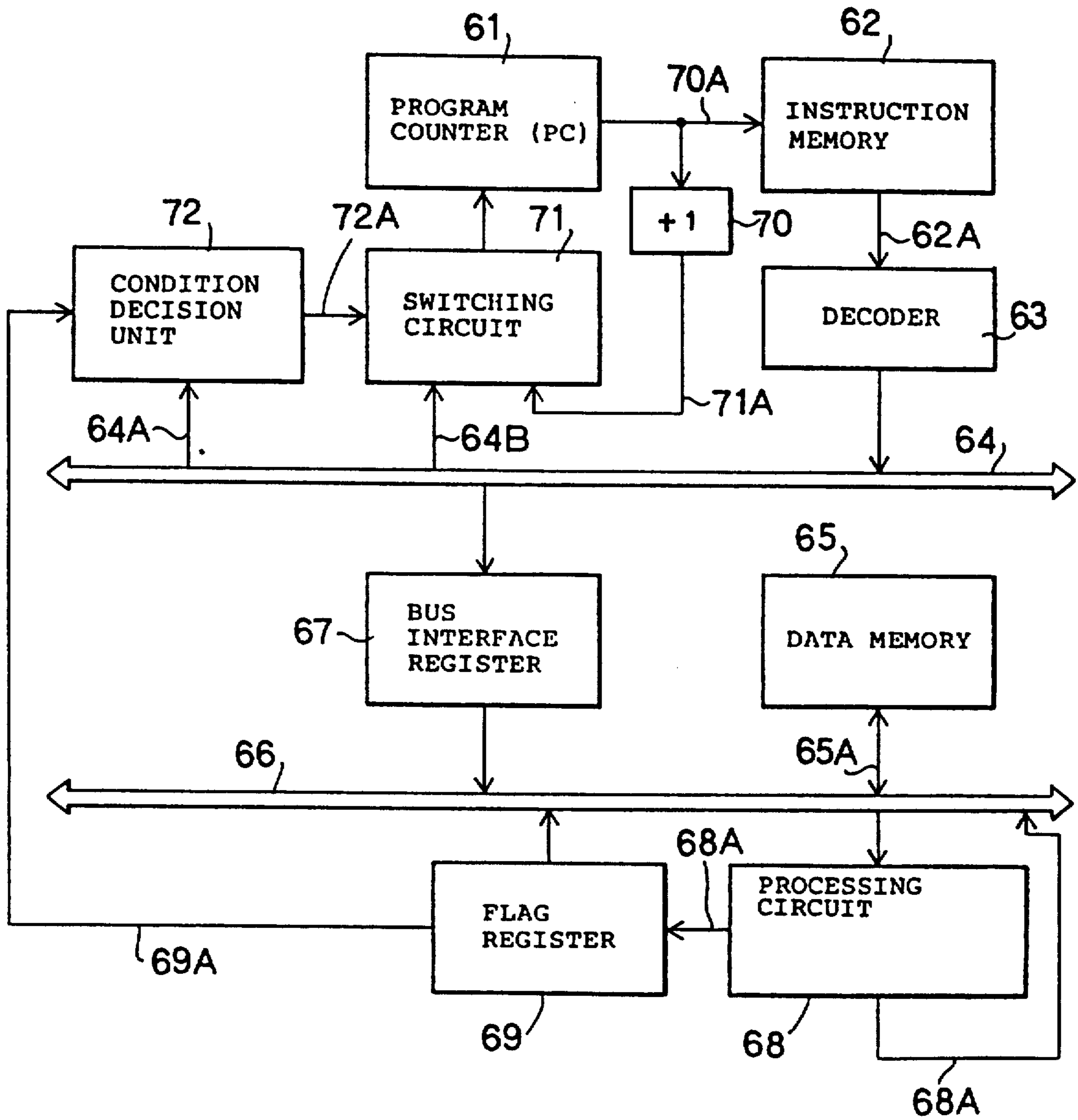
FIG. 6 (PRIOR ART)
