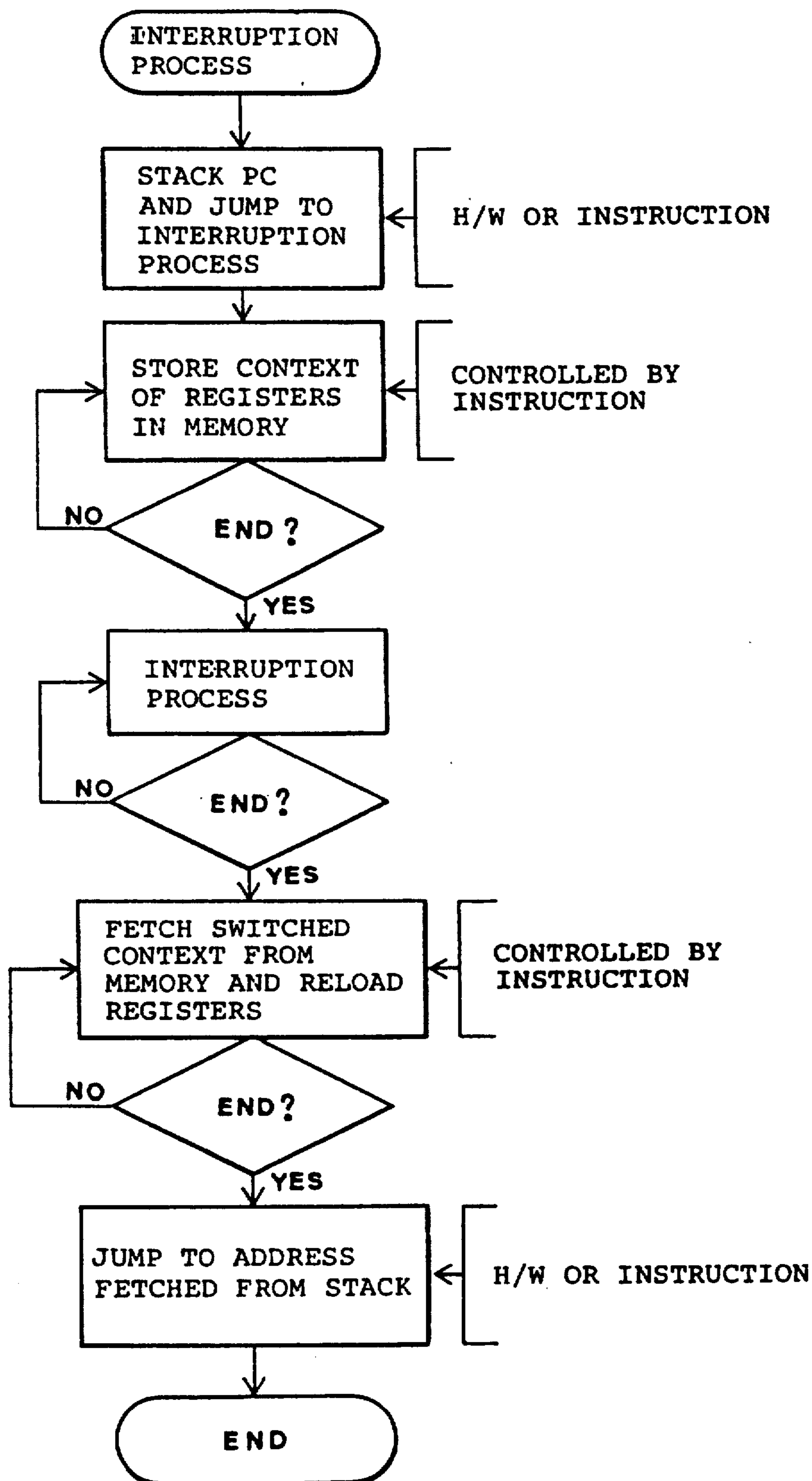
FIG. 14 (PRIOR ART)
