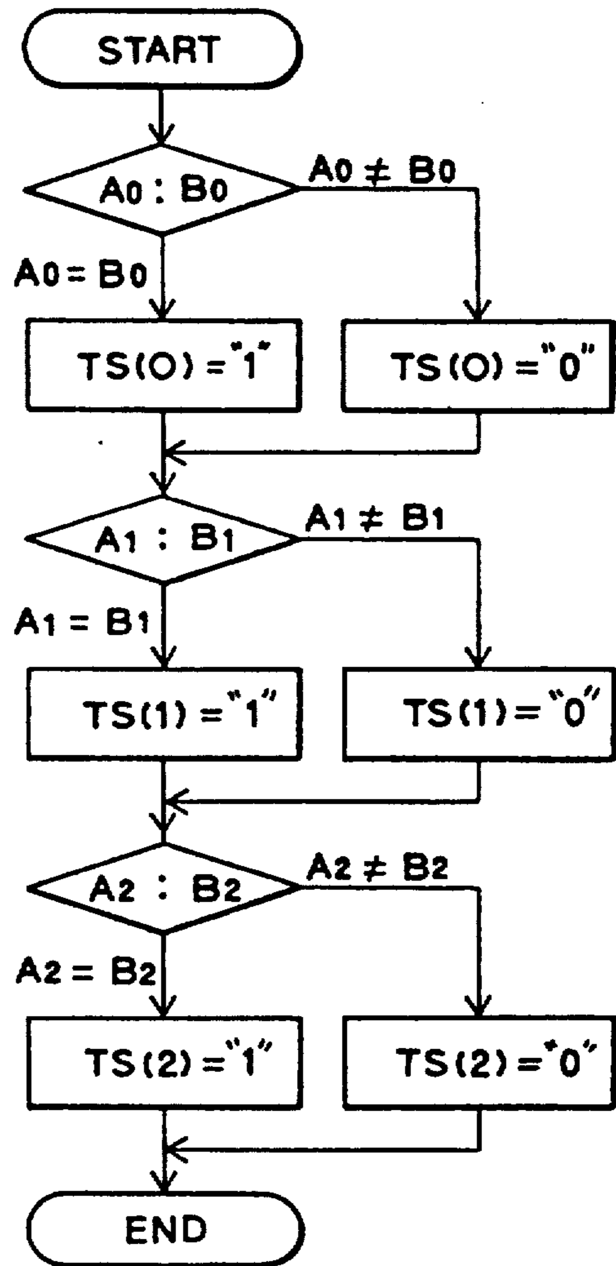
FIG. 7 (PRIOR ART)
