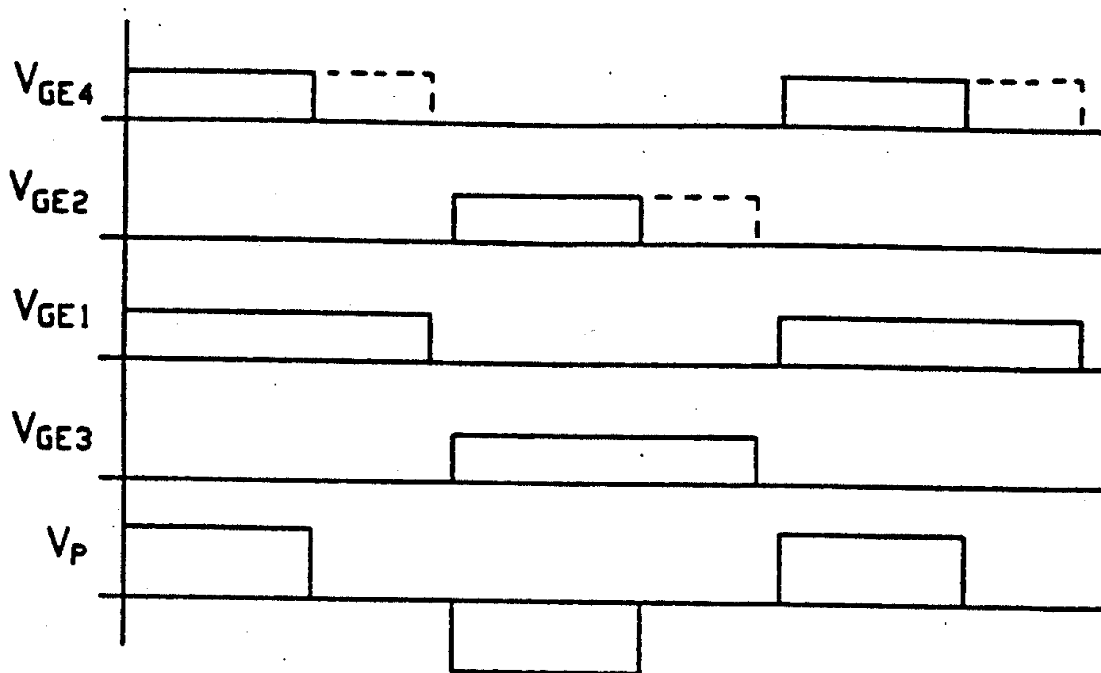
TIMING DIAGRAM
