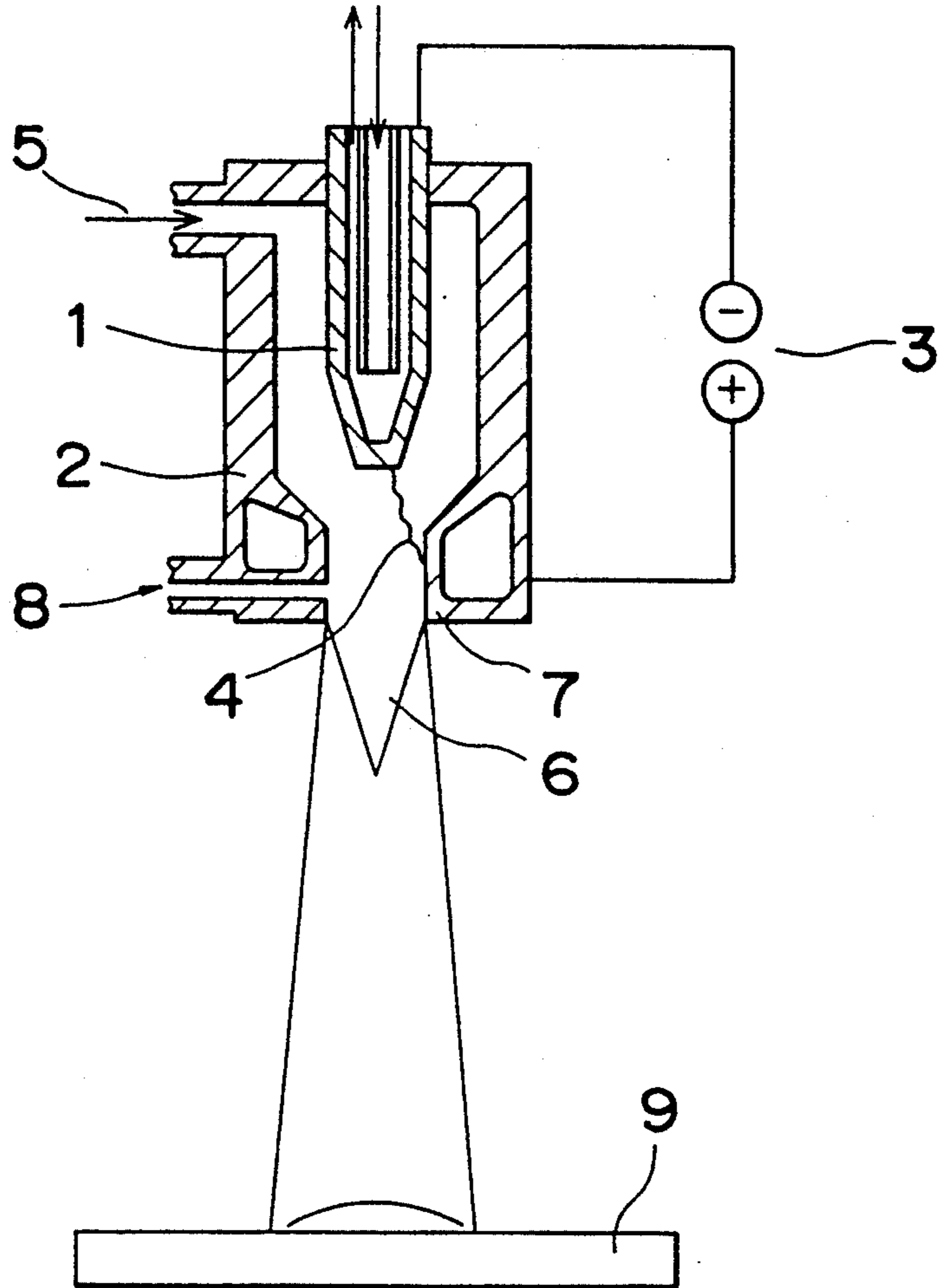
Fig. 1 PRIOR ART
