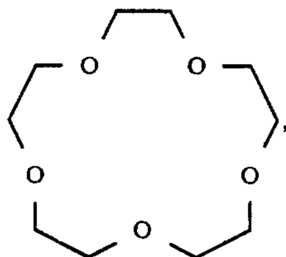
15-crown-5 ether;
