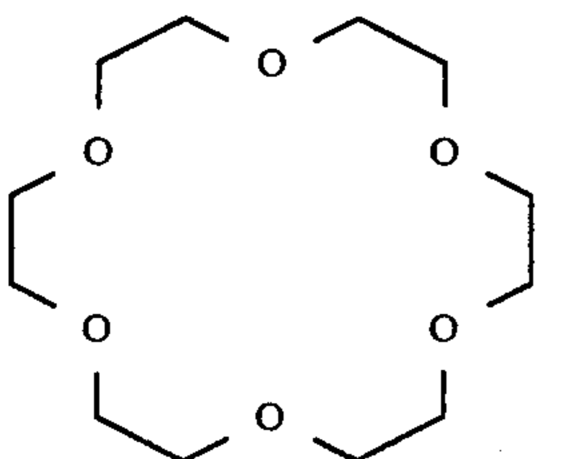
18-crown-6 ether;
