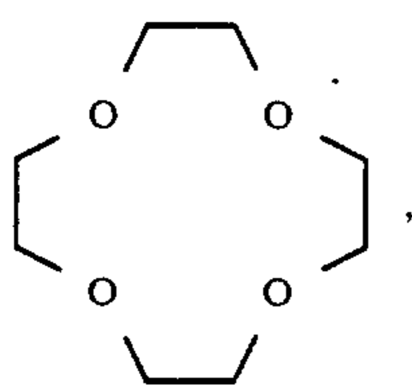
12-crown-4 ether;
