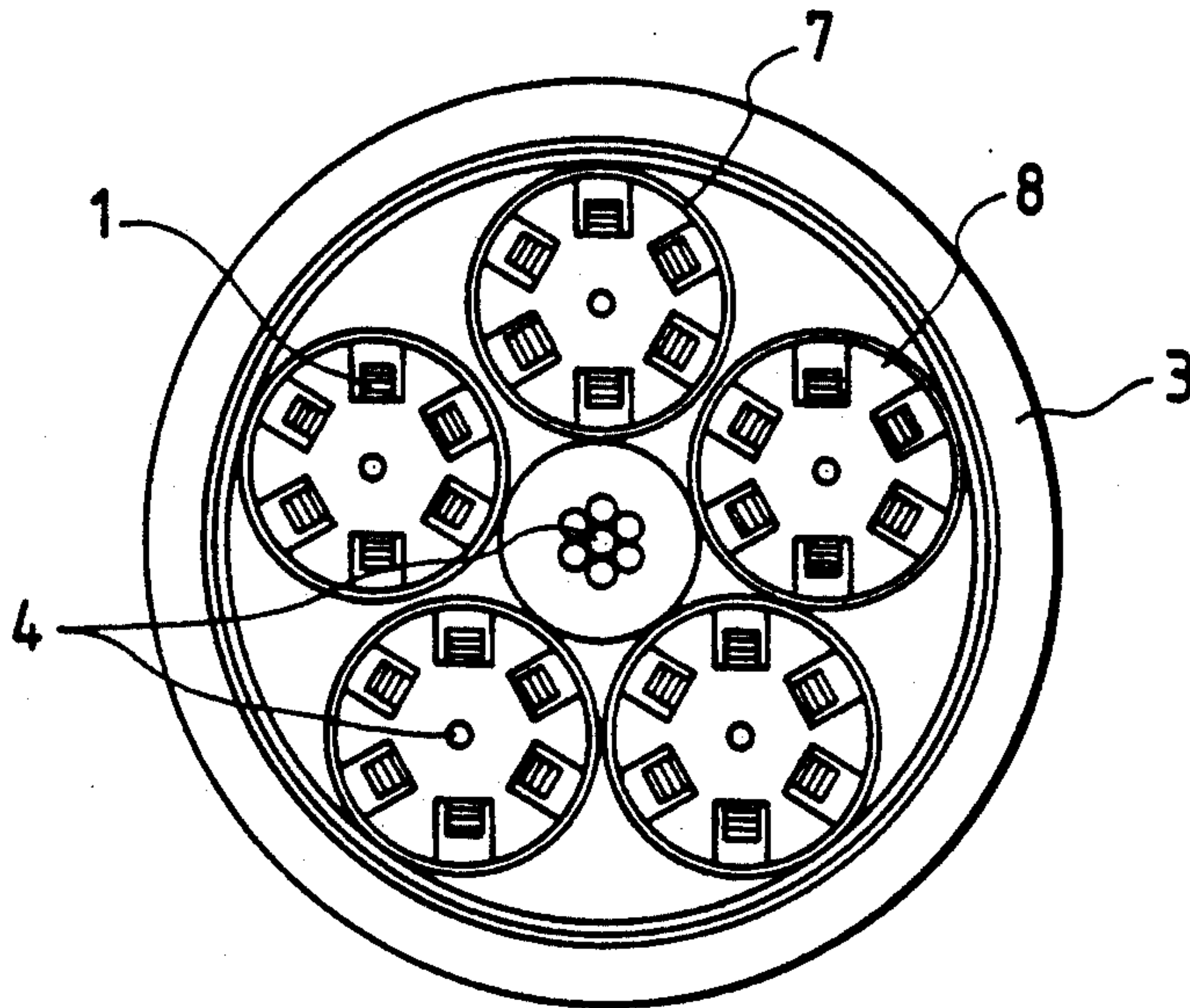
FIG. 5 (PRIOR ART)
