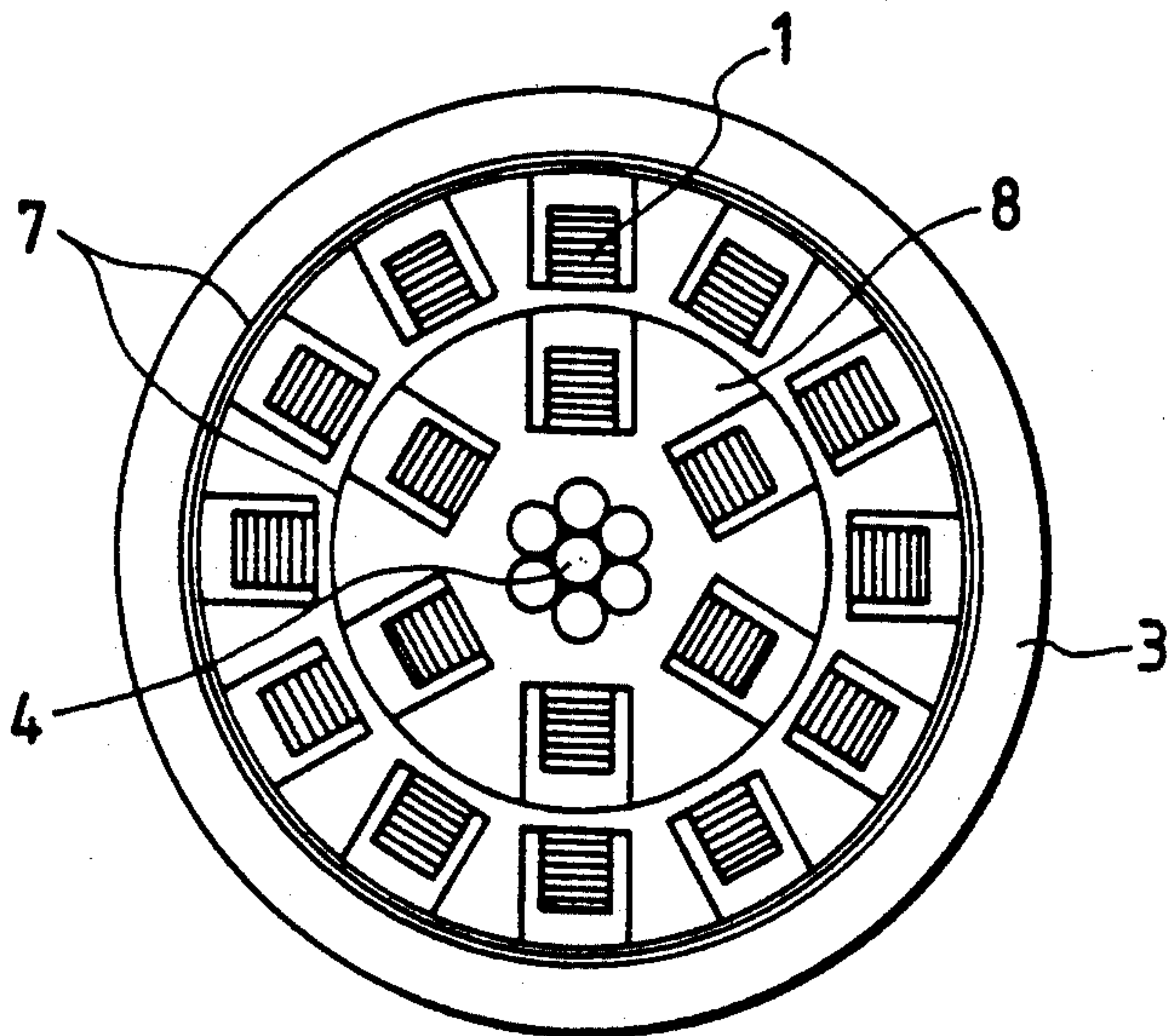
FIG. 7 (PRIOR ART)
