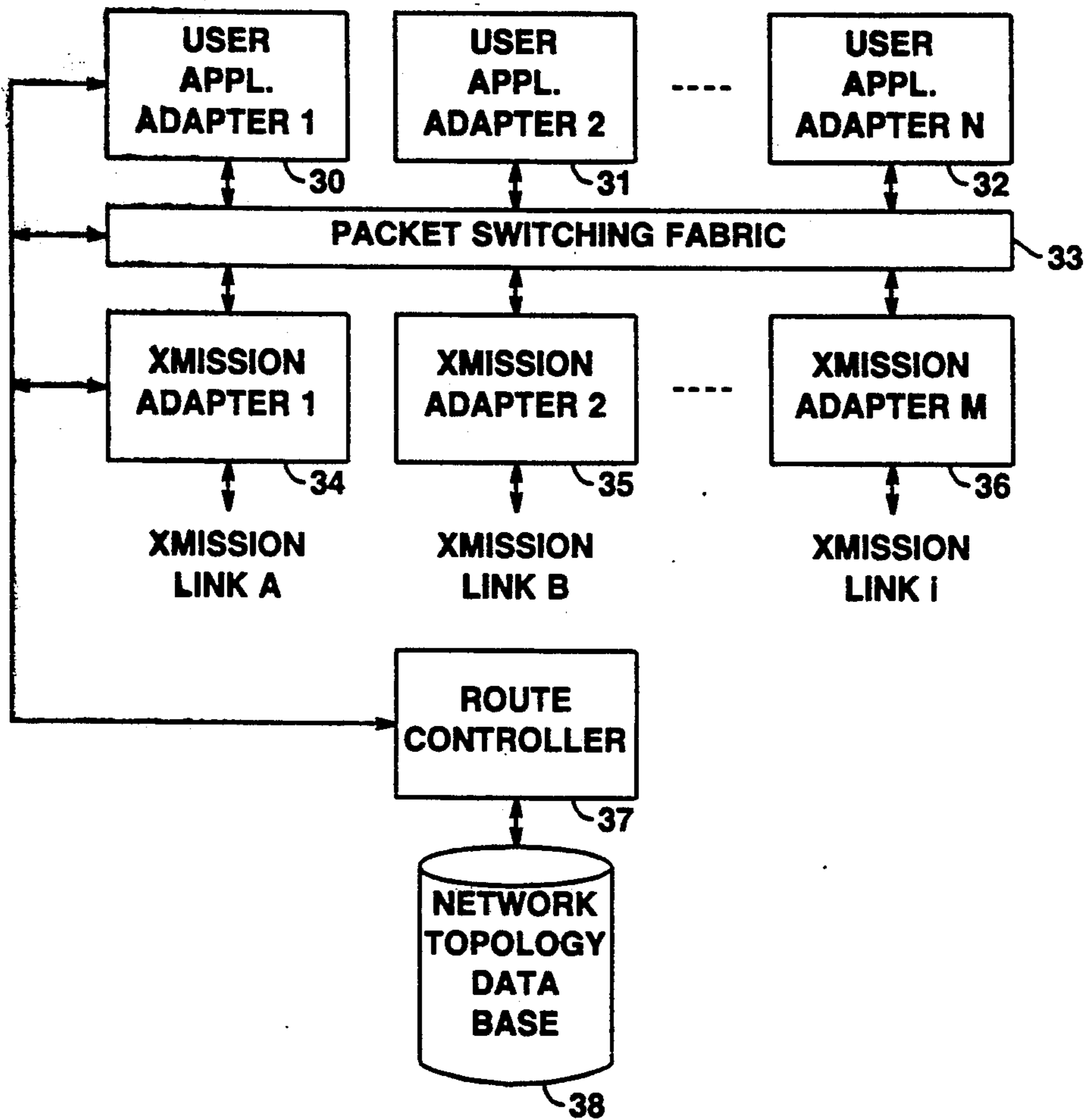
TYPICAL PACKET DECISION POINT
