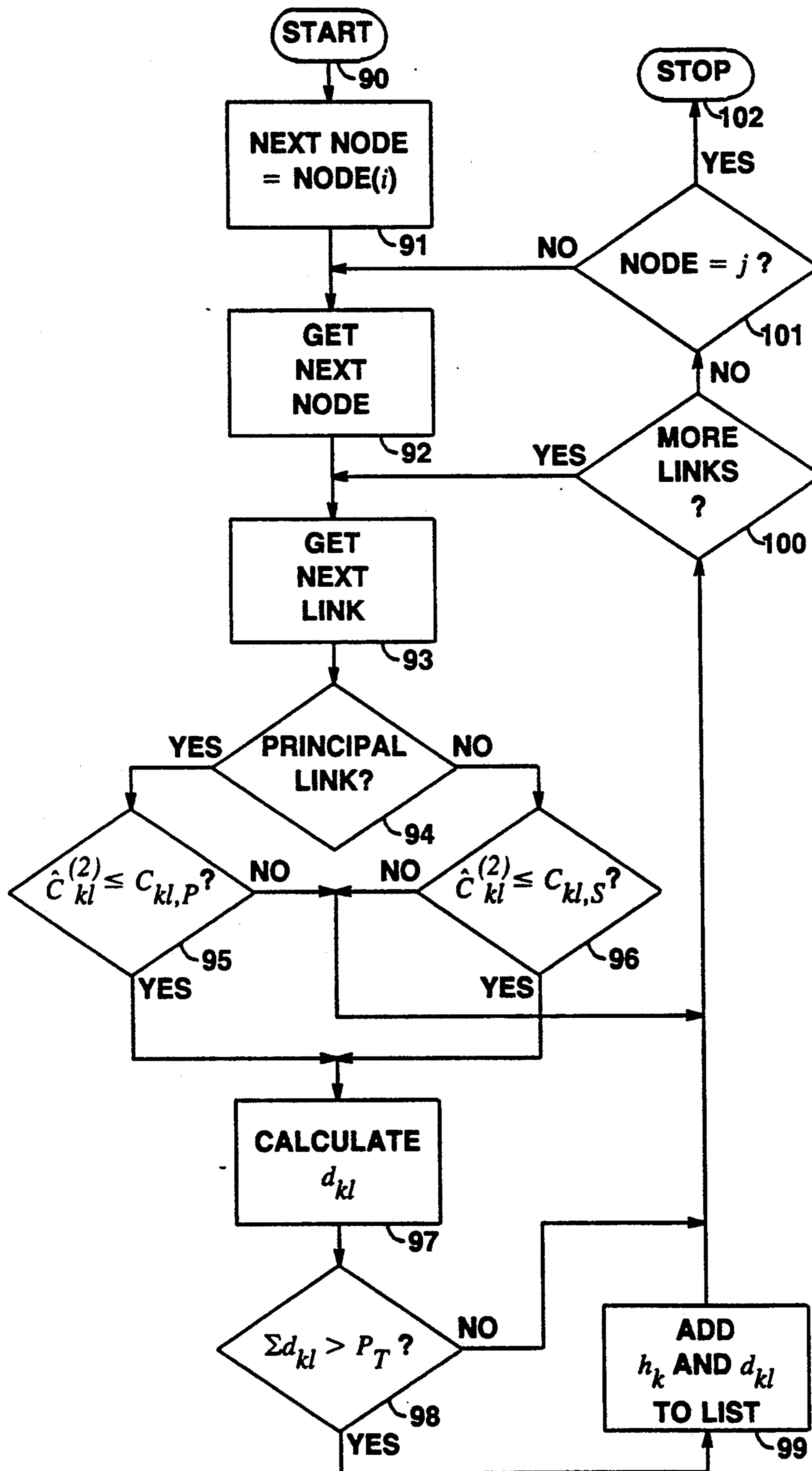
FIG. 10 SEARCH ALGORITHM
