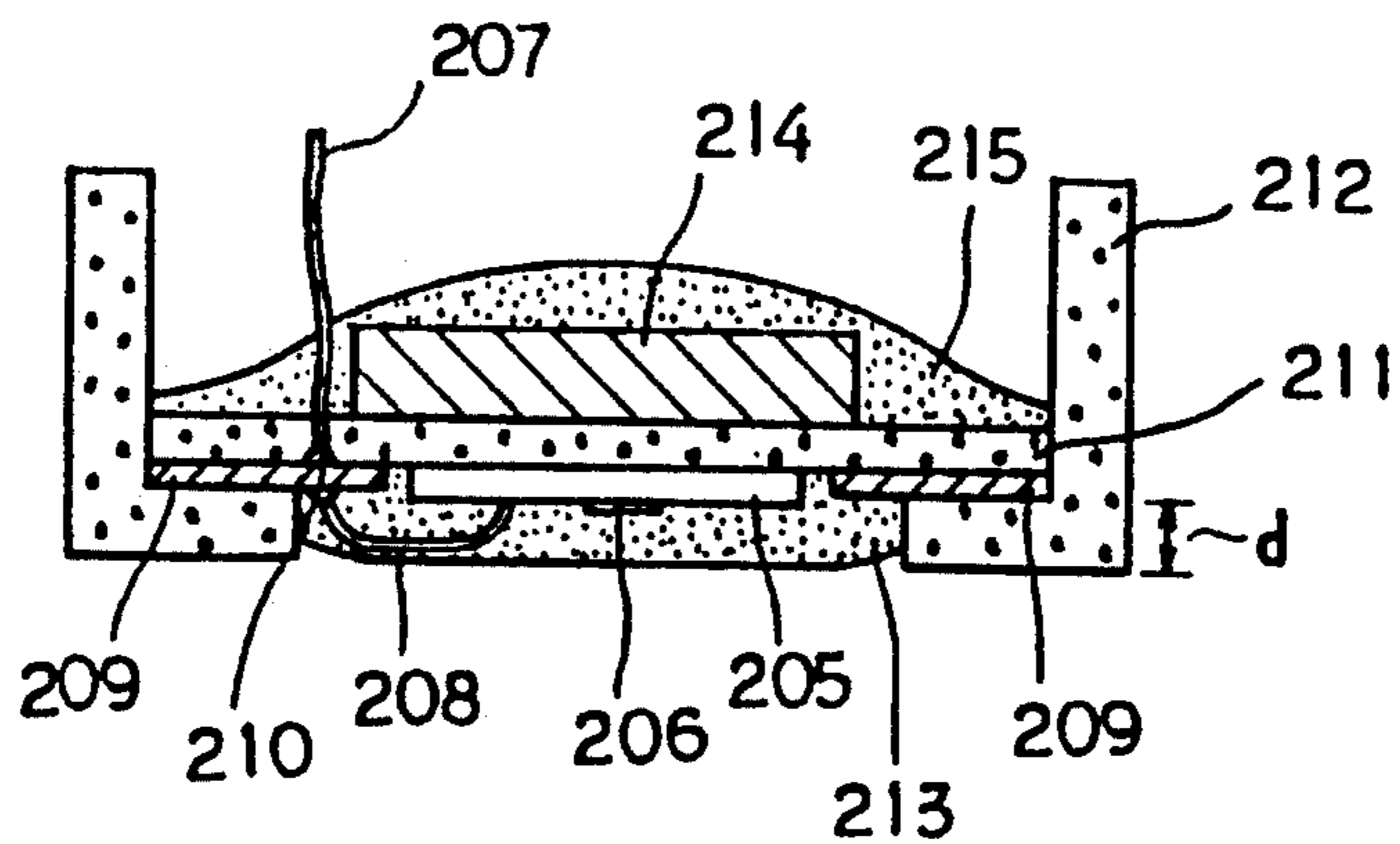
FIG. 2 (PRIOR ART)
