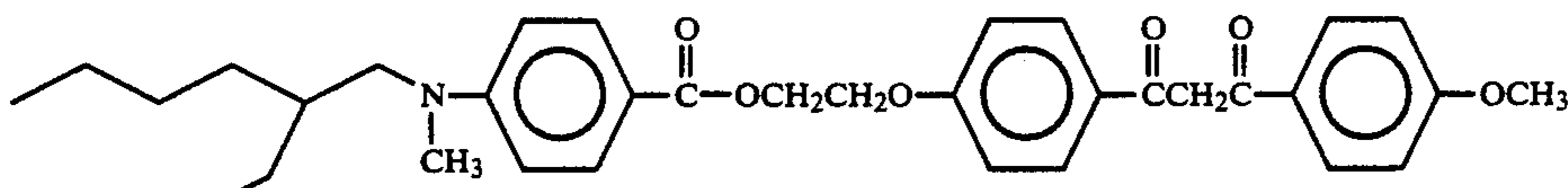
Compound 9
