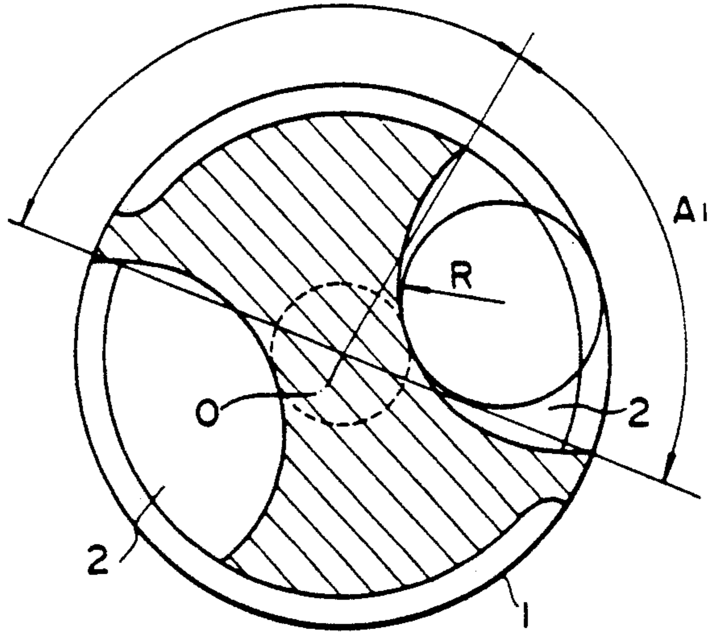
FIG. 4 (PRIOR ART)
