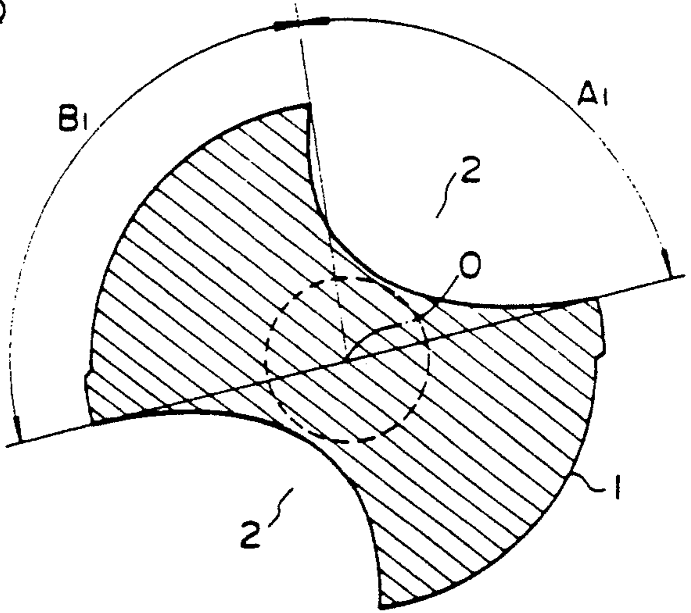
FIG. 4 (PRIOR ART)
