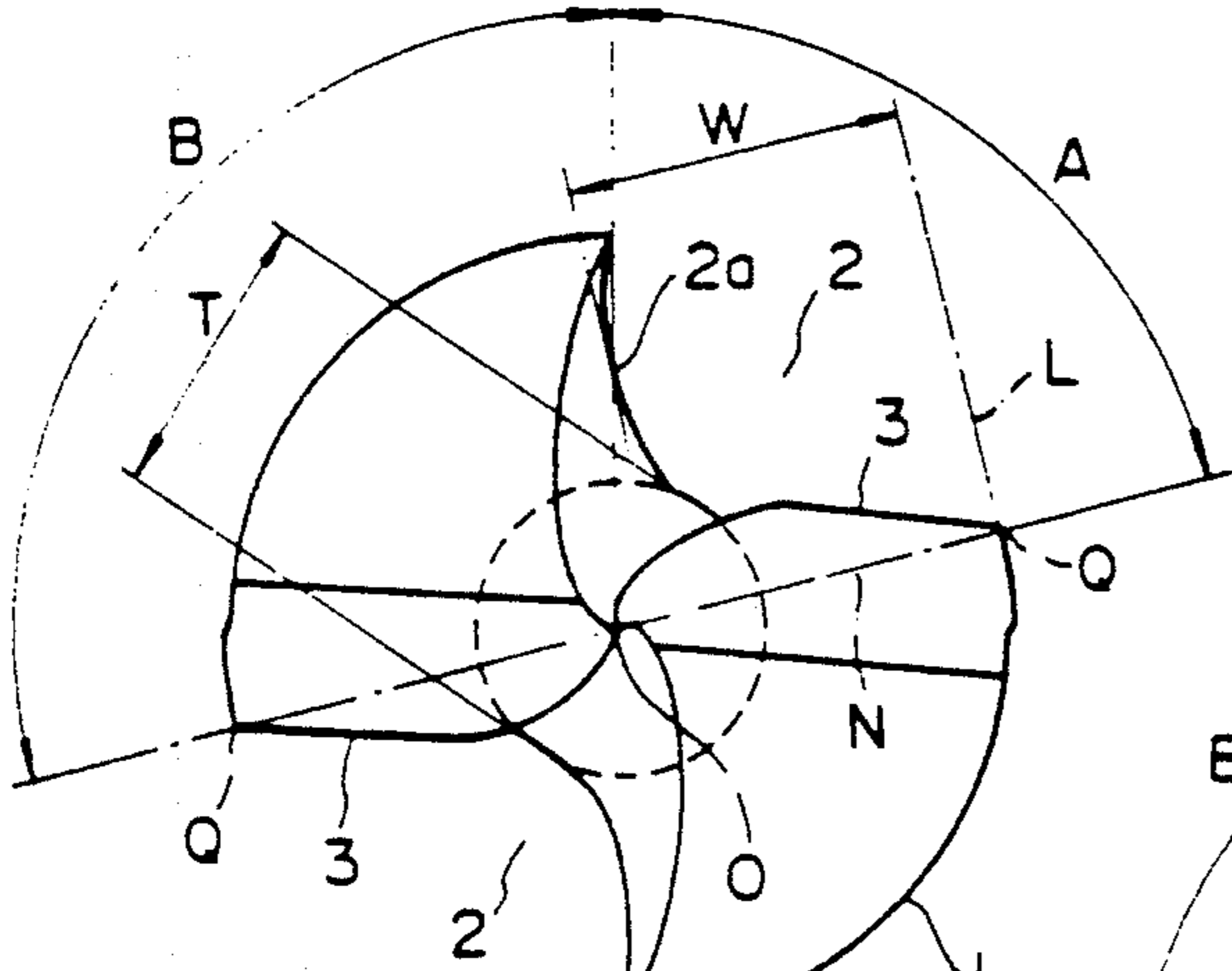
FIG. 3 (PRIOR ART)
