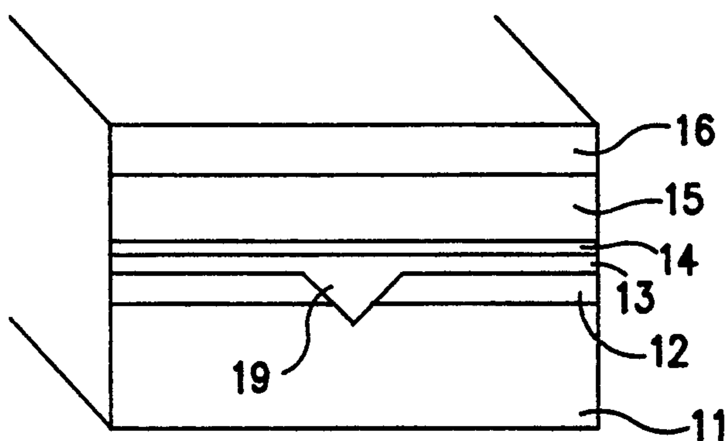
FIG. 30B PRIOR ART
