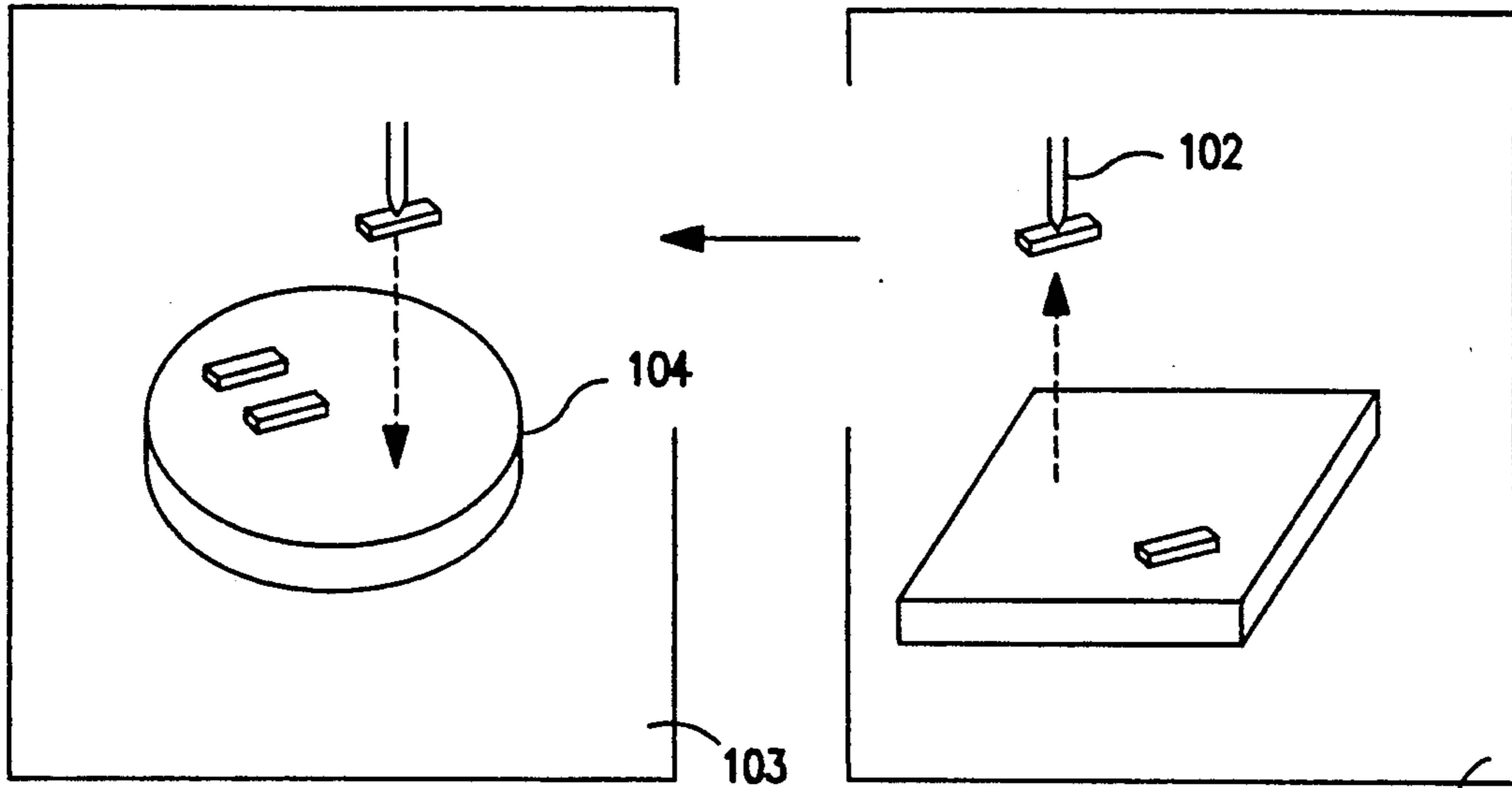
FIG. 30D PRIOR ART
