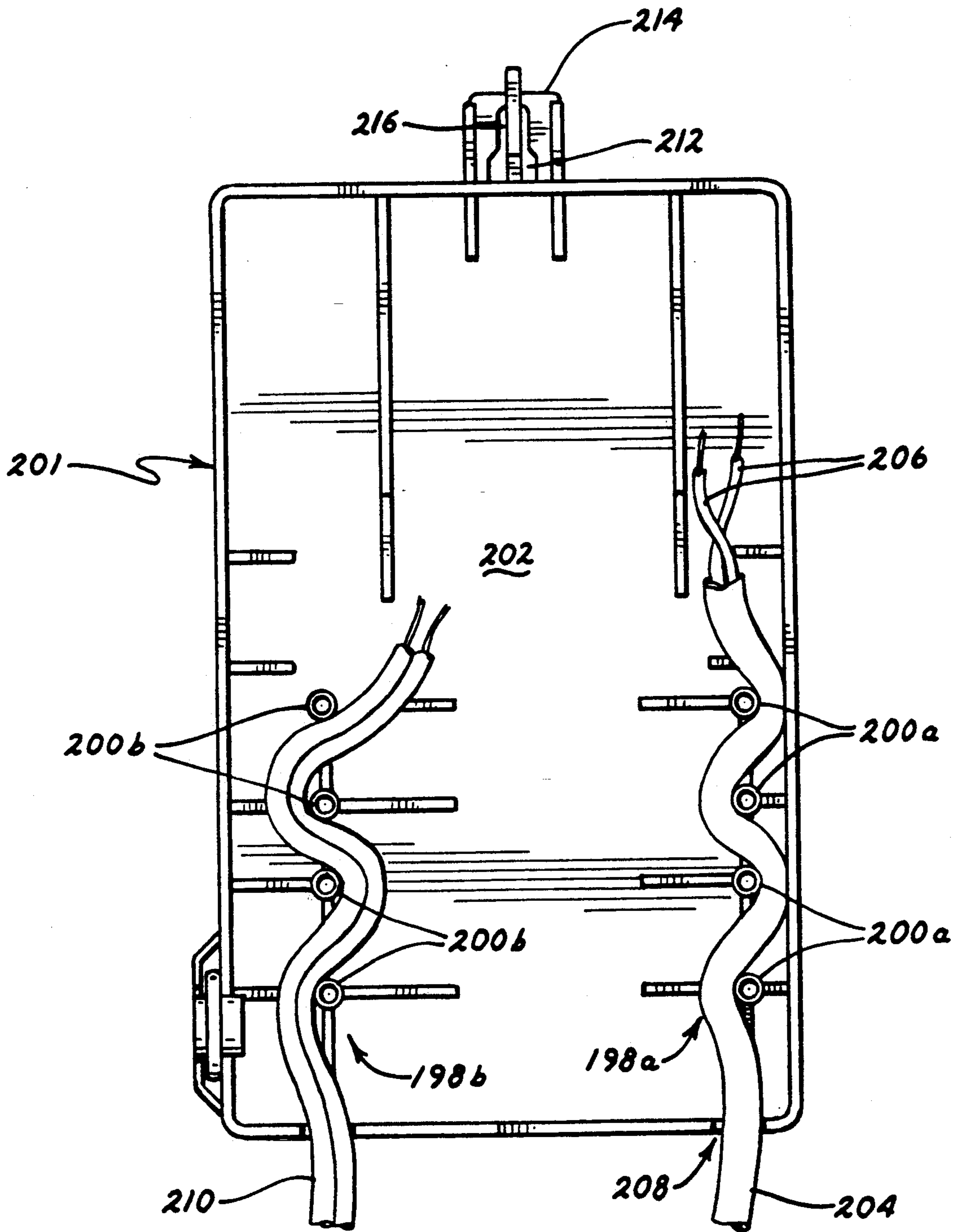
FIG. 9 PRIOR ART
