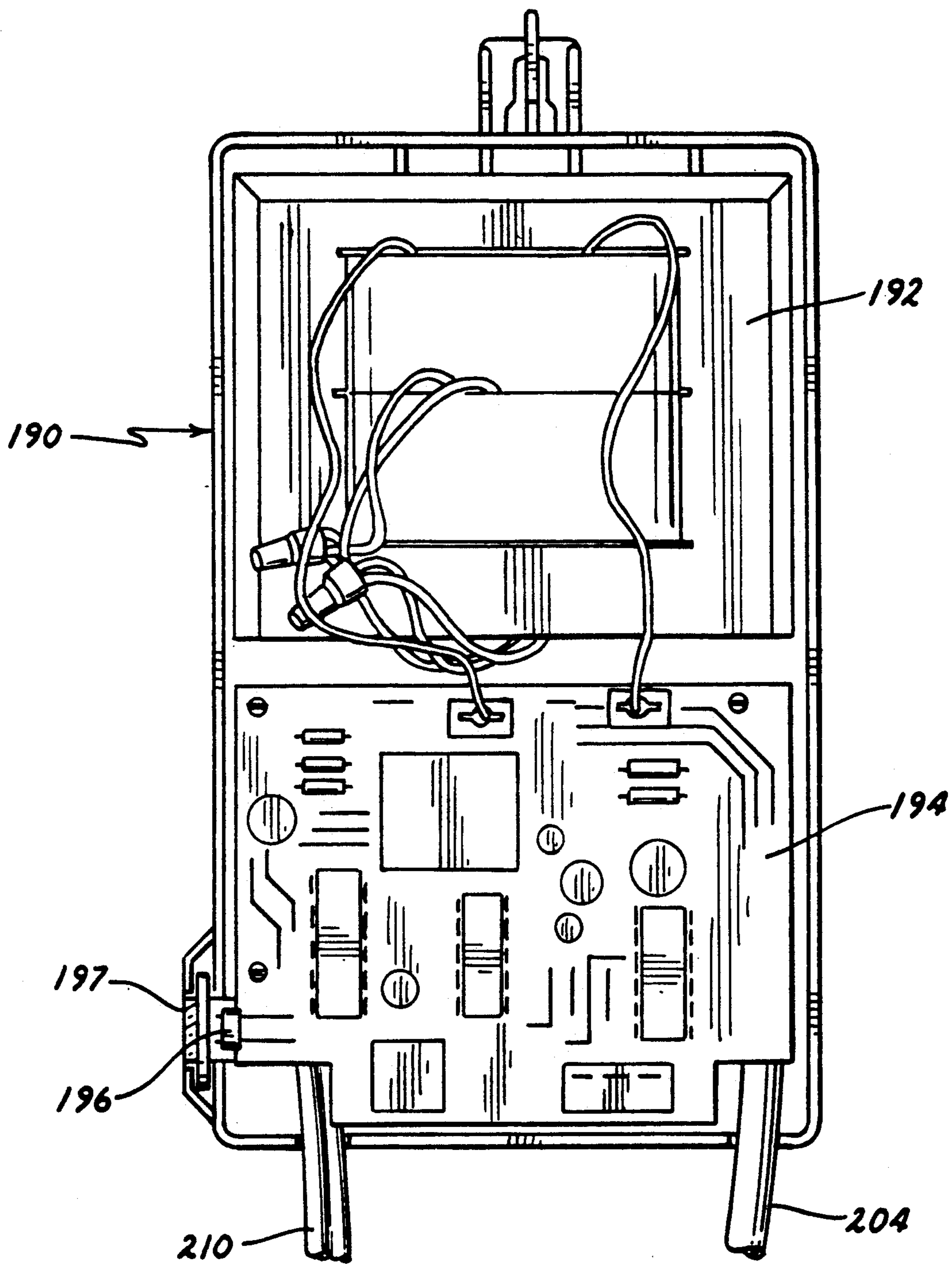
FIG. 10 PRIOR ART
