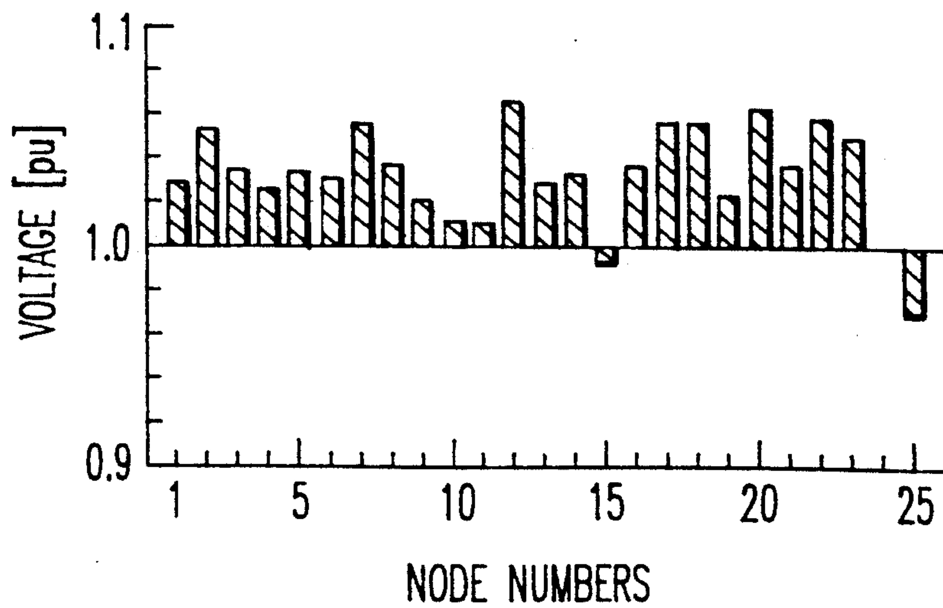
FIG. 14 PRIOR ART
