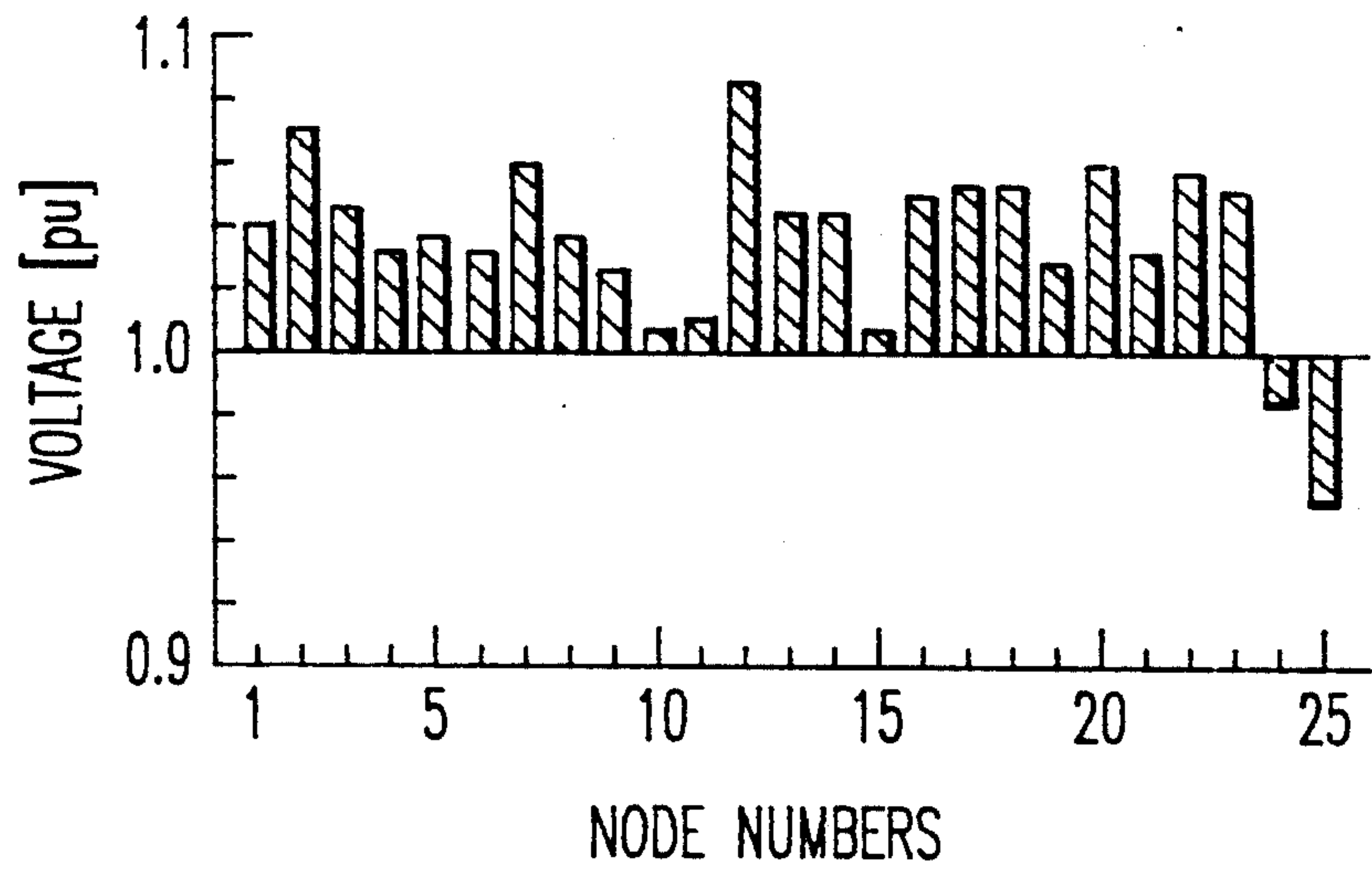
FIG. 12 PRIOR ART
