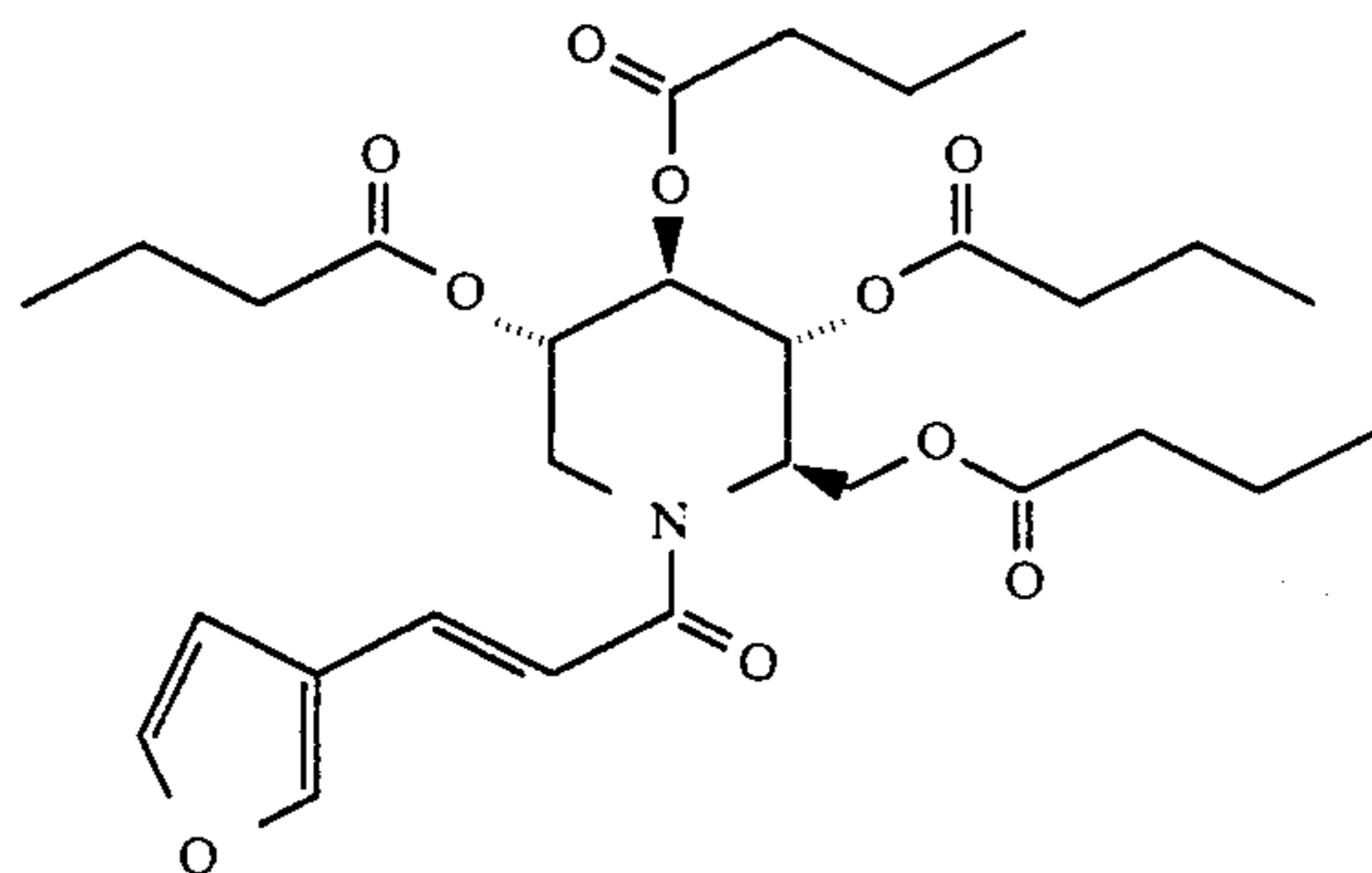
1,5-Dideoxy-1,5-[[3-(3-furanyl)-1-oxo-2E-propenyl]imino]-D-glucitol, tetrabutanoate
