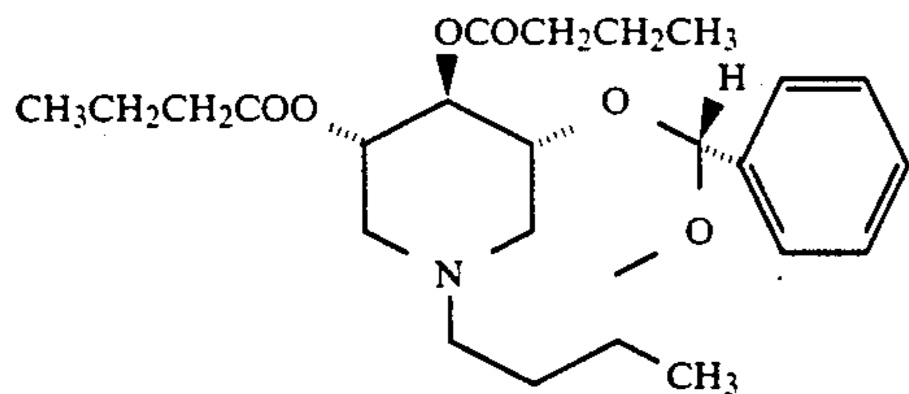
1,5-(Butylimino)-1,5-dideoxy-4R,6-O-(phenylmethylene)-D-glucitol, 2,3-dibutyrate
