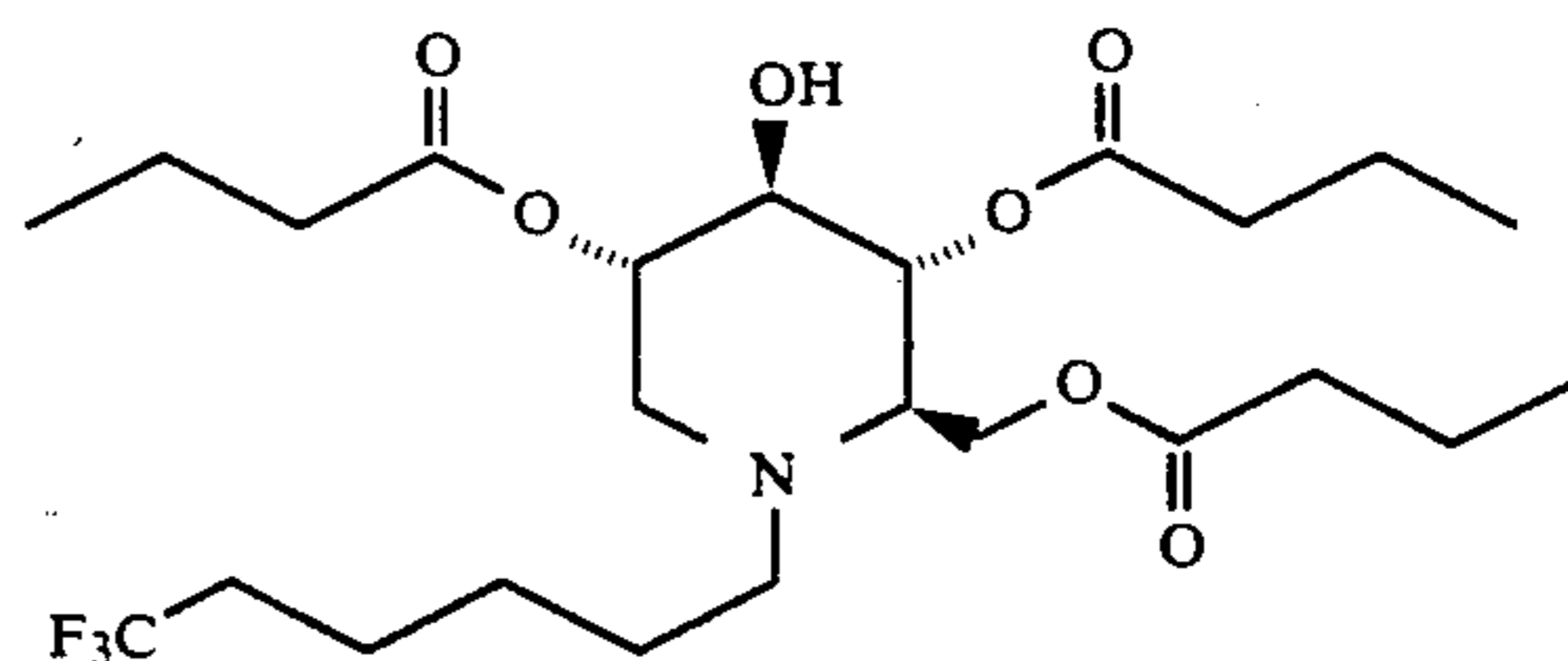
1,5-(6,6,6-Trifluorohexylimino)-1,5-dideoxy-D-glucitol, 2,4,6-tributyrates
