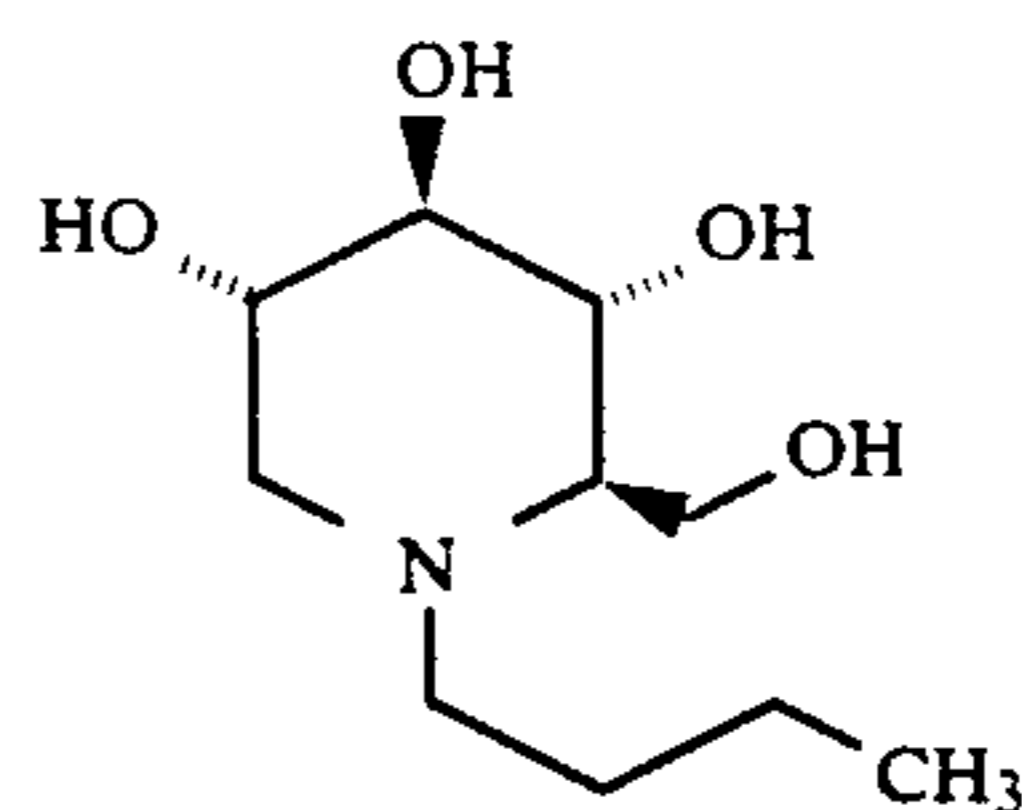
1,5-(Butylimino)-1,5-dideoxy-D-glucitol.
