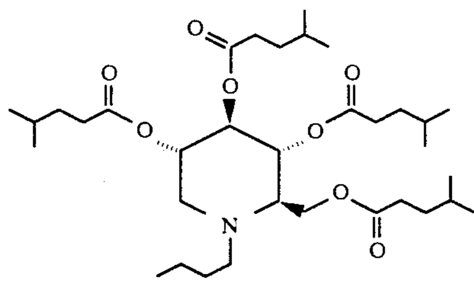
1,5-(Butylimino)-1,5-dideoxy-D-glucitol, tetra(4-methylpentanoate)
