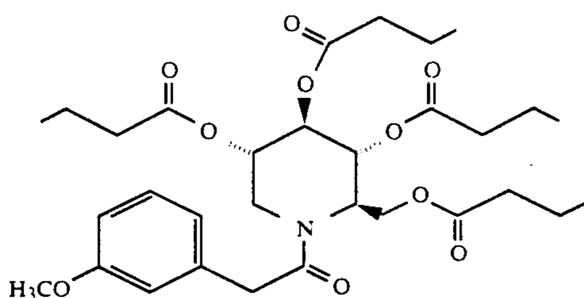
1,5-Dideoxy-1,5-[[2-(3-methoxyphenyl)-1-oxoethyl]-imino]-D-glucitol, tetrabutanoate
