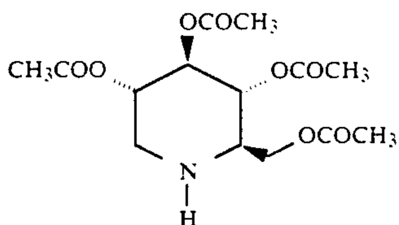
1,5-Dideoxy-1,5-imino-D-glucitol, tetraacetate.
