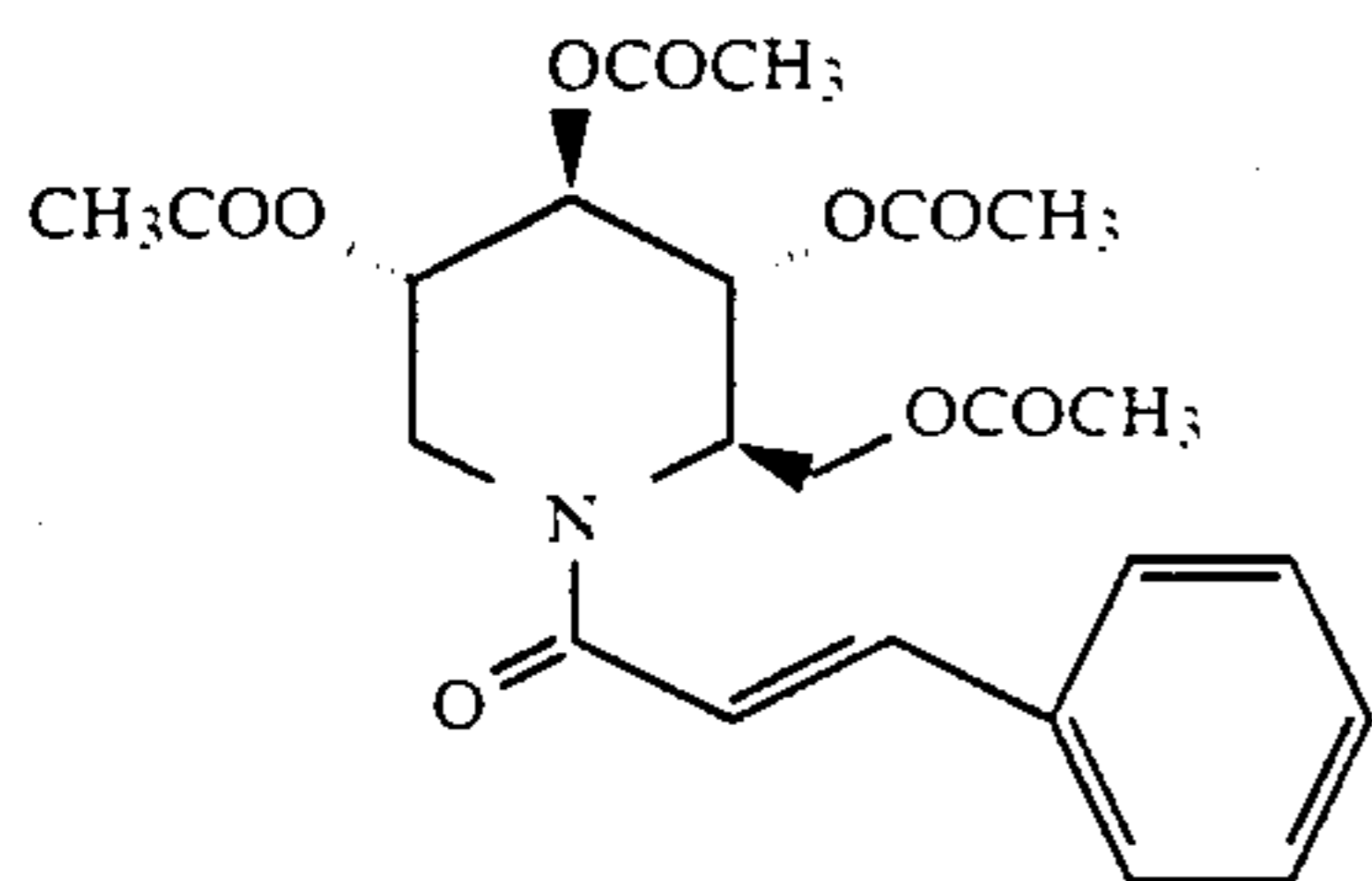
1,5-(Cinnamoylimino)-1,5-dideoxy-D-glucitol, tetraacetate
