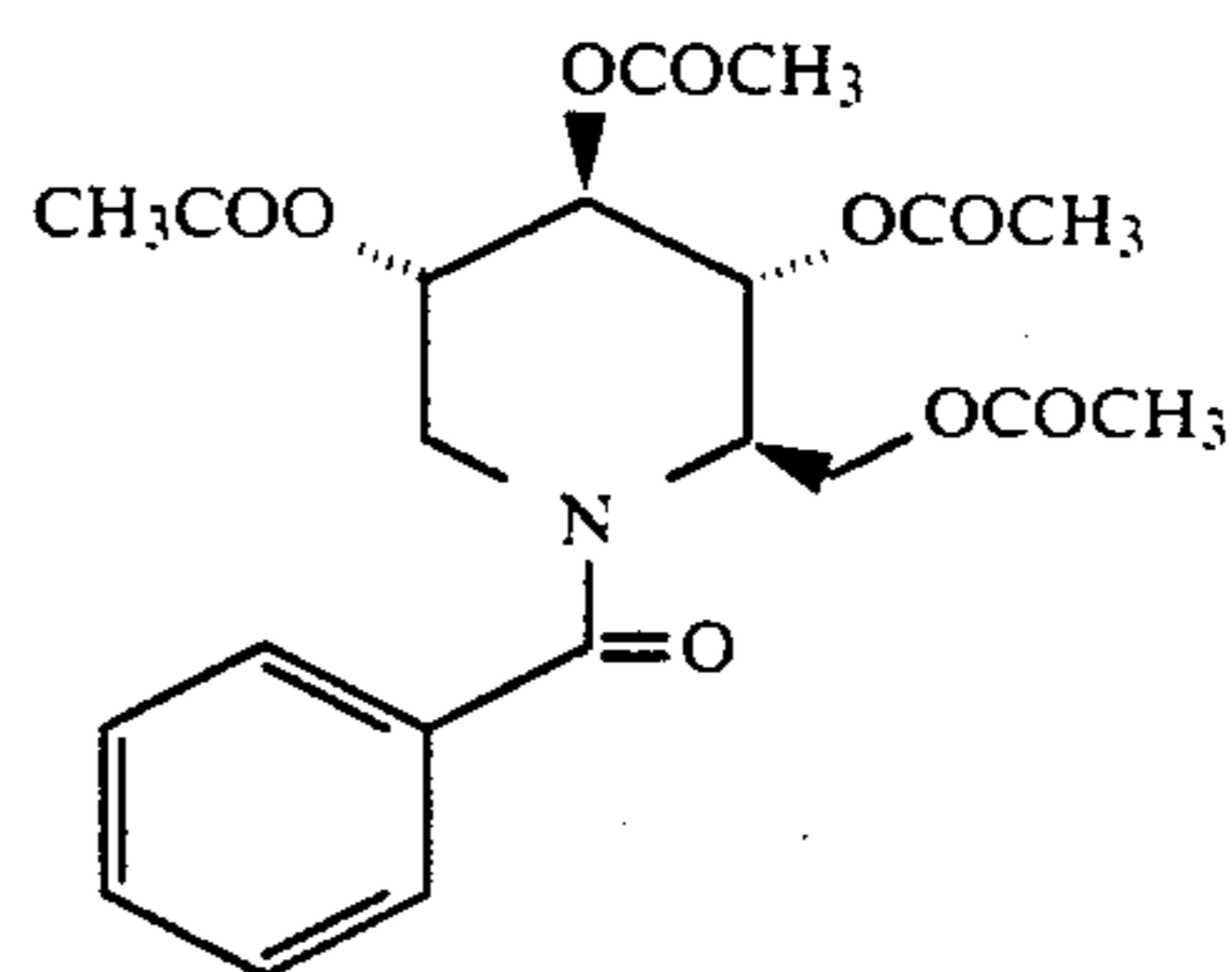
1,5-(Benzoylimino)-1,5-dideoxy-D-glucitol, tetraacetate.
