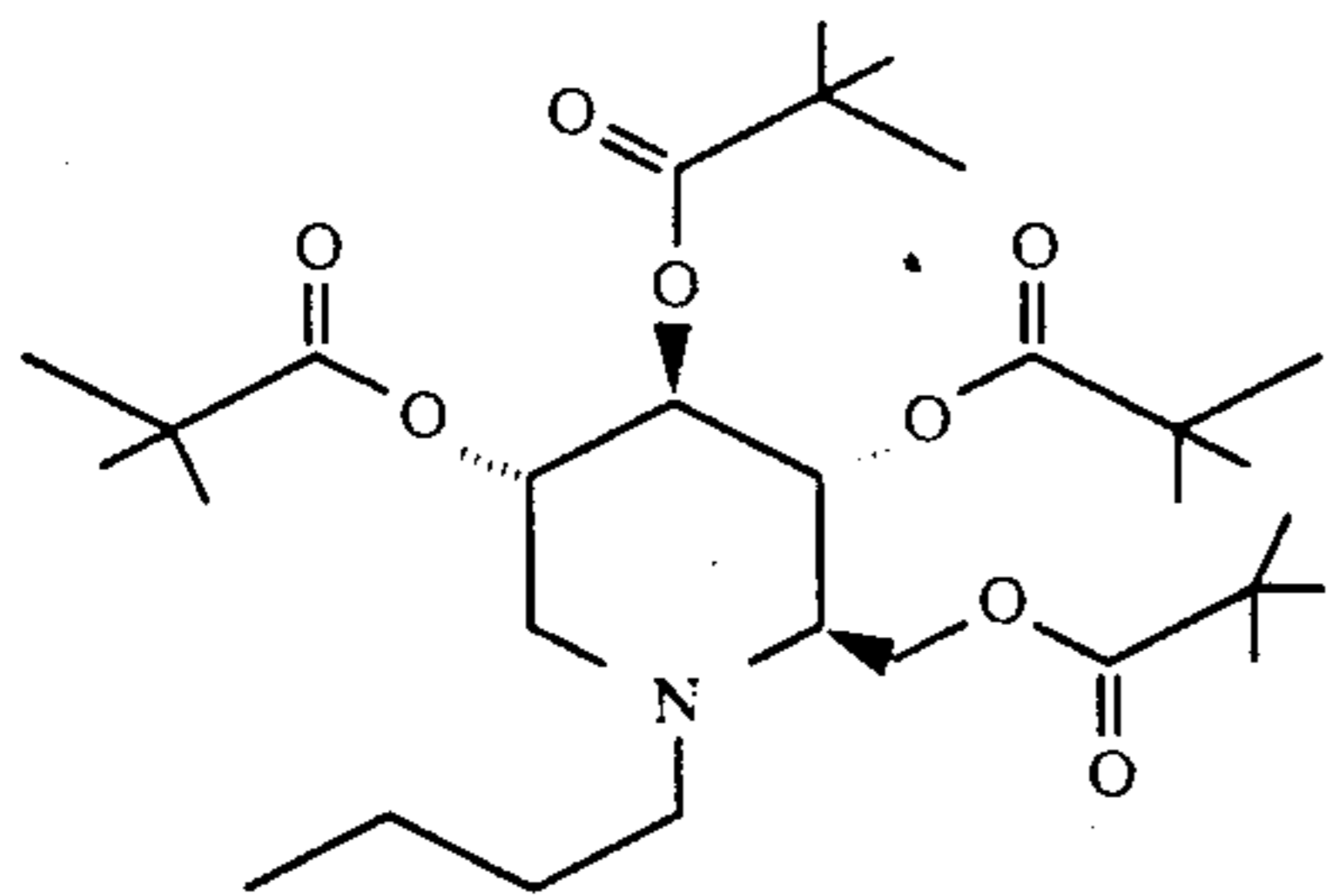
1,5-(Butylimino)-1,5-dideoxy-D-glucitol, tetra(2,2-dimethylpropanoate)
