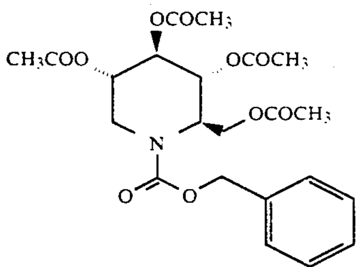
1,5-(Benzyloxycarbonylimino)-1,5-dideoxy-D-glucitol, tetraacetate.
