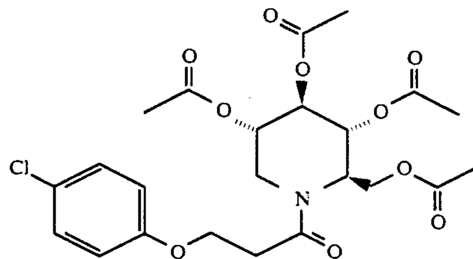
1,5-Dideoxy-1,5-[[3-(4-chlorophenoxy)-1-oxopropyl]- imino]-D-glucitol, tetraacetate
