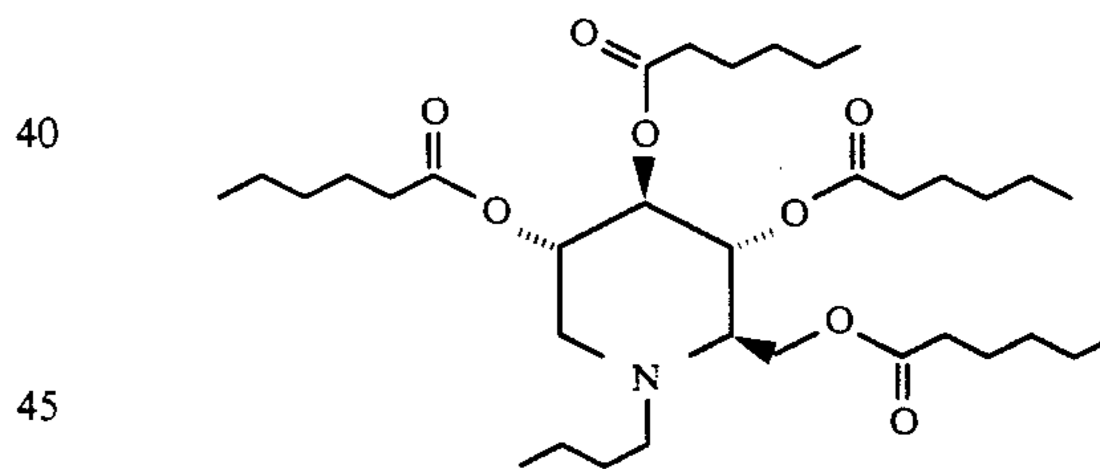
1,5-(Butylimino)-1,5-dideoxy-D-glucitol, tetrahexanoate
