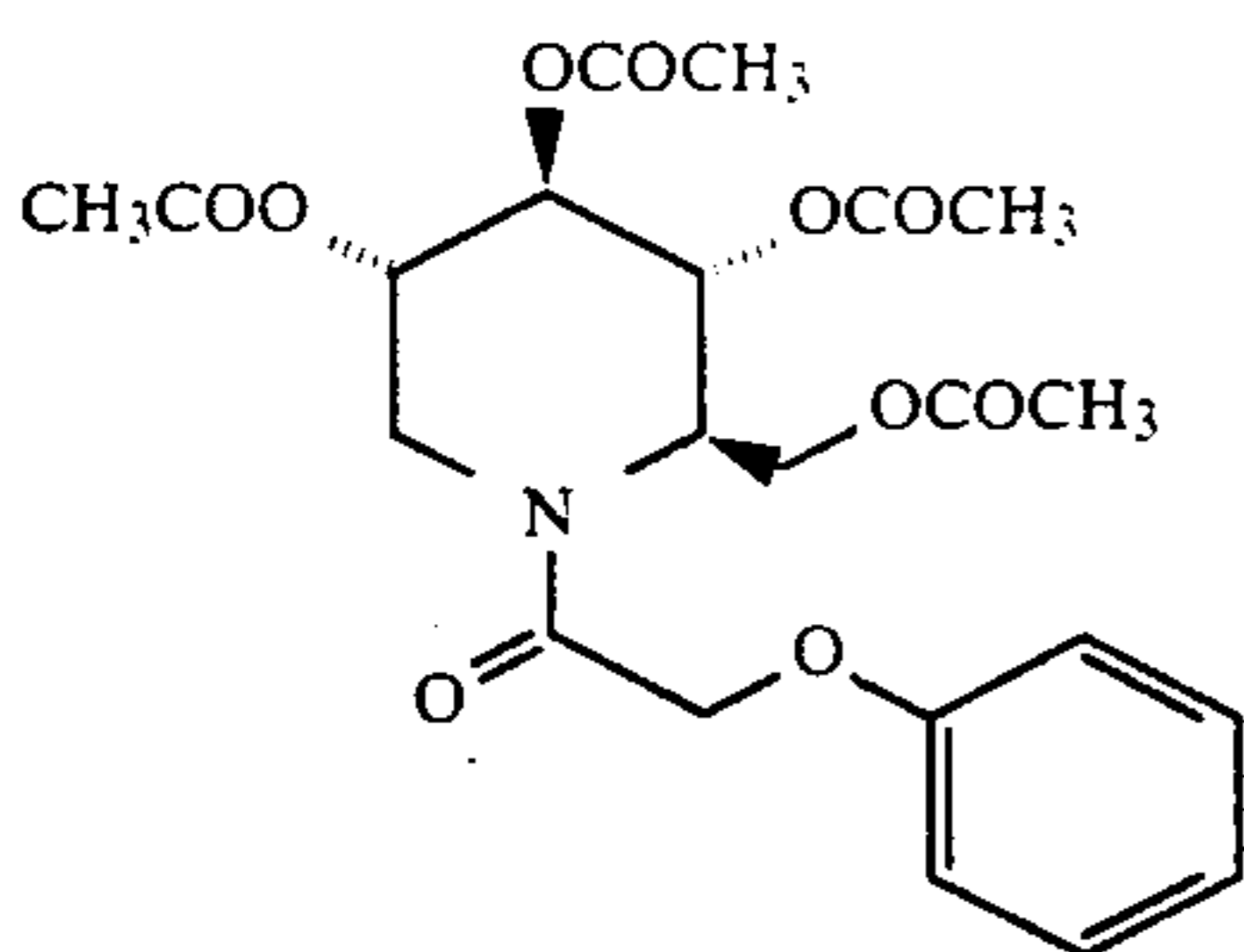
1,5-[(Phenoxymethyl)carbonylimino]-1,5-dideoxy-D-glucitol, tetraacetate
