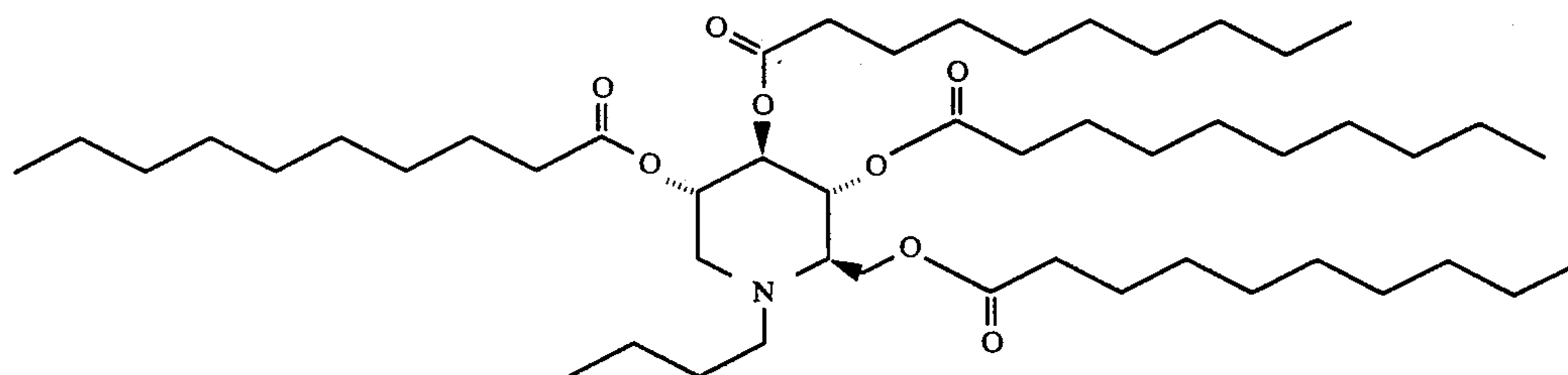
1,5-(Butylimino)-1,5-dideoxy-D-glucitol, tetradecanoate
