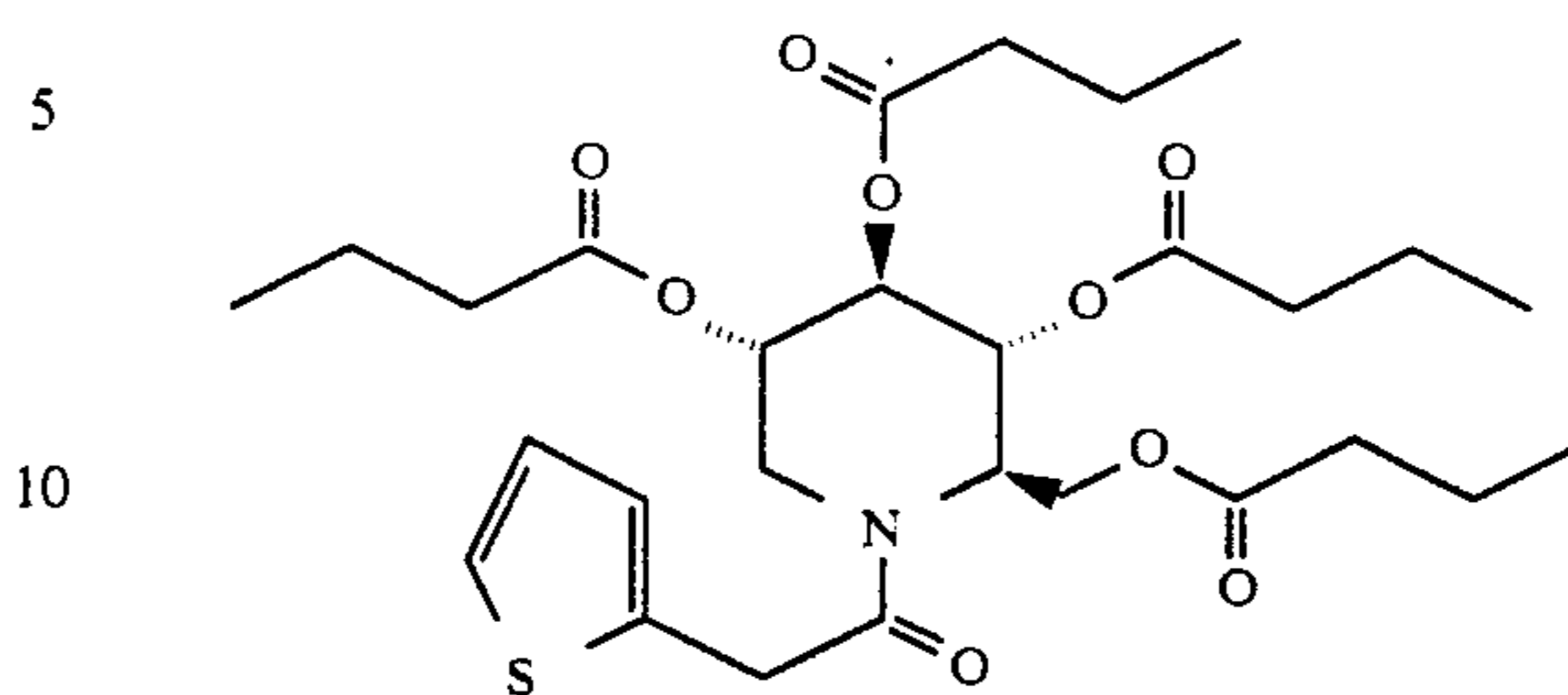
1,5-Dideoxy-1,5-[[1-oxo-2-(2-thienyl)ethyl]imino]-D-glucitol, tetrabutanoate
