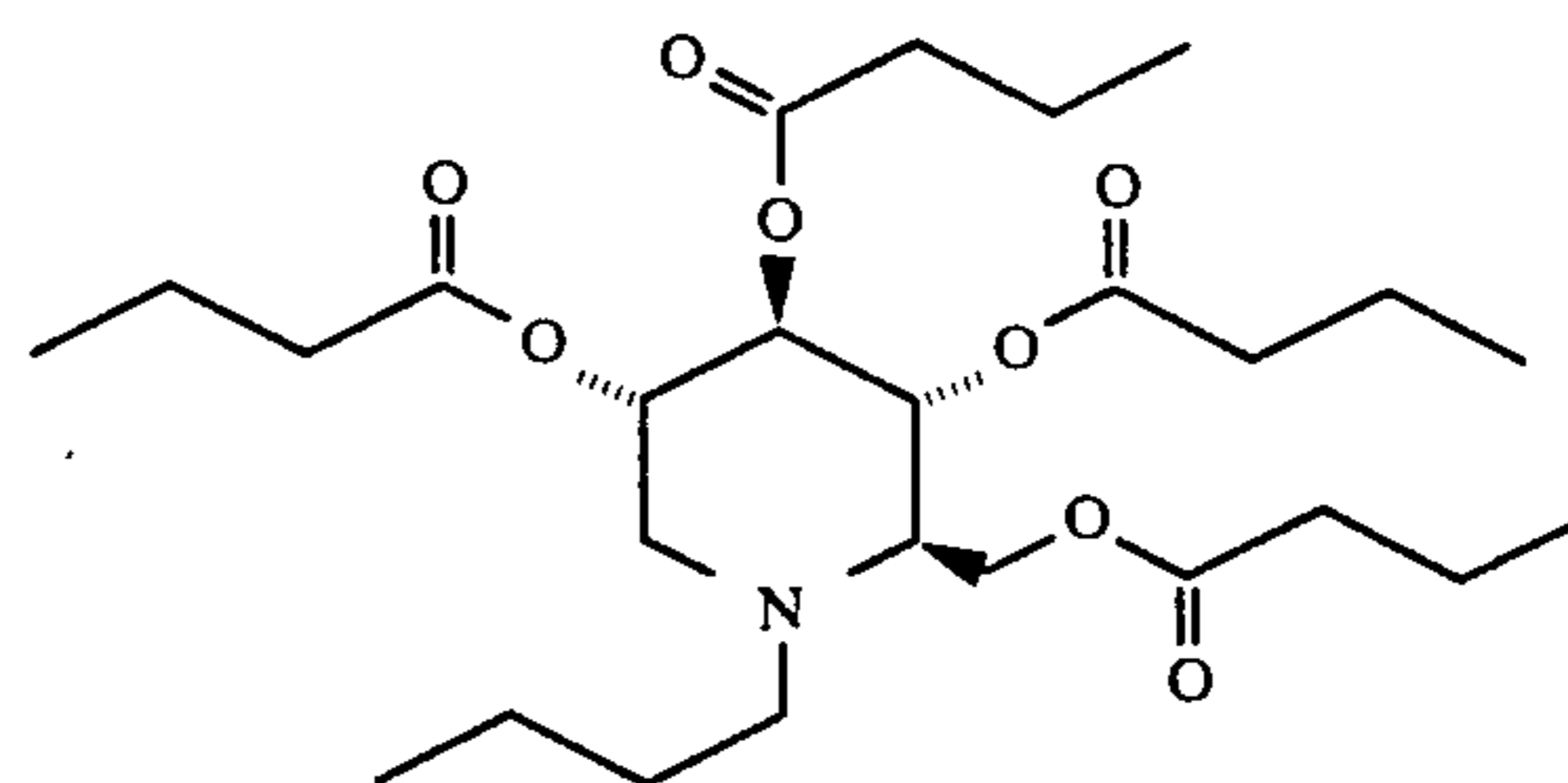
1,5-(Butylimino)-1,5-dideoxy-D-glucitol, tetrabutyrate
