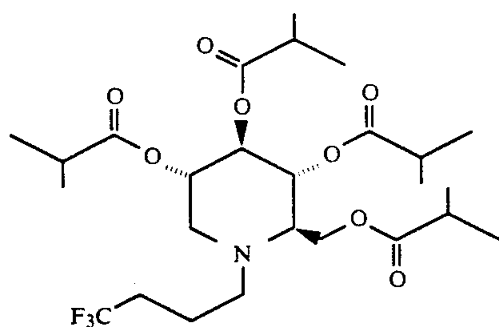
1,5-(4,4,4-Trifluorobutylimino)-1,5-dideoxy-D-glucitol, tetraisobutyrate
