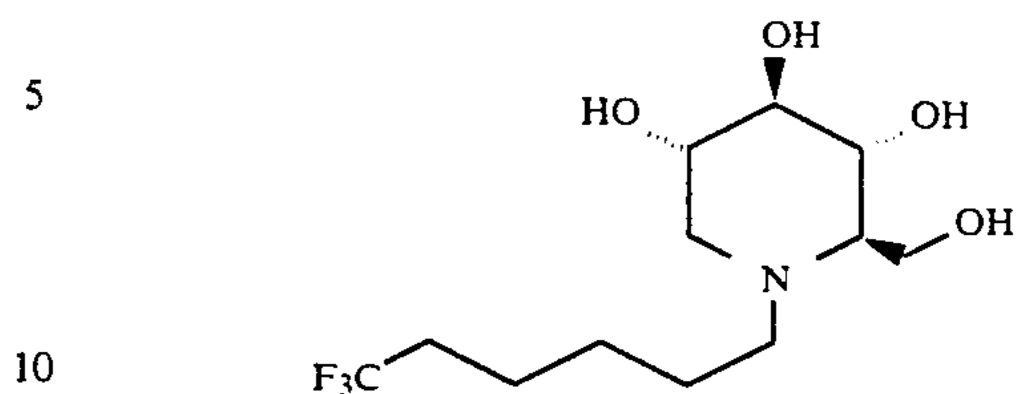
1,5-(6,6,6-Trifluorohexylimino)-1,5-dideoxy-D-glucitol
