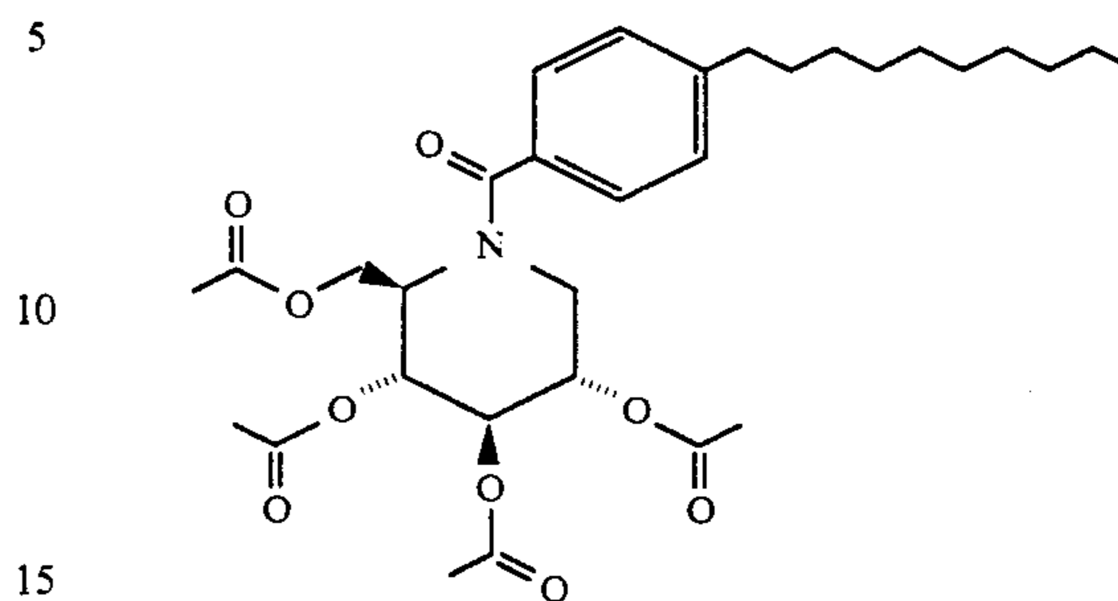
1,5-[(4-Decylbenzoyl)imino]-1,5-dideoxy-D-glucitol, tetraacetate
