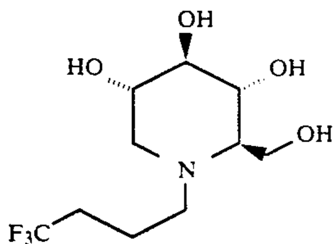
1,5-(4,4,4-Trifluorobutylimino)-1,5-dideoxy-D-glucitol
