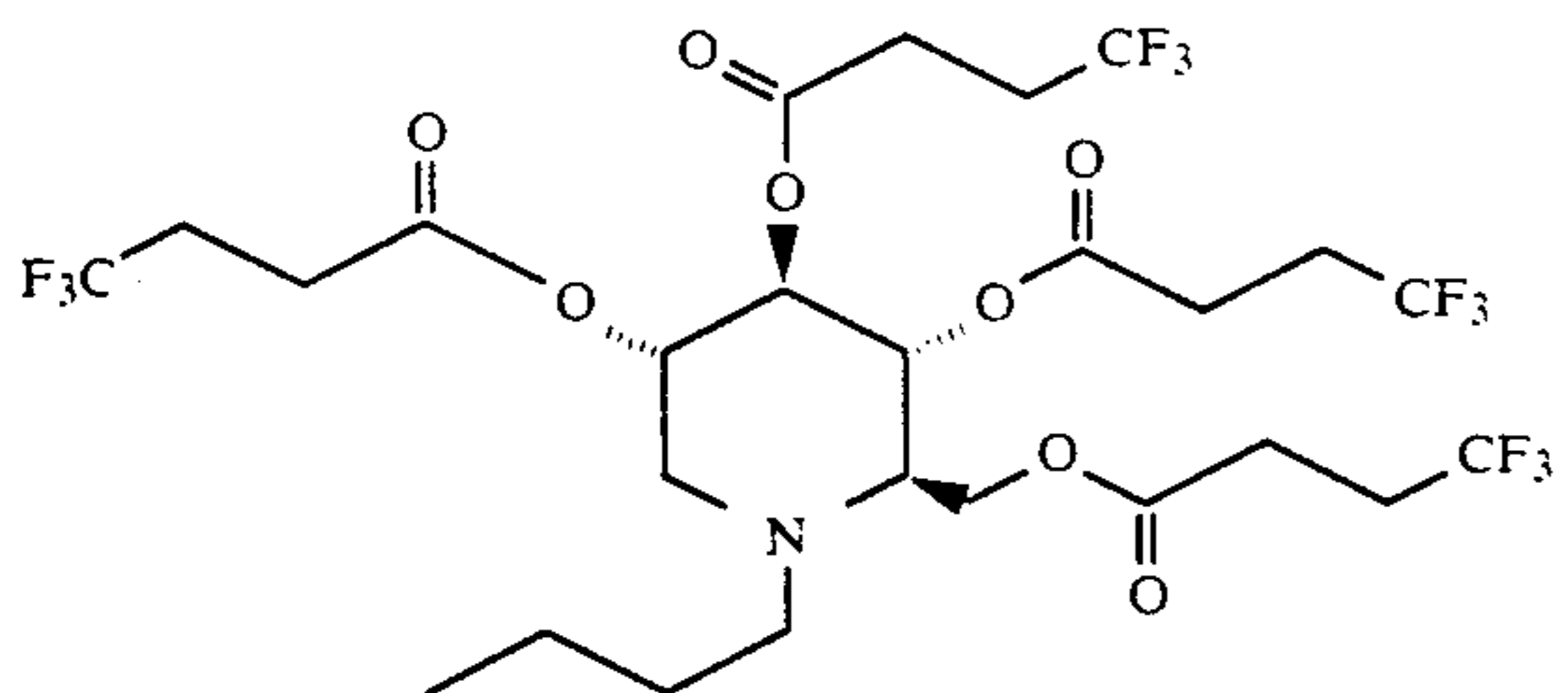
1,5-(Butylimino)-1,5-dideoxy-D-glucitol, tetra(4,4,4-trifluorobutanoate)
