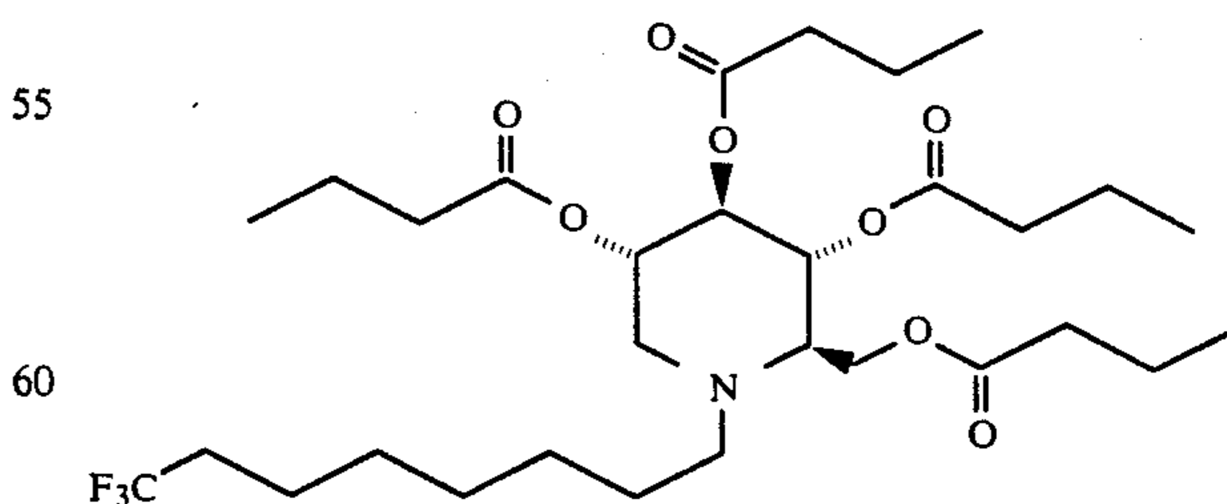
1,5-(8,8,8-Trifluorooctylimino)-1,5-dideoxy-D-glucitol, tetrabutrate
