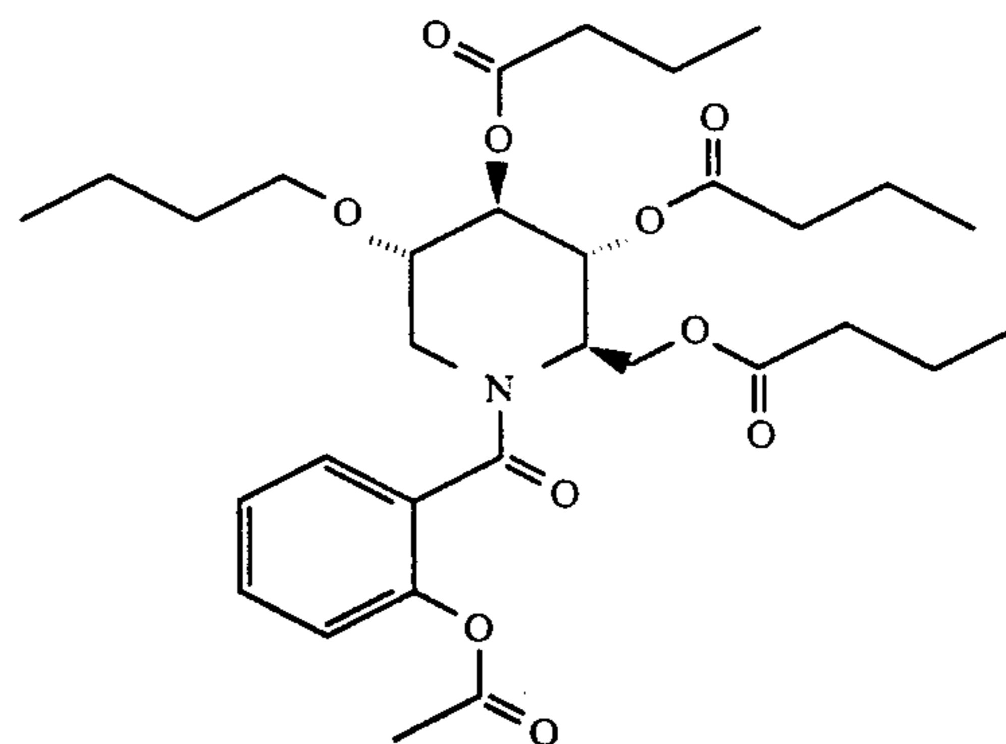
1,5-[[2-Acetyloxy]benzoyl]imino]-1,5-dideoxy-D- glucitol, tetrabutanoate
