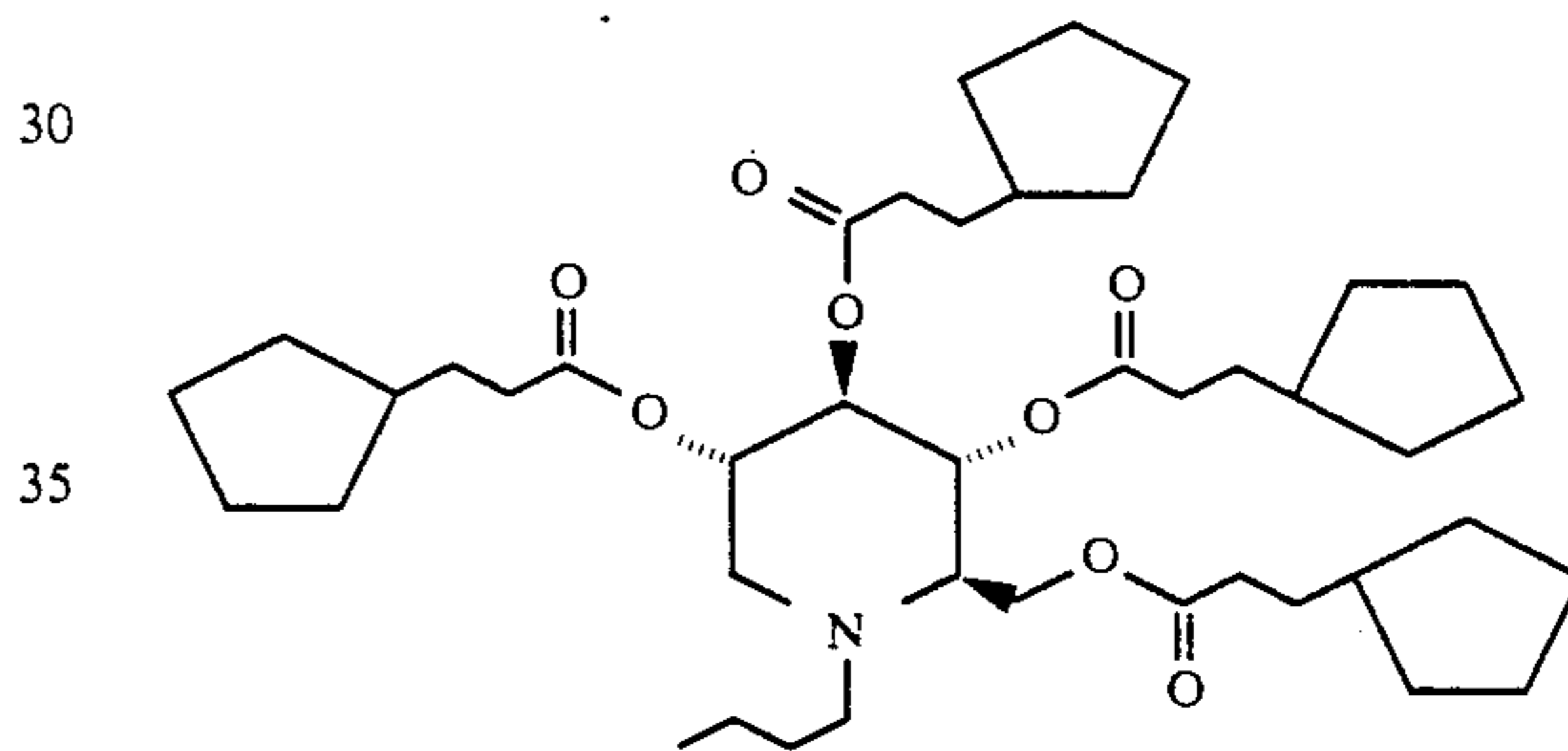
1,5-(Butylimino)-1,5-dideoxy-D-glucitol, tetra(3-cyclopentylpropanoate)
