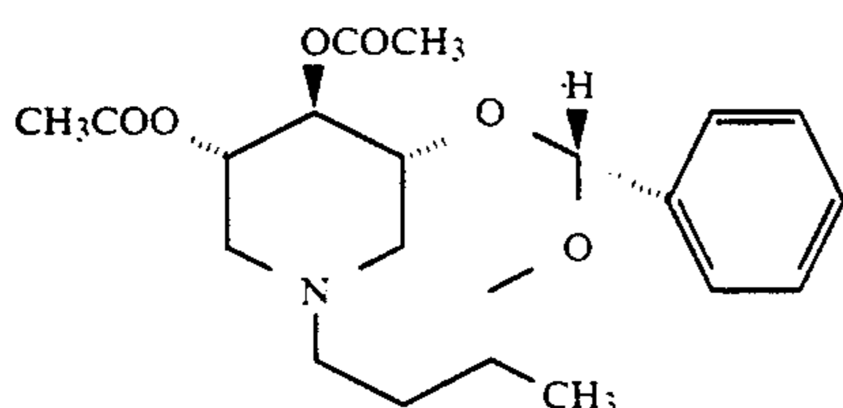
1,5-(Butylimino)-1,5-dideoxy-4R,6-O-(phenylmethyl)-D-glucitol, diacetate
