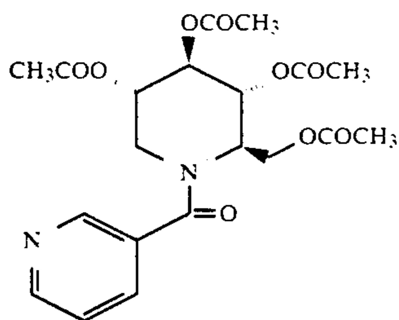
1,5-[(3-Nicotinoyl)imino]-1,5-dideoxy-D-glucitol, tetraacetate
