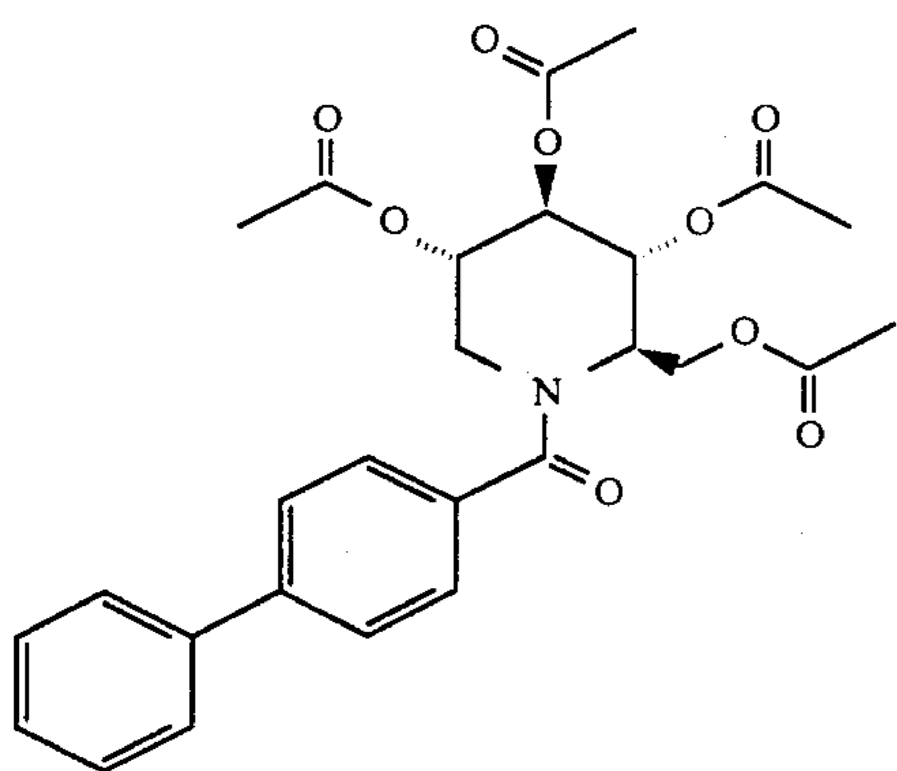
1,5-[[[1,1'-biphenyl]-4-ylcarbonyl]imino]-1,5-dideoxy-D-glucitol, tetraacetate
