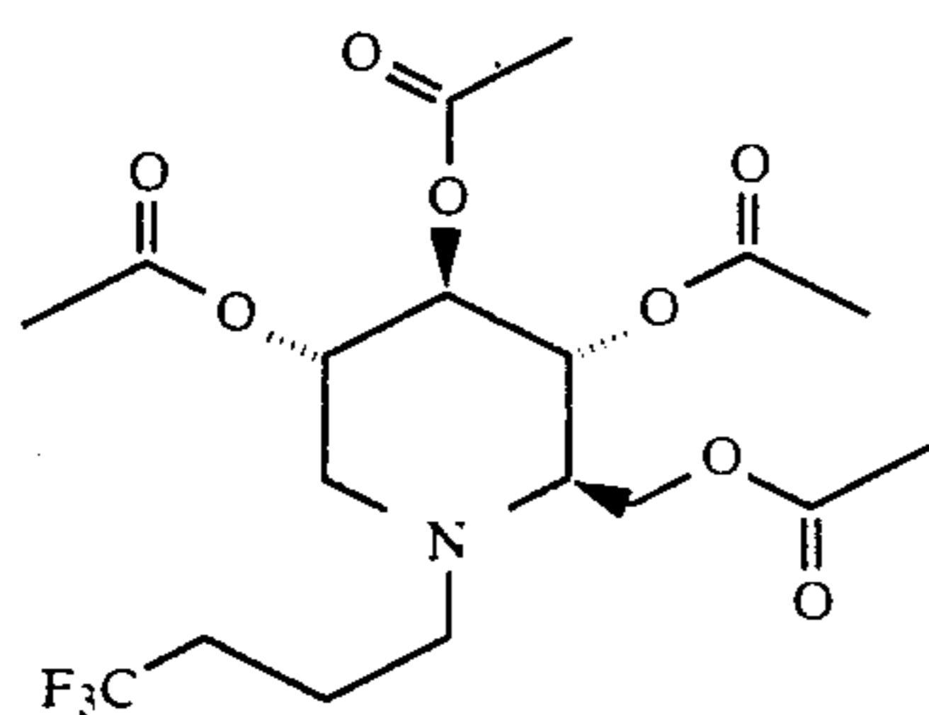
1,5-(4,4,4-Trifluorobutylimino)-1,5-dideoxy-D-glucitol, tetraacetate
