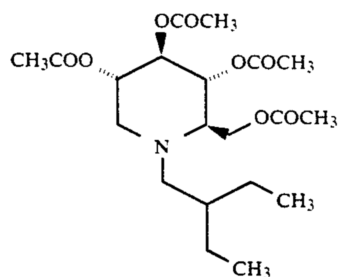
1,5-[(2-Ethylbutyl)imino]-1,5-dideoxy-D-glucitol, tetraacetate
