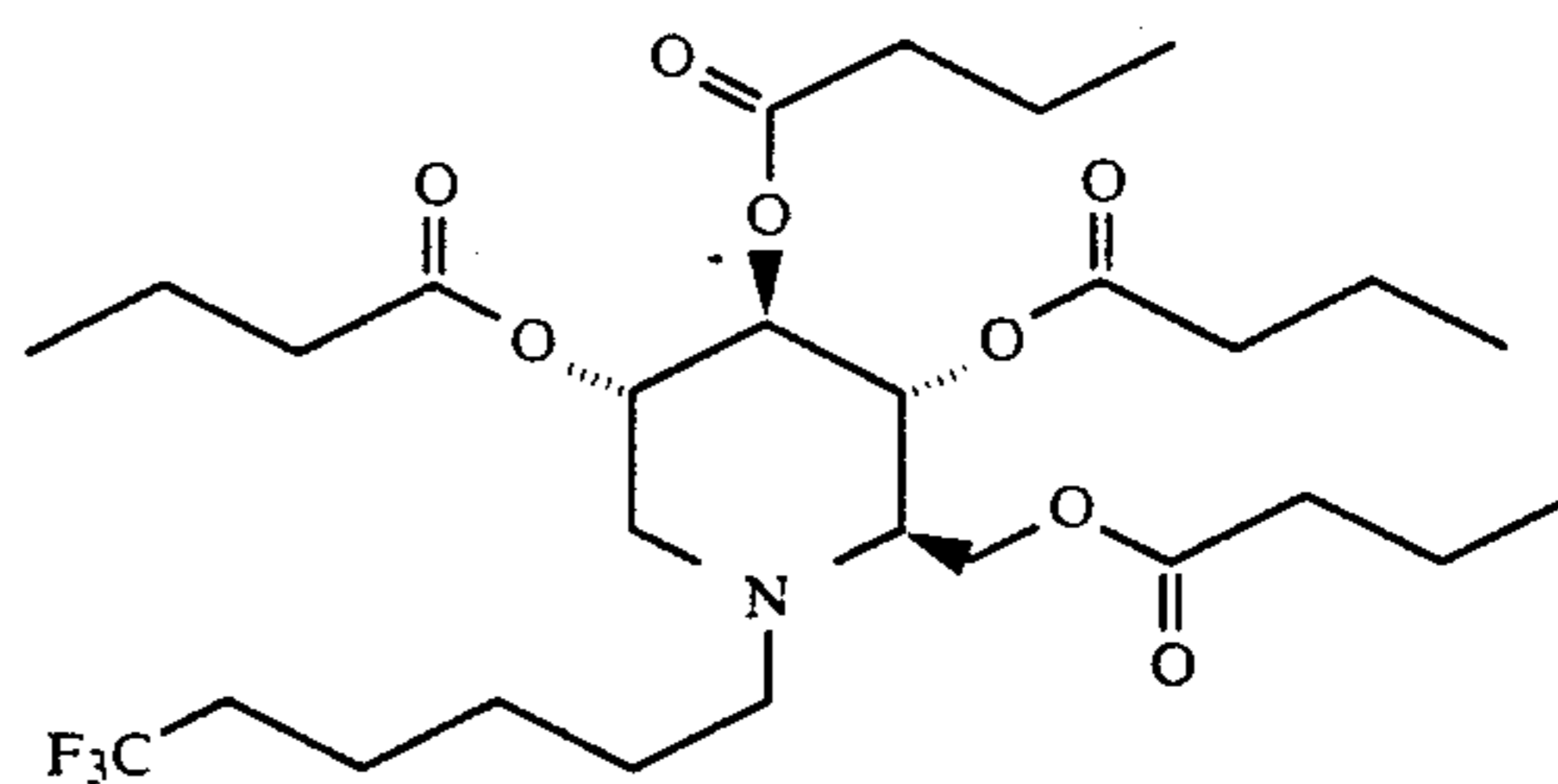
1,5-(6,6,6-Trifluorohexylimino)-1,5-dideoxy-D-glucitol, tetrabutyrates
