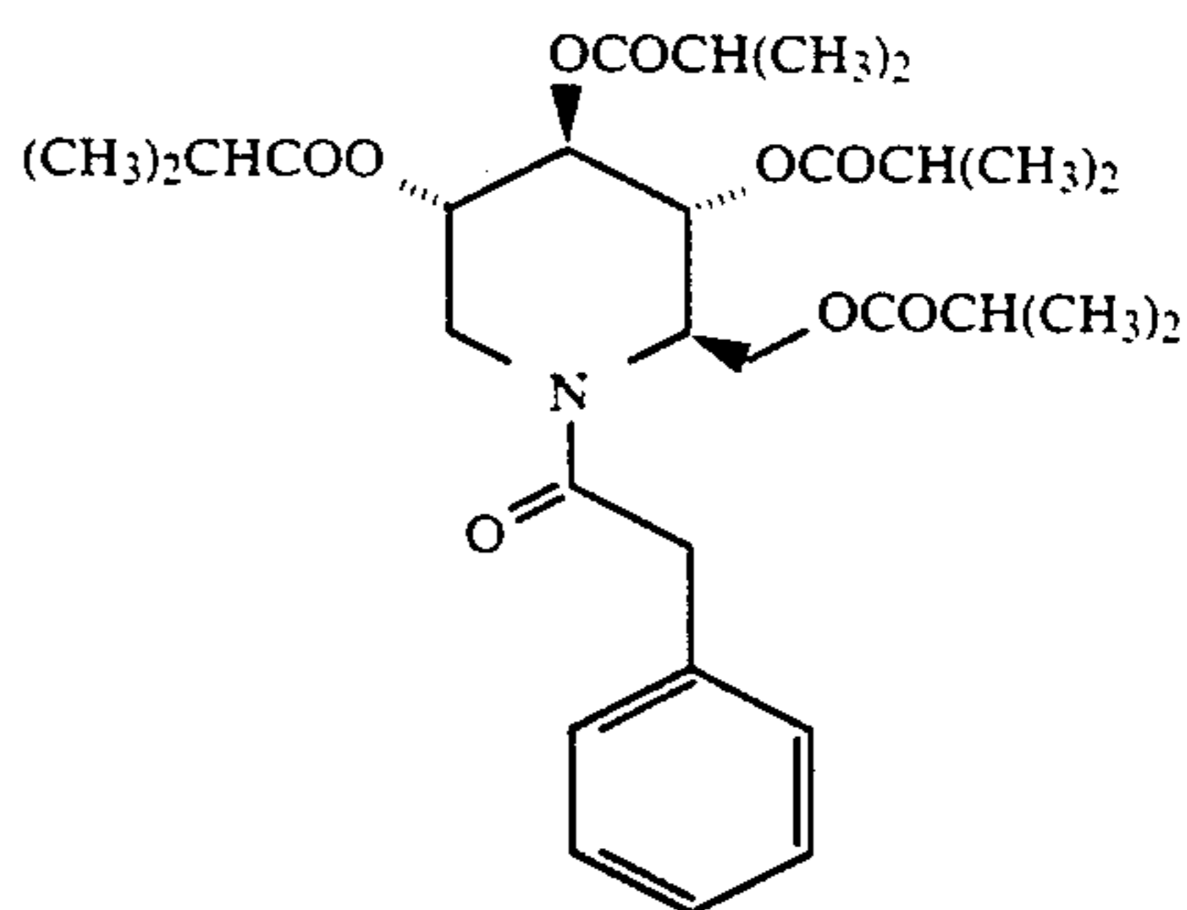
1,5-(Phenylacetylimino)-1,5-dideoxy-D-glucitol, tetraisobutyrate
