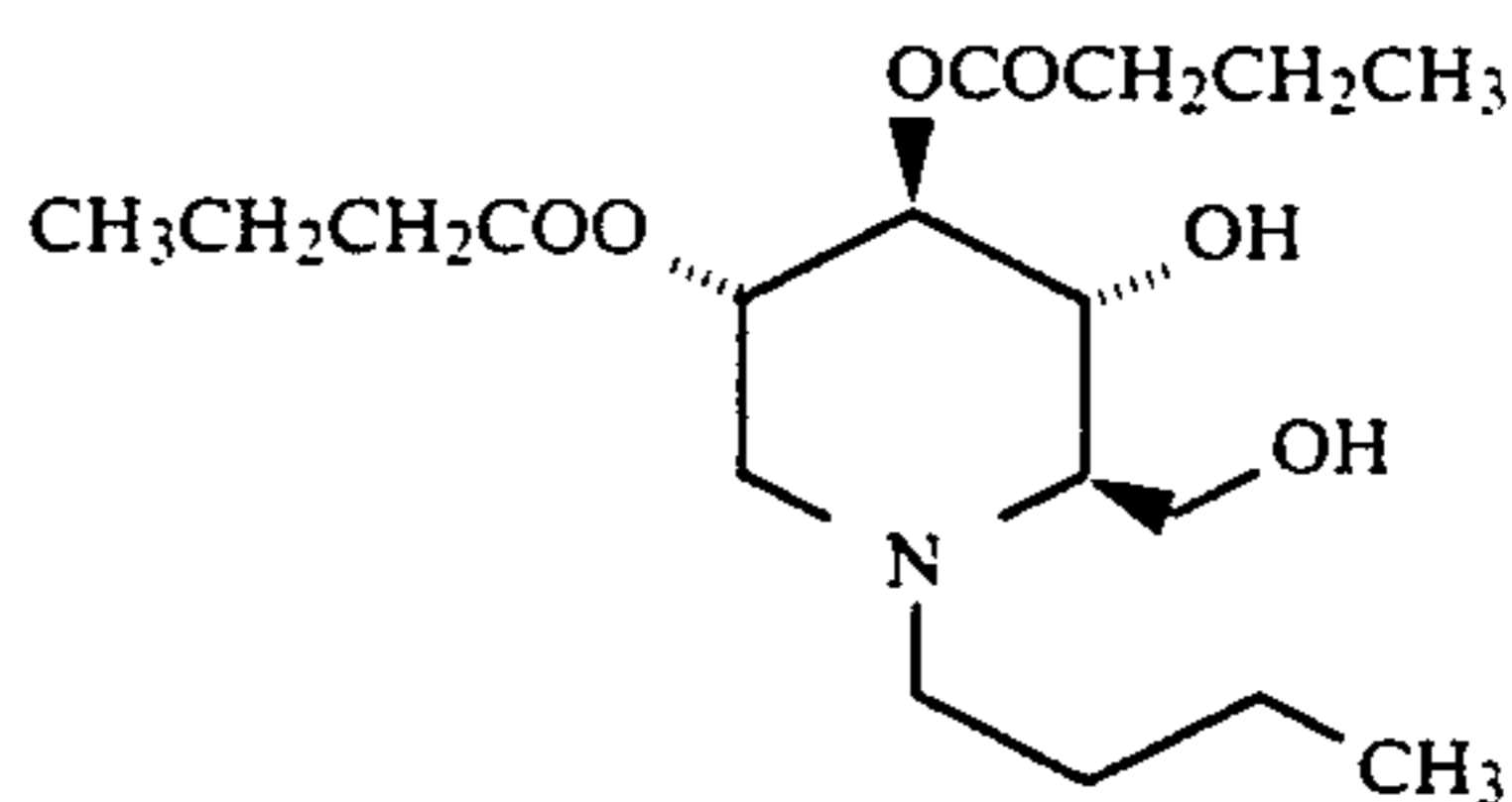
1,5-(Butylimino)-1,5-dideoxy-D-glucitol, 2,3-dibutyrate
