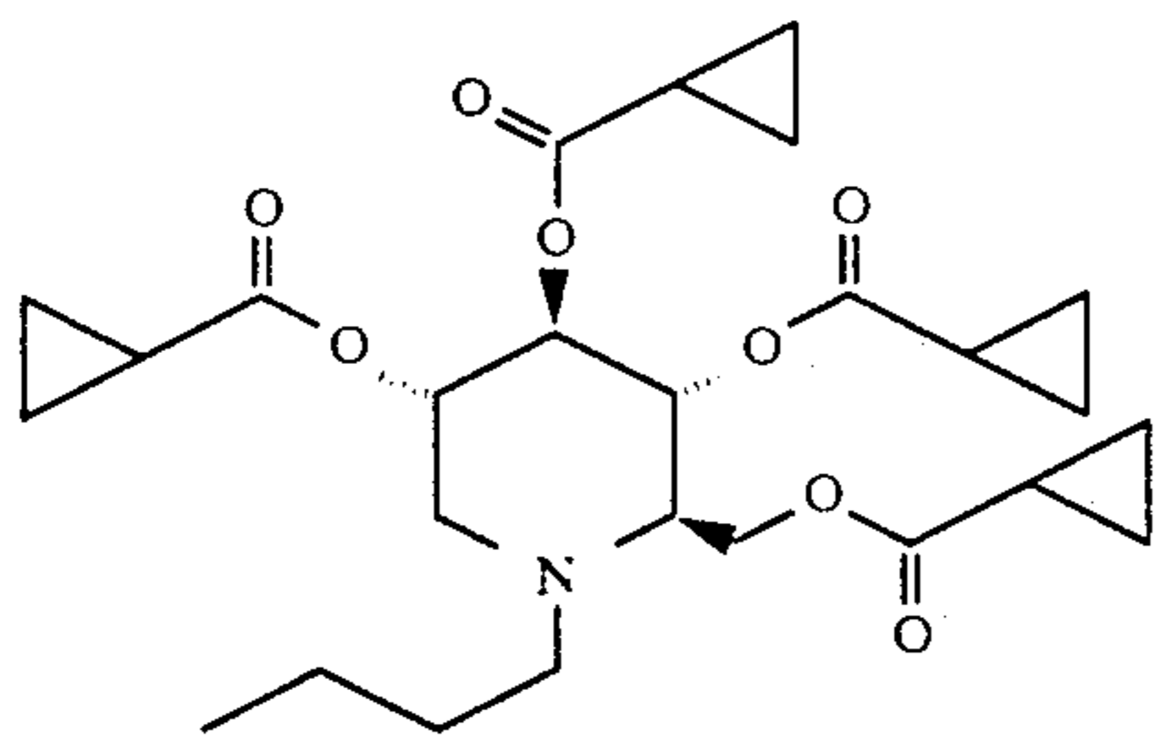
1,5-(Butylimino)-1,5-dideoxy-D-glucitol, tetra(cyclopropylcarboxylate)
