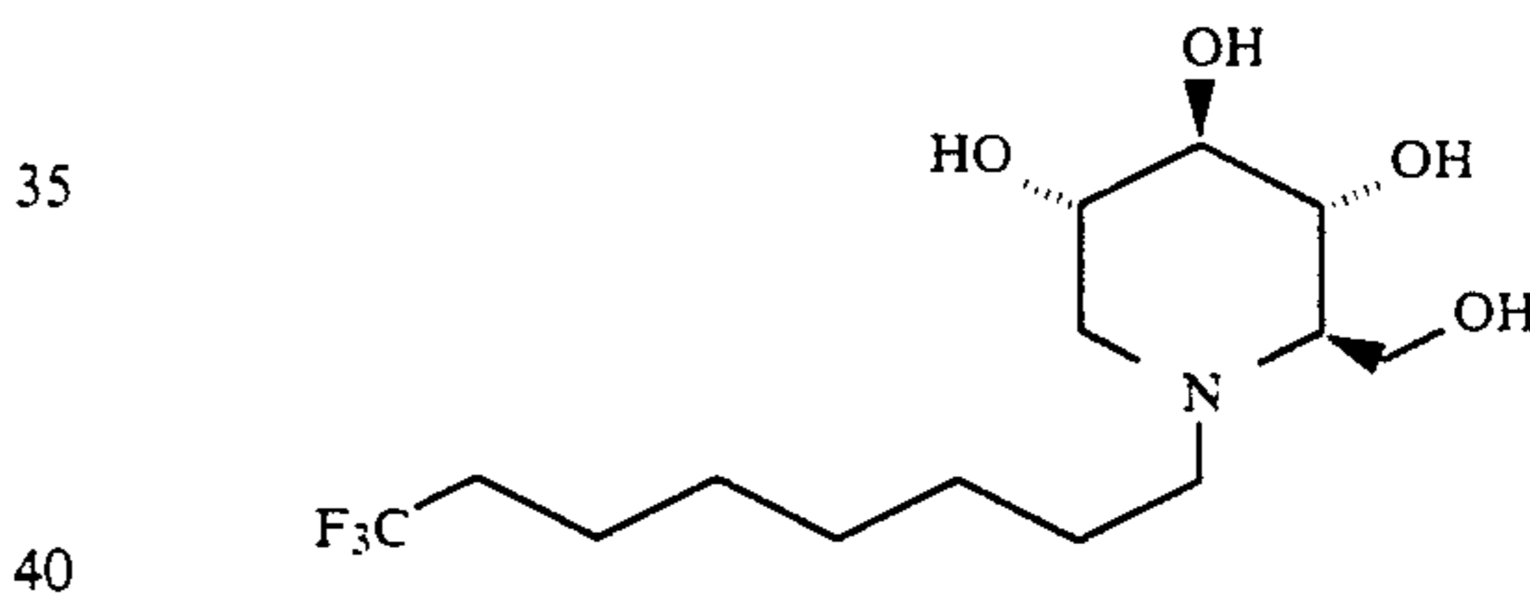
1,5-(8,8,8-Trifluorooctylimino)-1,5-dideoxy-D-glucitol
