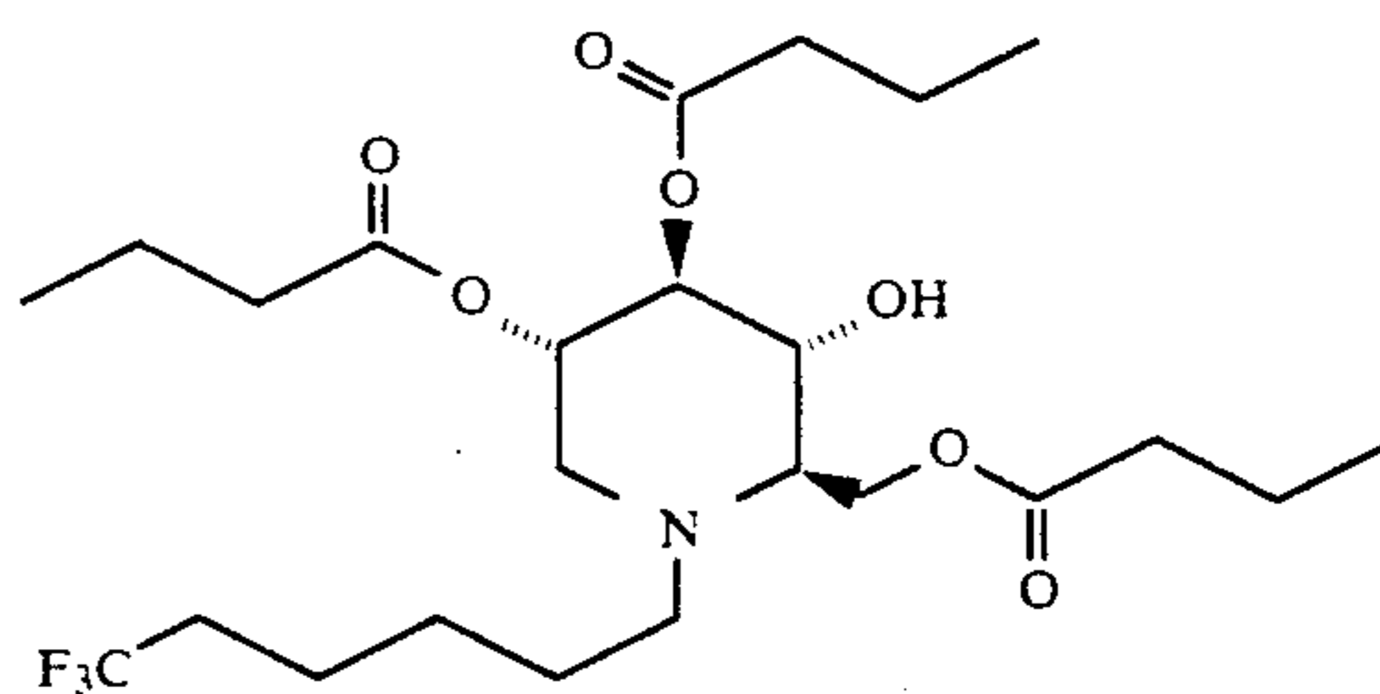
1,5-(6,6,6-Trifluorohexylimino)-1,5-dideoxy-D-glucitol, 2,3,6-tributyrates
