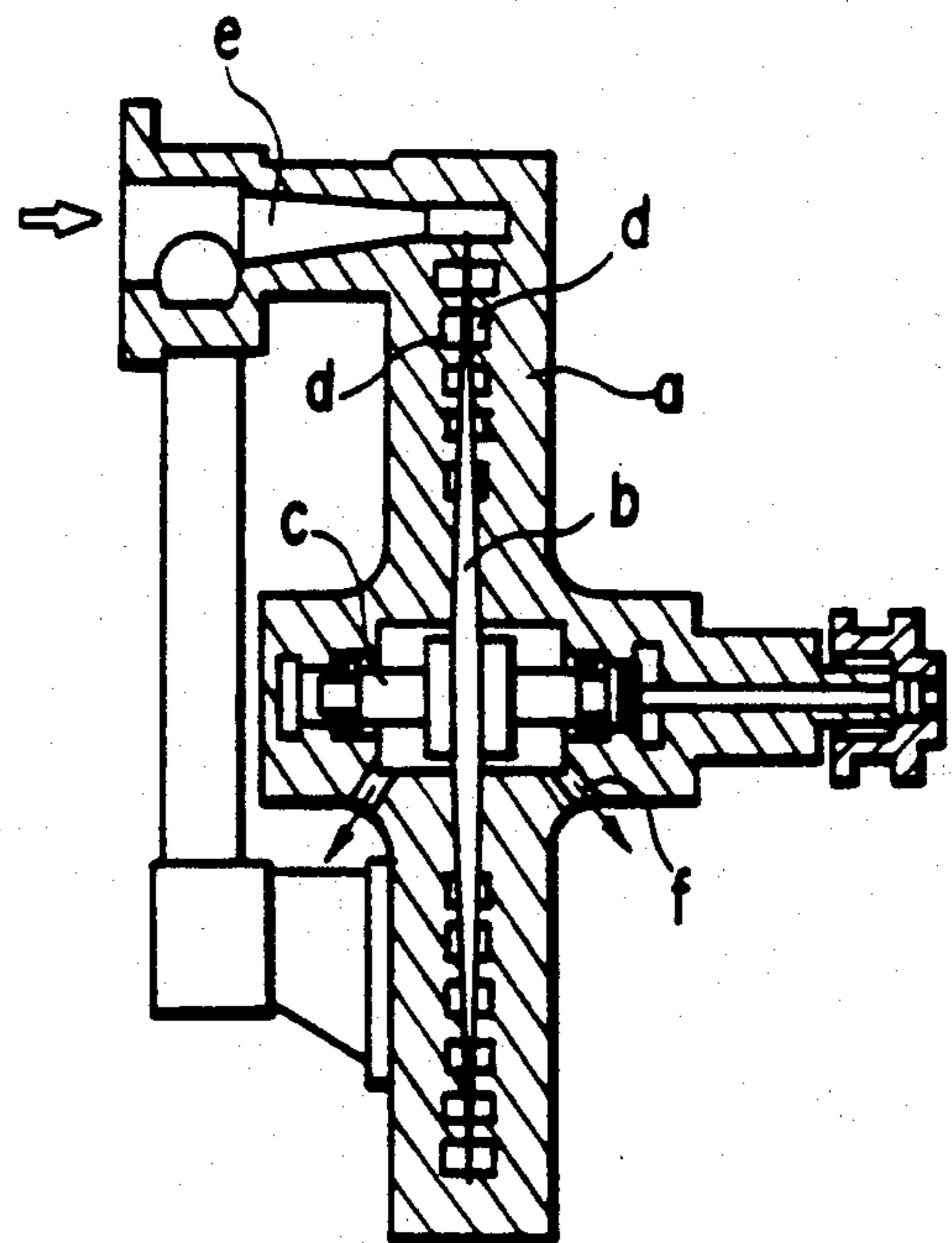
FIG. 50 PRIOR ART
