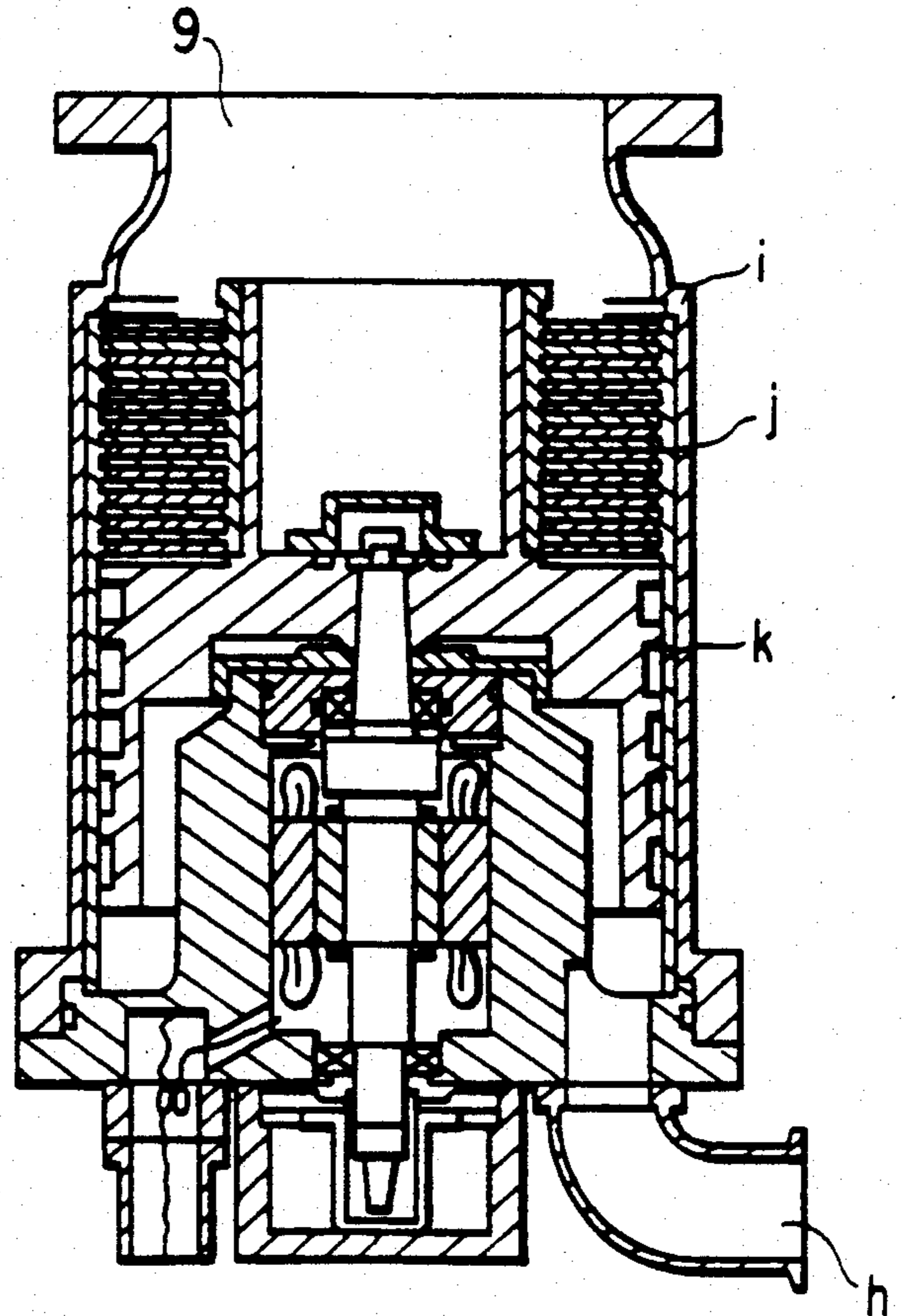
FIG. 26 PRIOR ART
