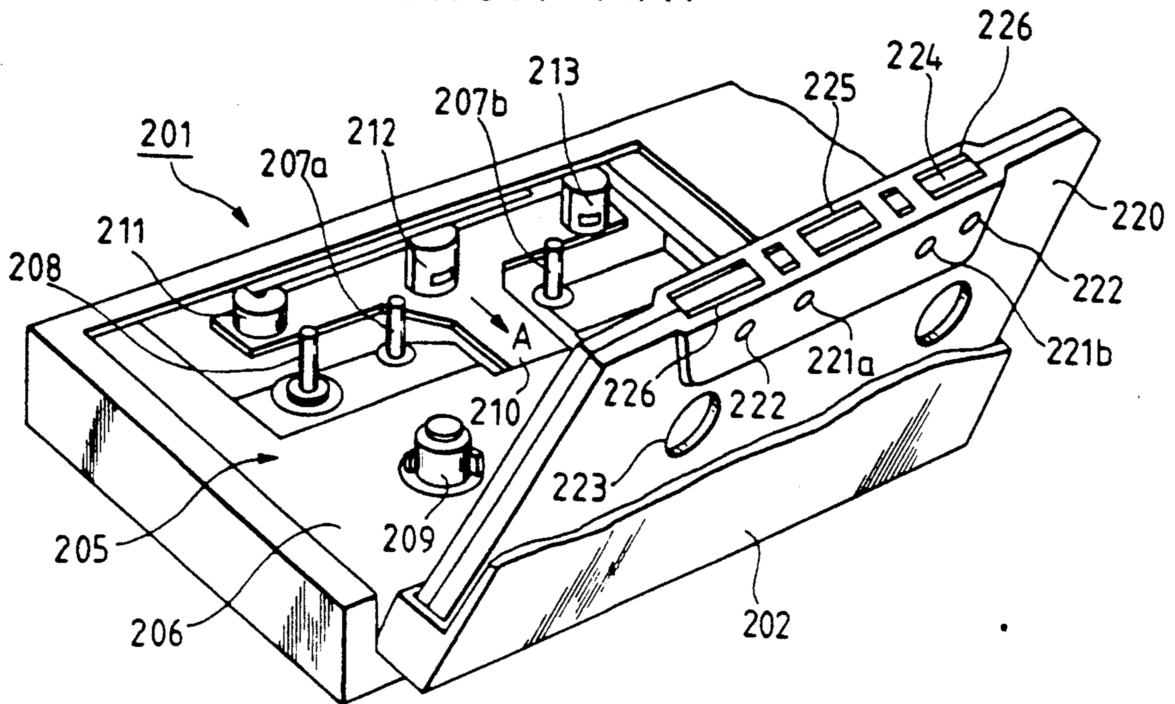
FIG. 1 PRIOR ART
