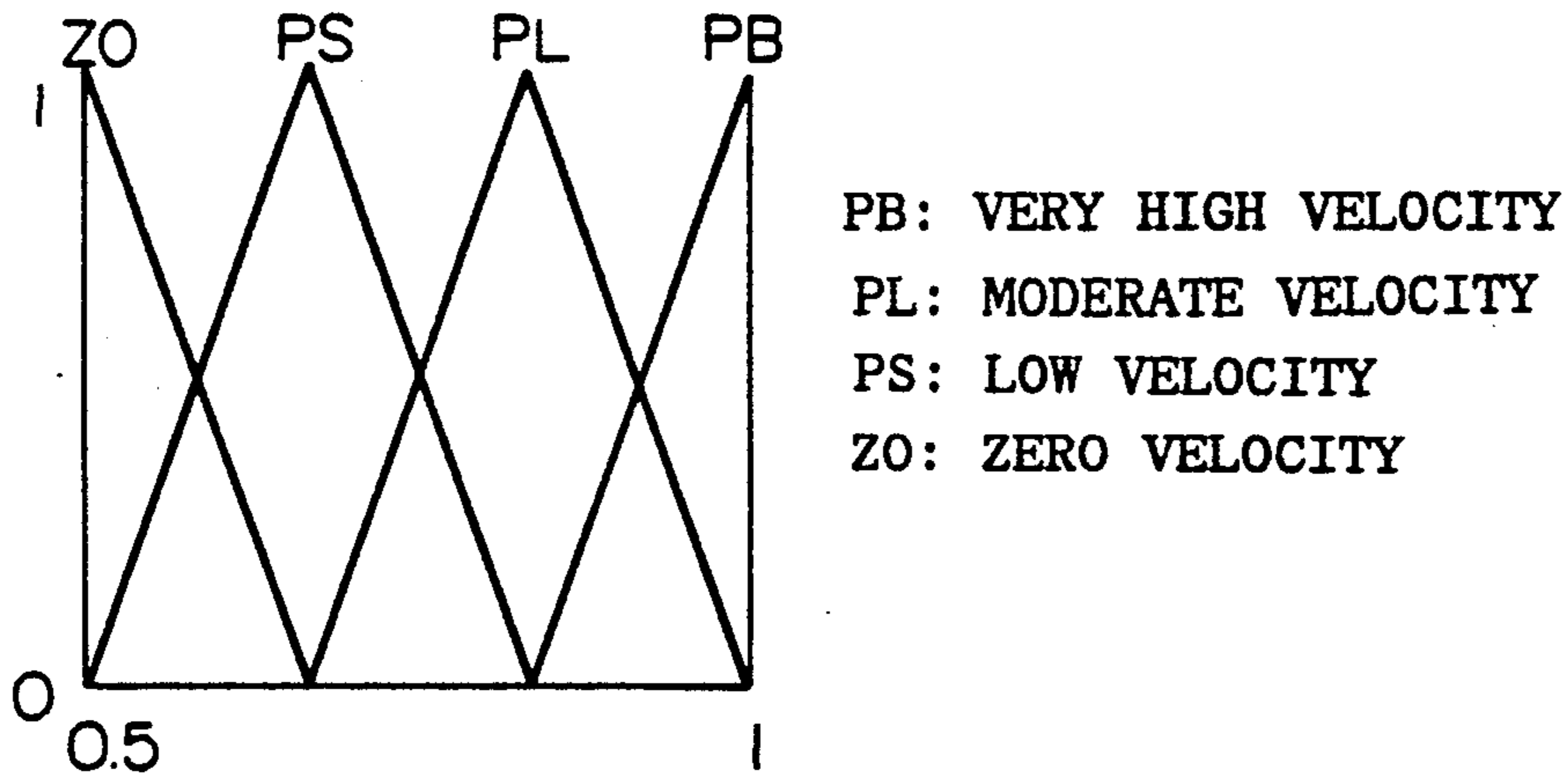
FIG.37 (MEMBERSHIP FUNCTION OF VELOCITY CONTROL COMMAND)
