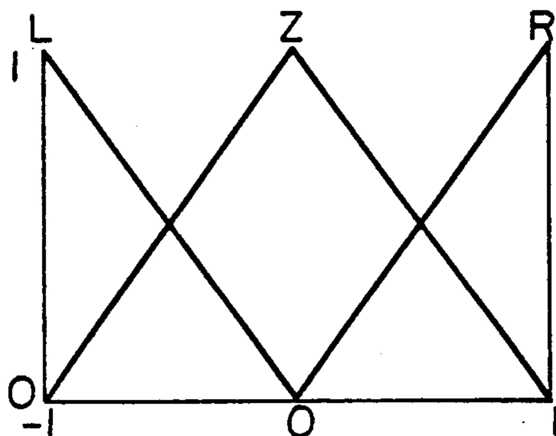
FIG.32 (MEMBERSHIP FUNCTION OF DEVIATION SIGNAL)
