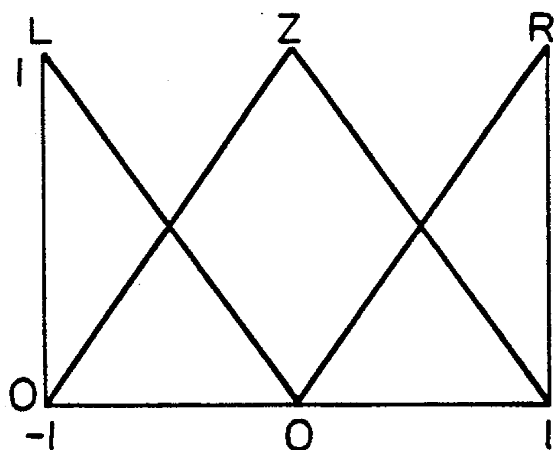
FIG.33 (MEMBERSHIP FUNCTION OF TIME-DIFFERENTIATED SIGNAL)
