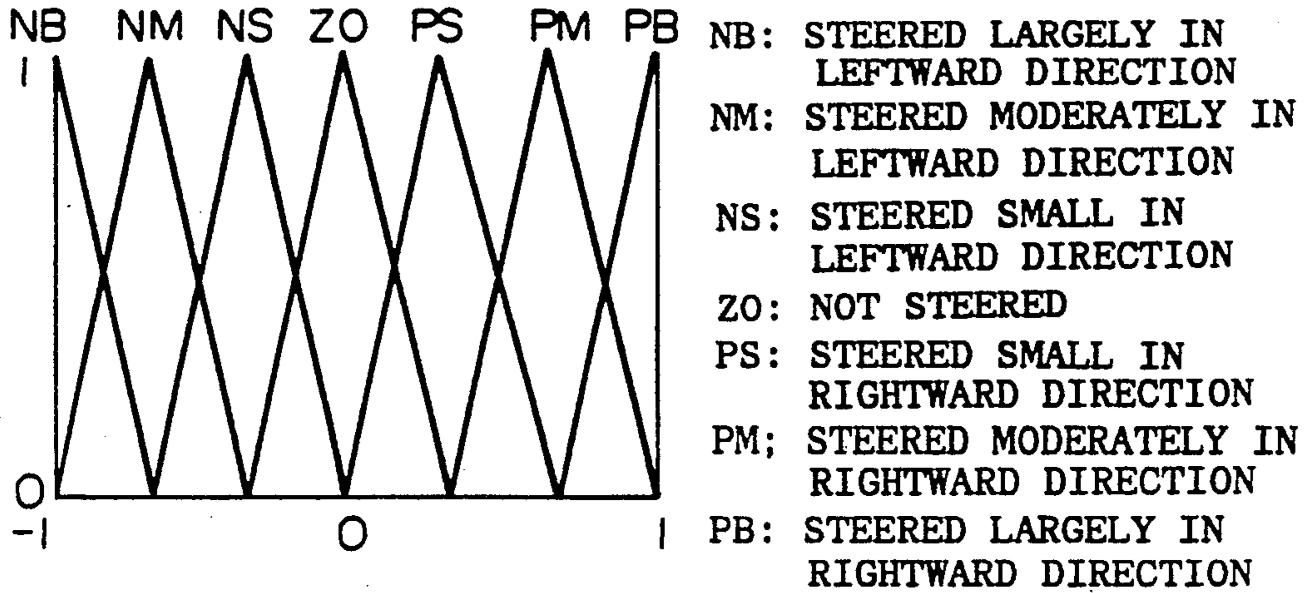
FIG.36 (MEMBERSHIP FUNCTION OF CURRENT VELOCITY)
