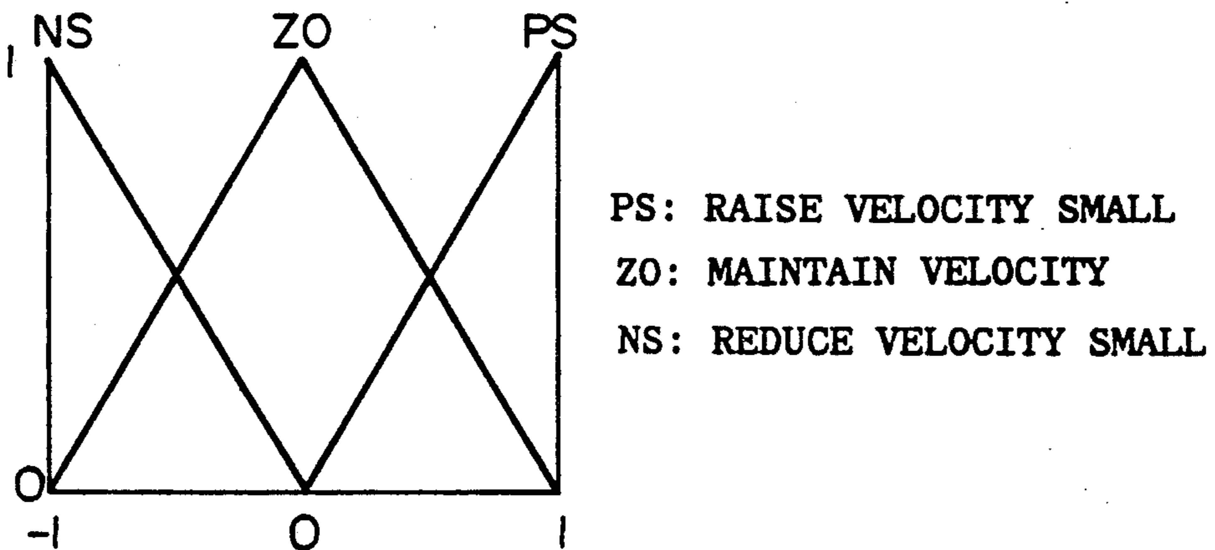
FIG.37 (MEMBERSHIP FUNCTION OF VELOCITY CONTROL COMMAND)
