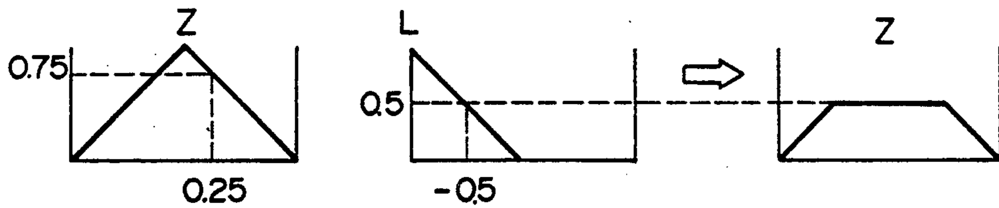
FIG.28B (EVALUATION OF REGULATION 4)
