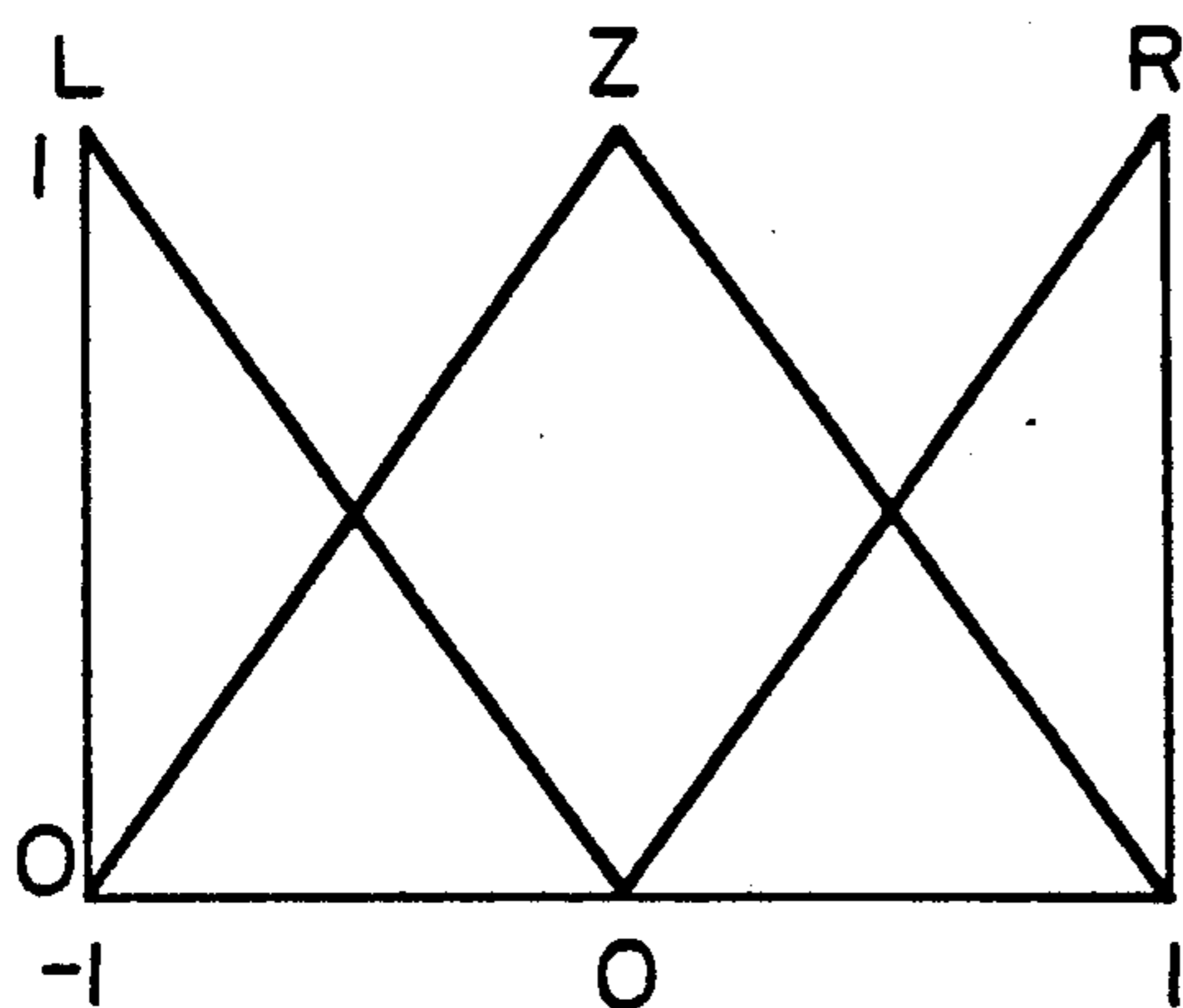
FIG.34 (MEMBERSHIP FUNCTION OF CURRENT STEERING ANGLE)
