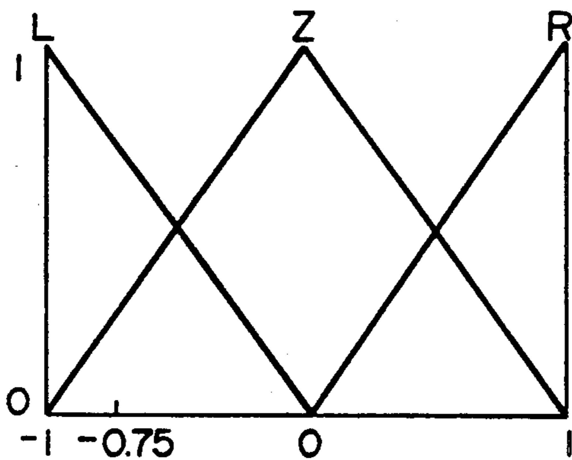
FIG. 12 (MEMBERSHIP FUNCTION OF CURRENT STEERING ANGLE G )
