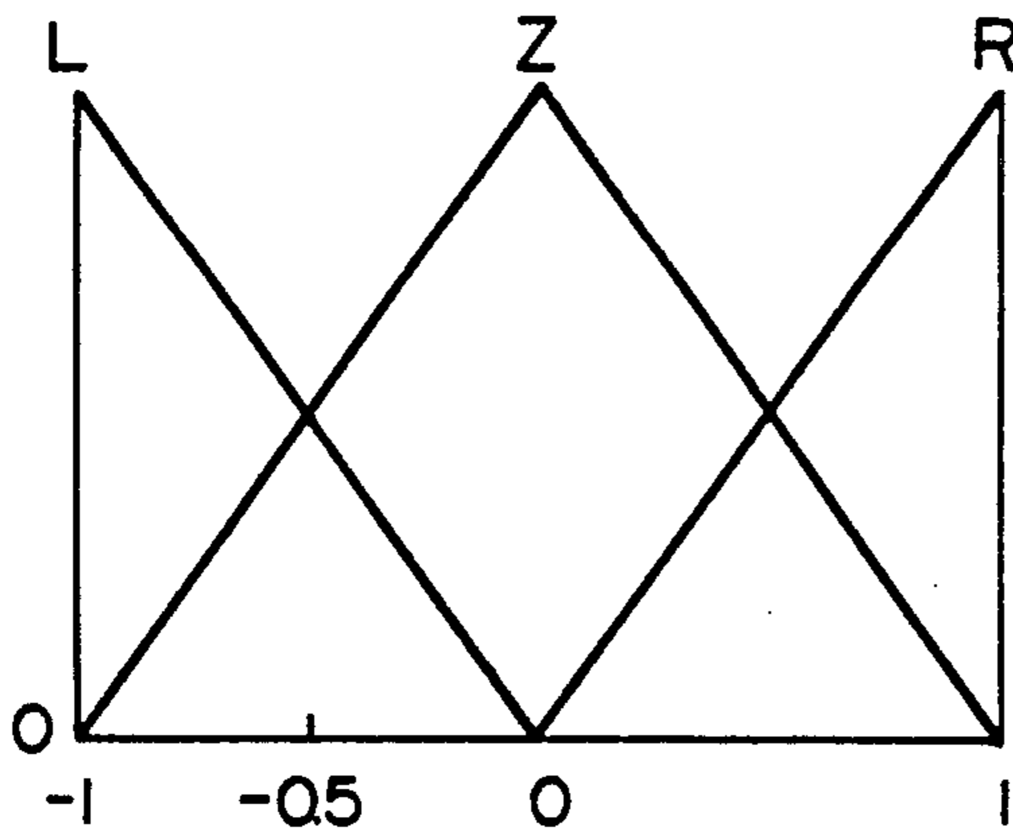
FIG. 11 (MEMBERSHIP FUNCTION OF TIME-DIFFERENTIATED SIGNAL \Delta^2 D )
