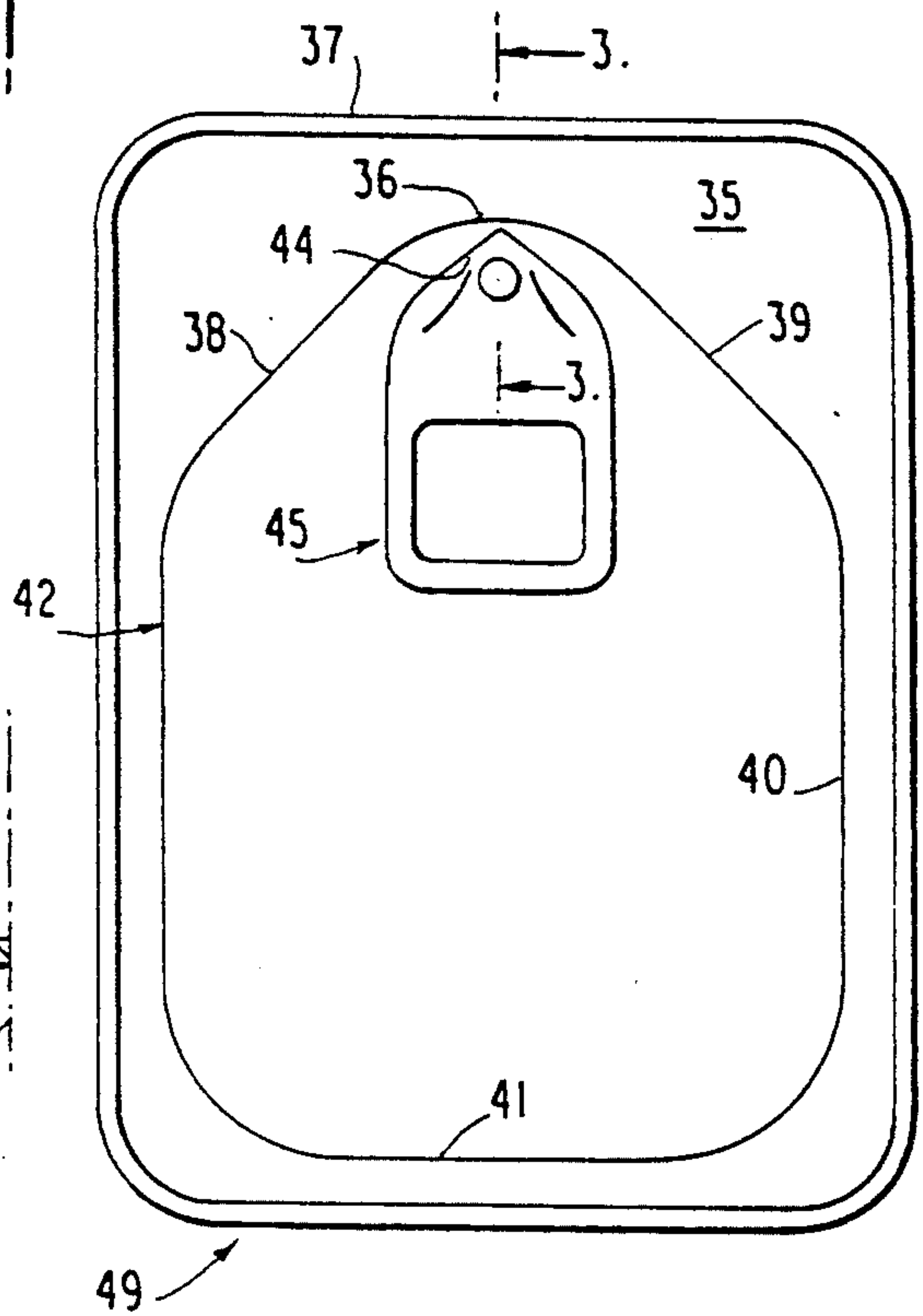
FIG. 2 PRIOR ART
