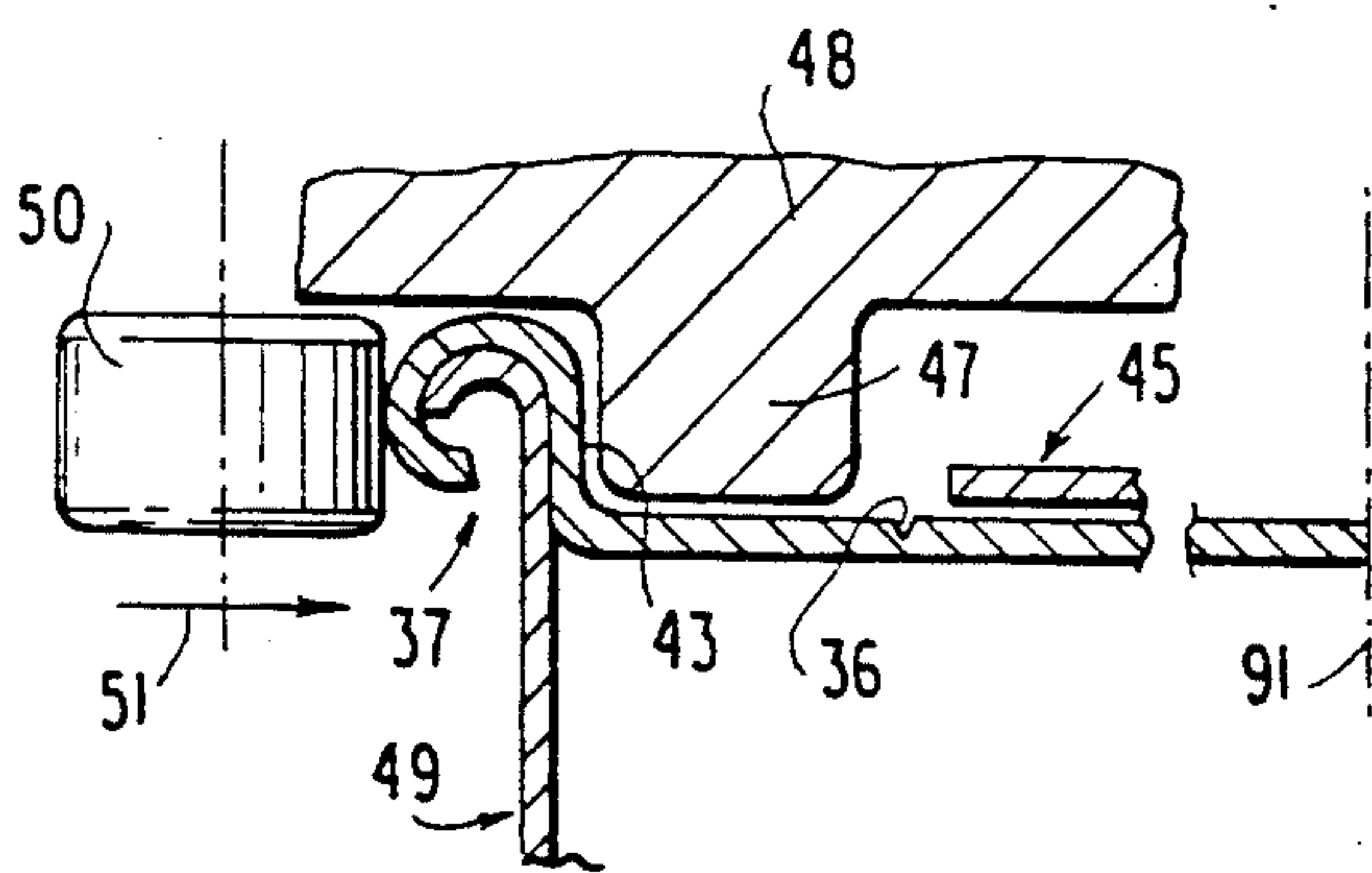
FIG. 3 PRIOR ART
