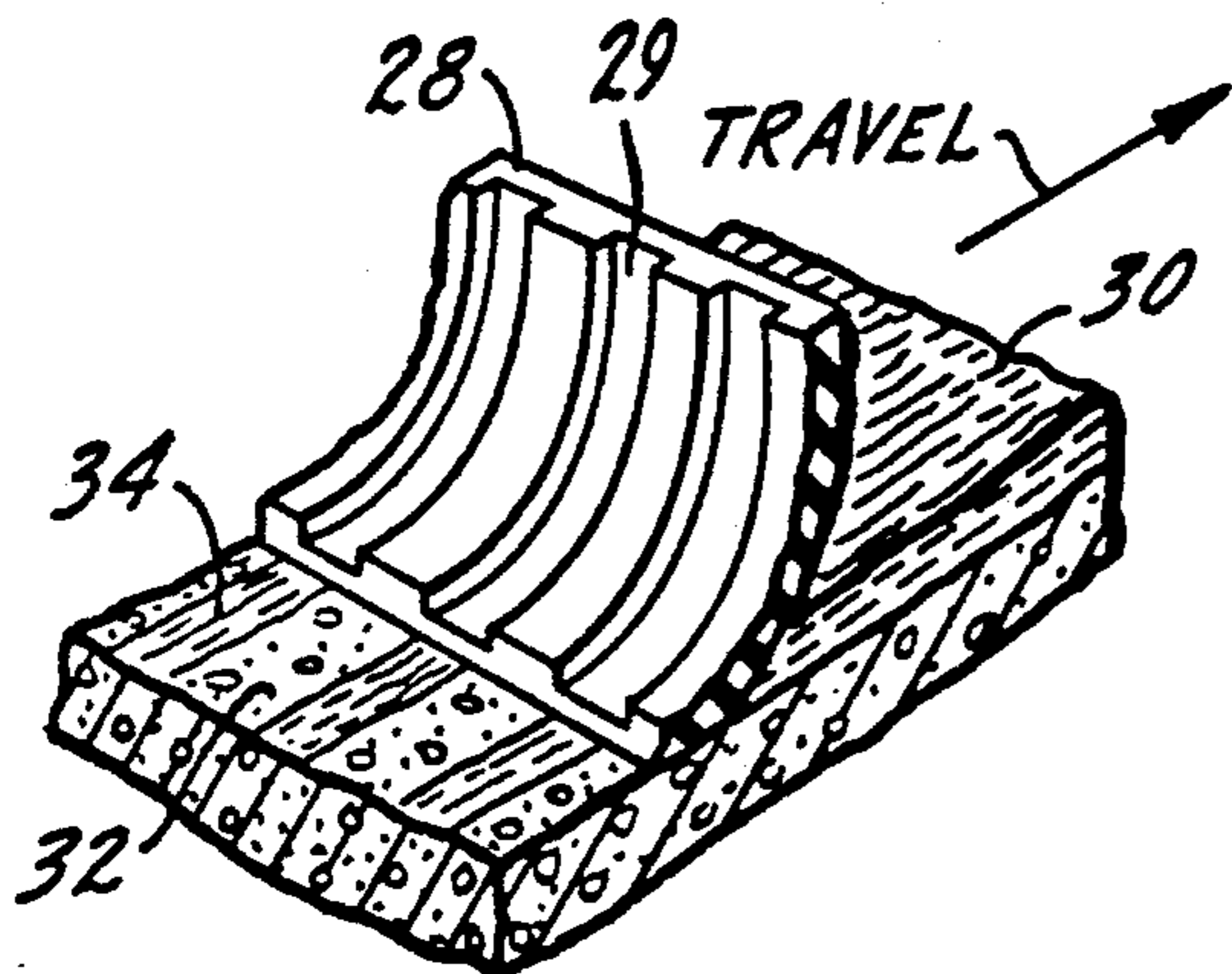
FIG. 6. (PRIOR ART)
