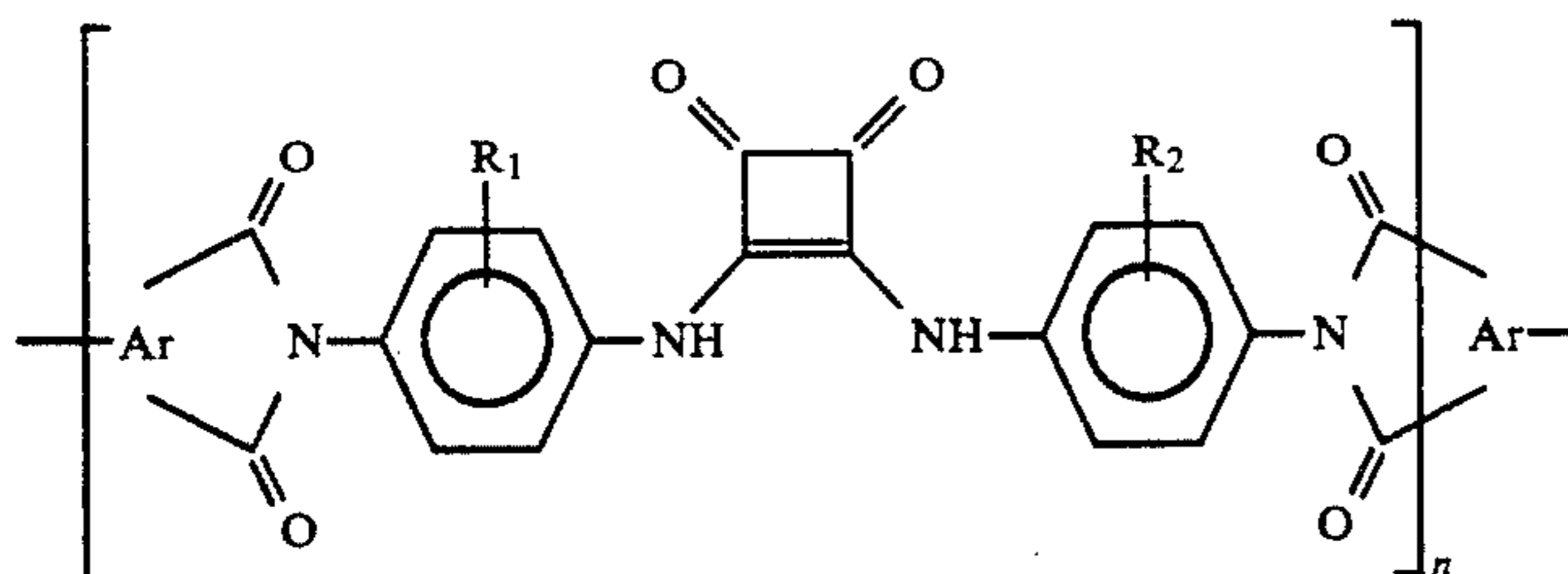
SCHEME I
