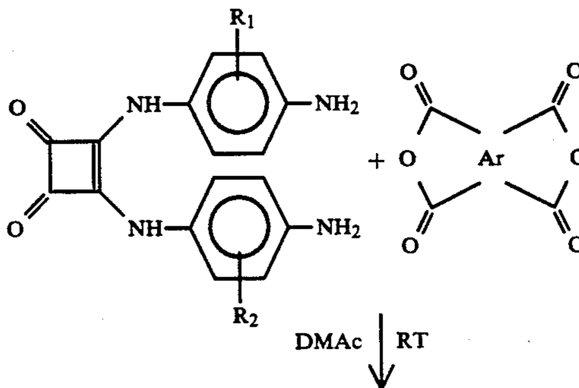
SCHEME I
