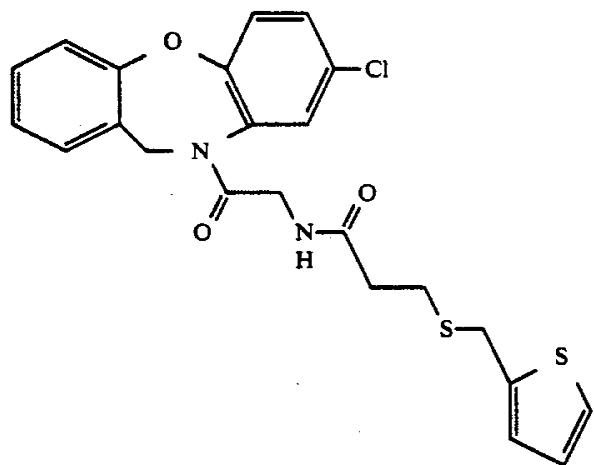
(a) Preparation of 2-thiophenemethanethiol
