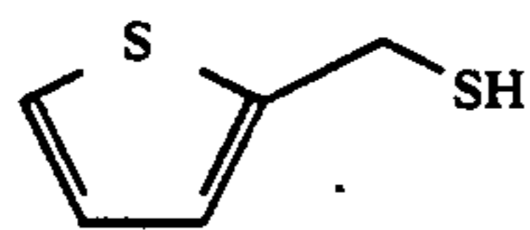
(a) Preparation of 2-thiophenemethanethiol
