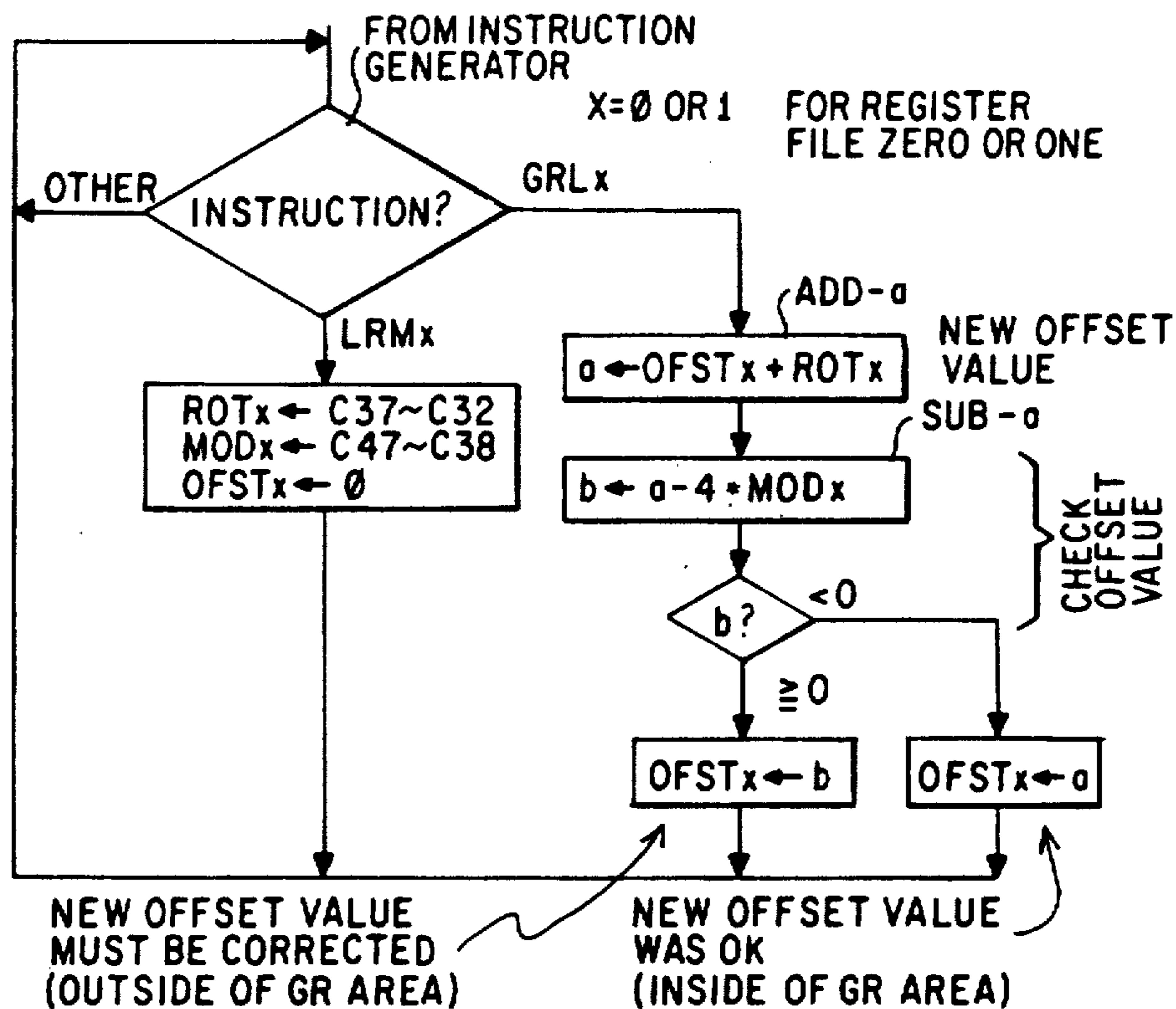
FUNCTION OF LRM0, LRM1 GRL0, GRL1 Fig.46a
