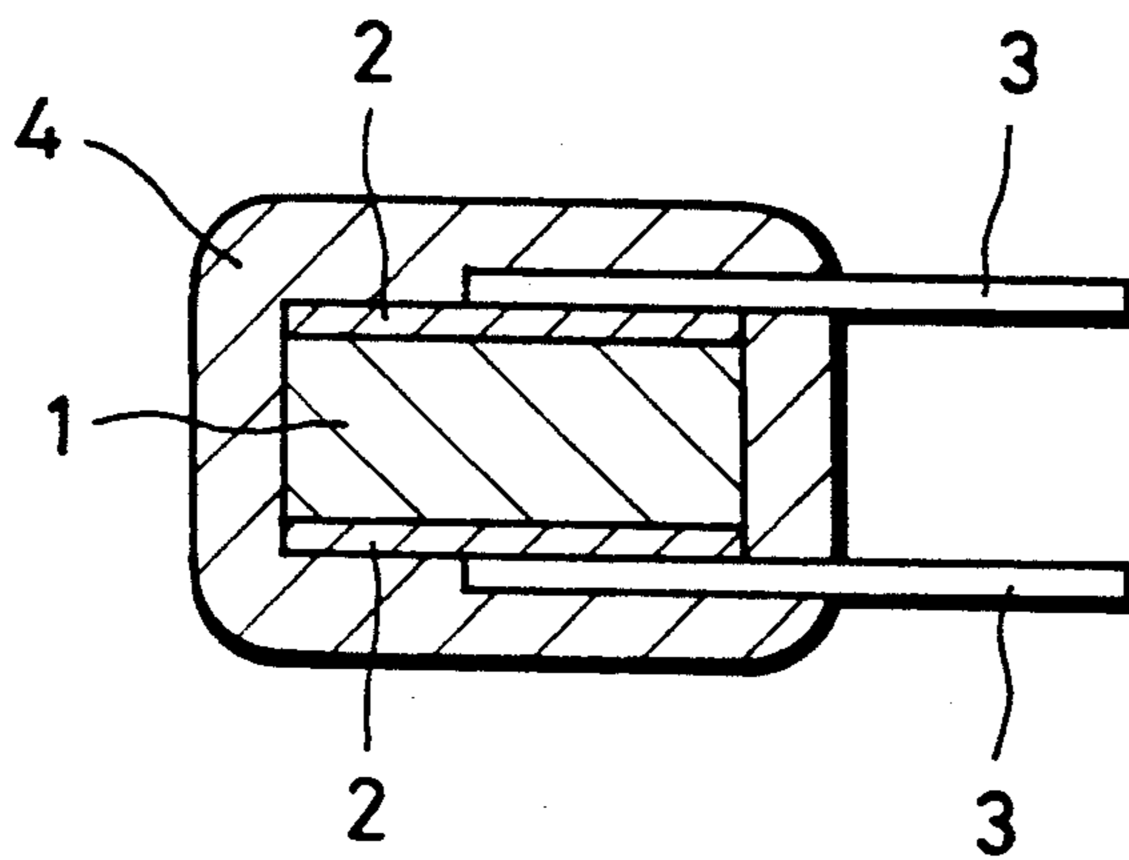
FIG. 6 (PRIOR ART)
