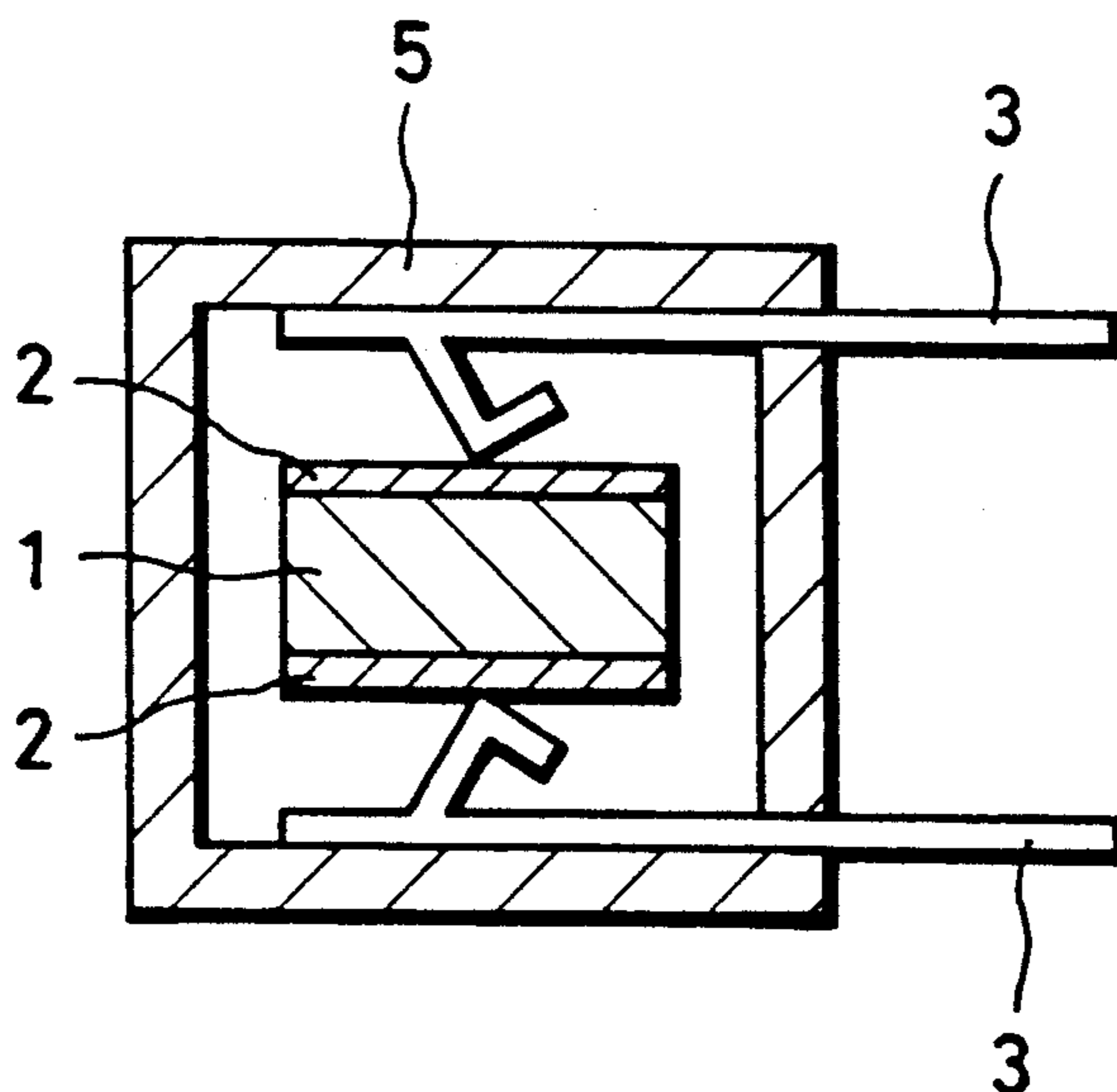
FIG. 7 (PRIOR ART)
