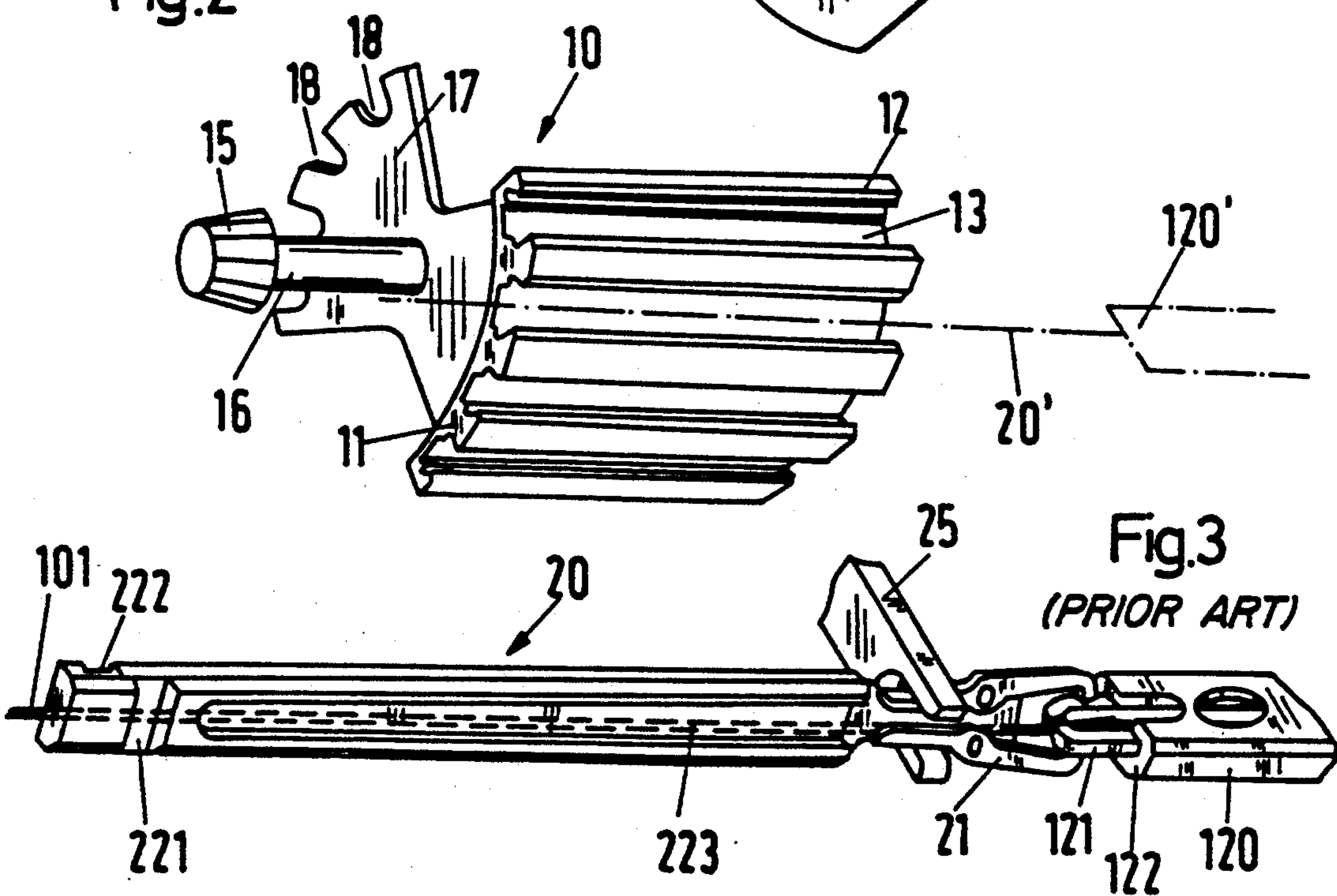
Fig.2 (PRIOR ART)
