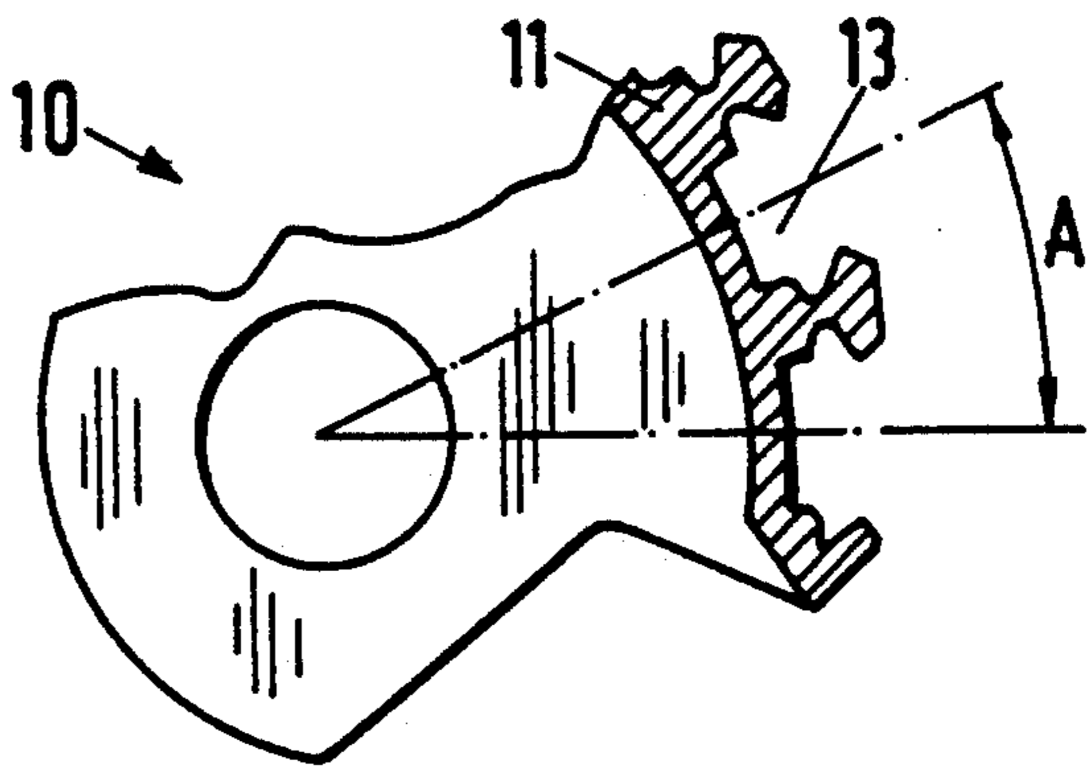
Fig.4 (PRIOR ART)
