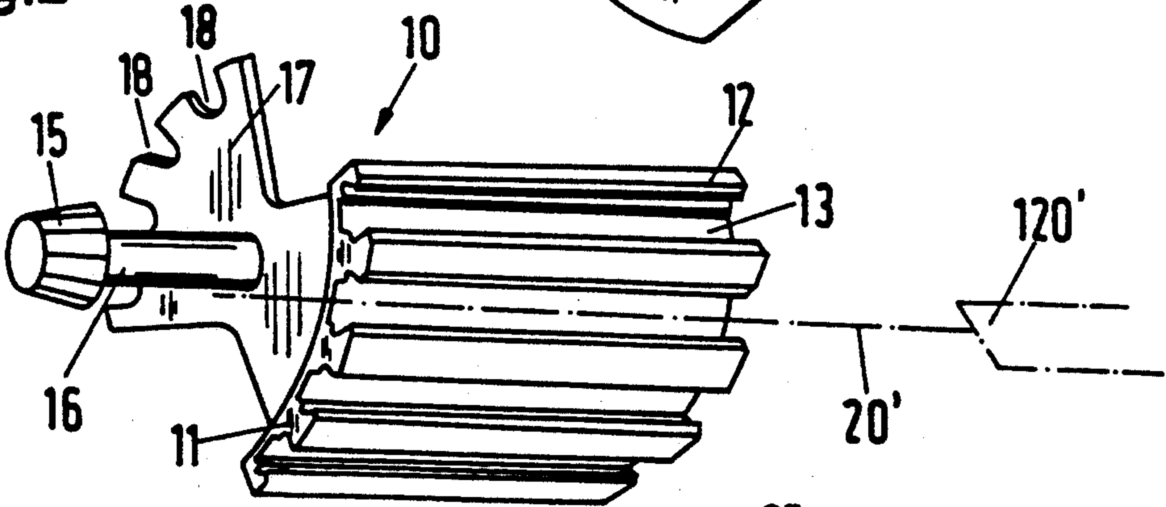
Fig.3 (PRIOR ART)
