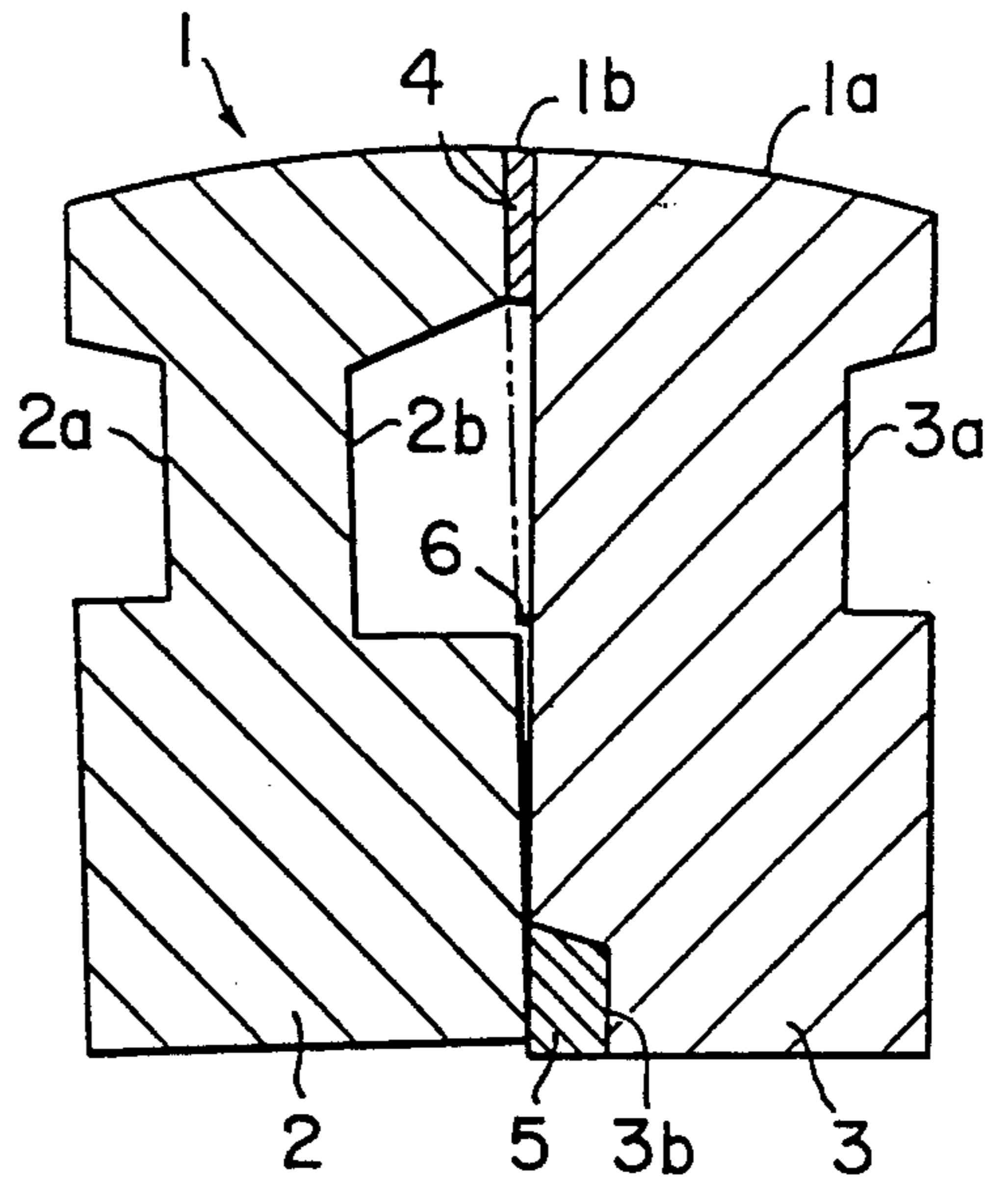
FIG. 1C PRIOR ART
