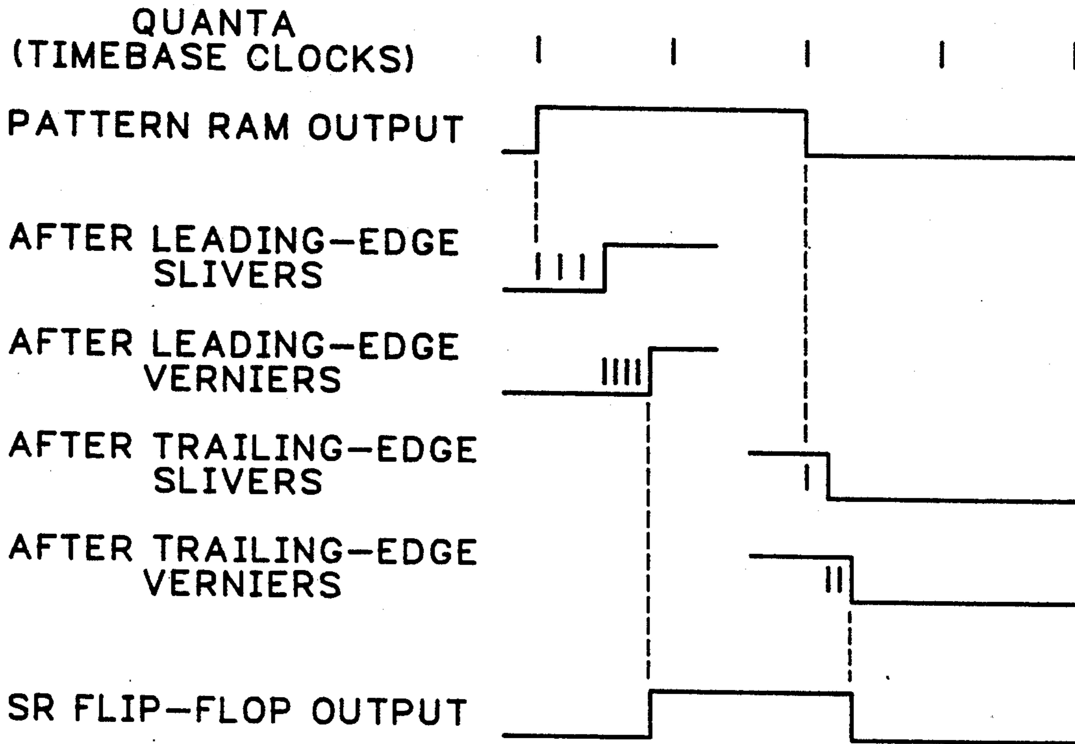
FIG. 9A USE OF SLIVERS AND VERNIERS
