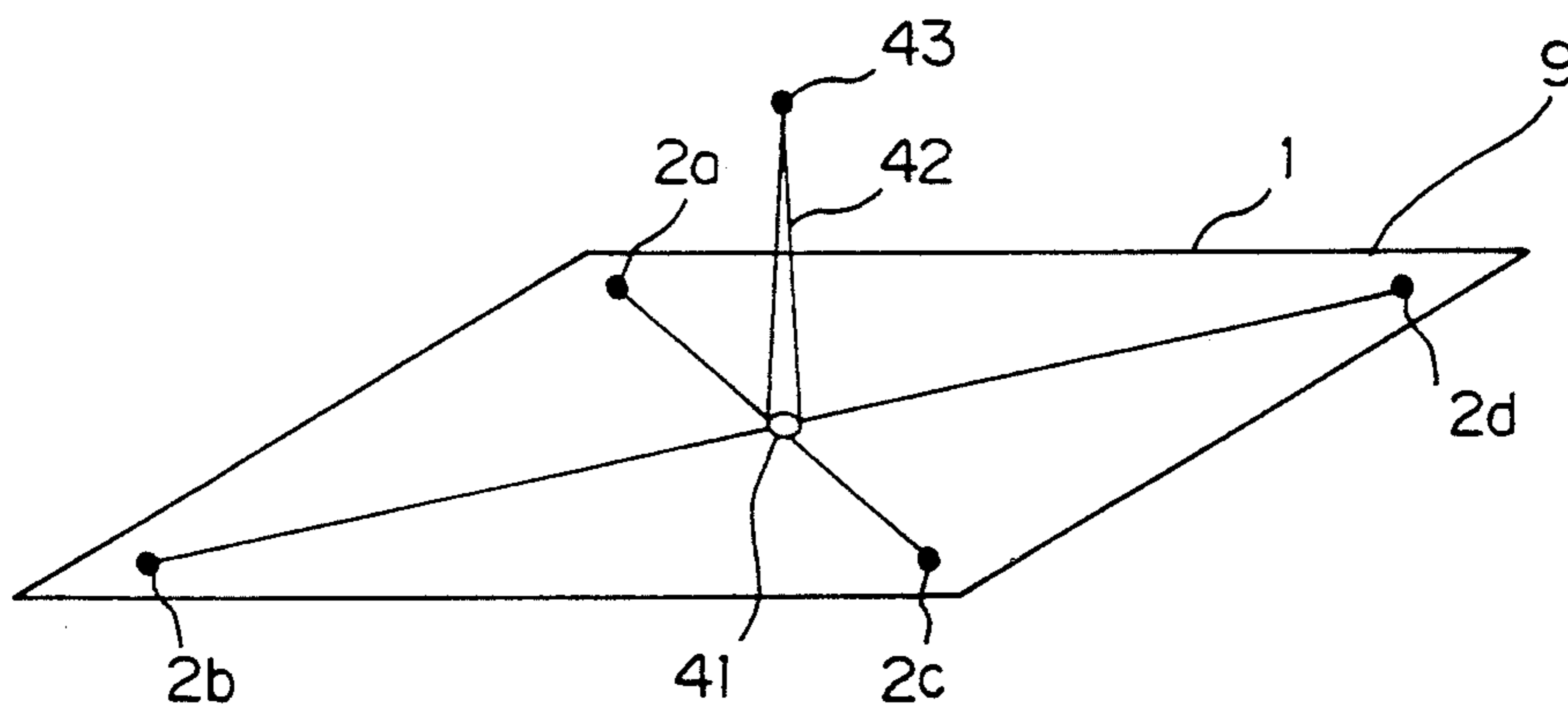
Fig. 9 (PRIOR ART)
