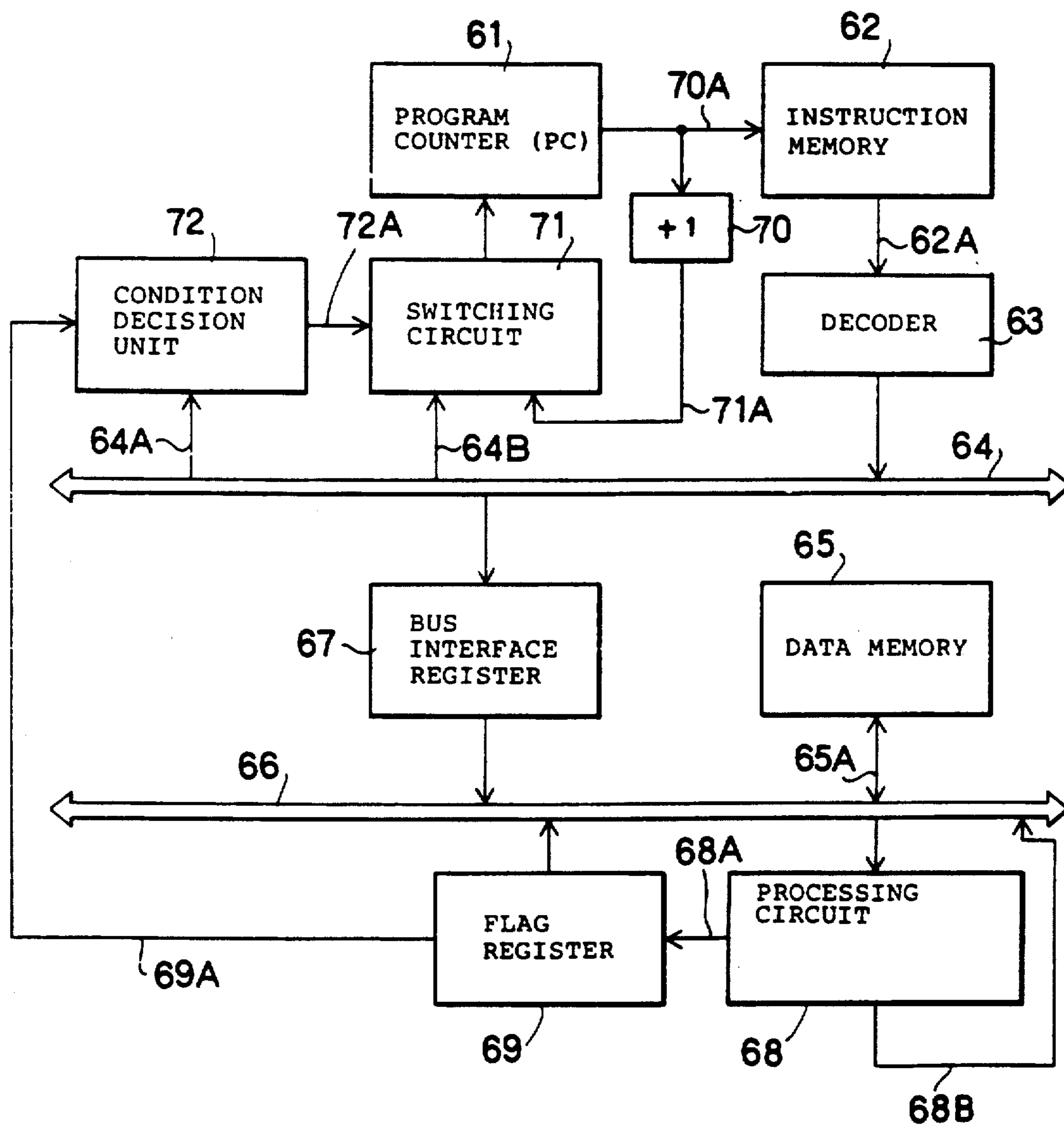
FIG. 6 (PRIOR ART)
