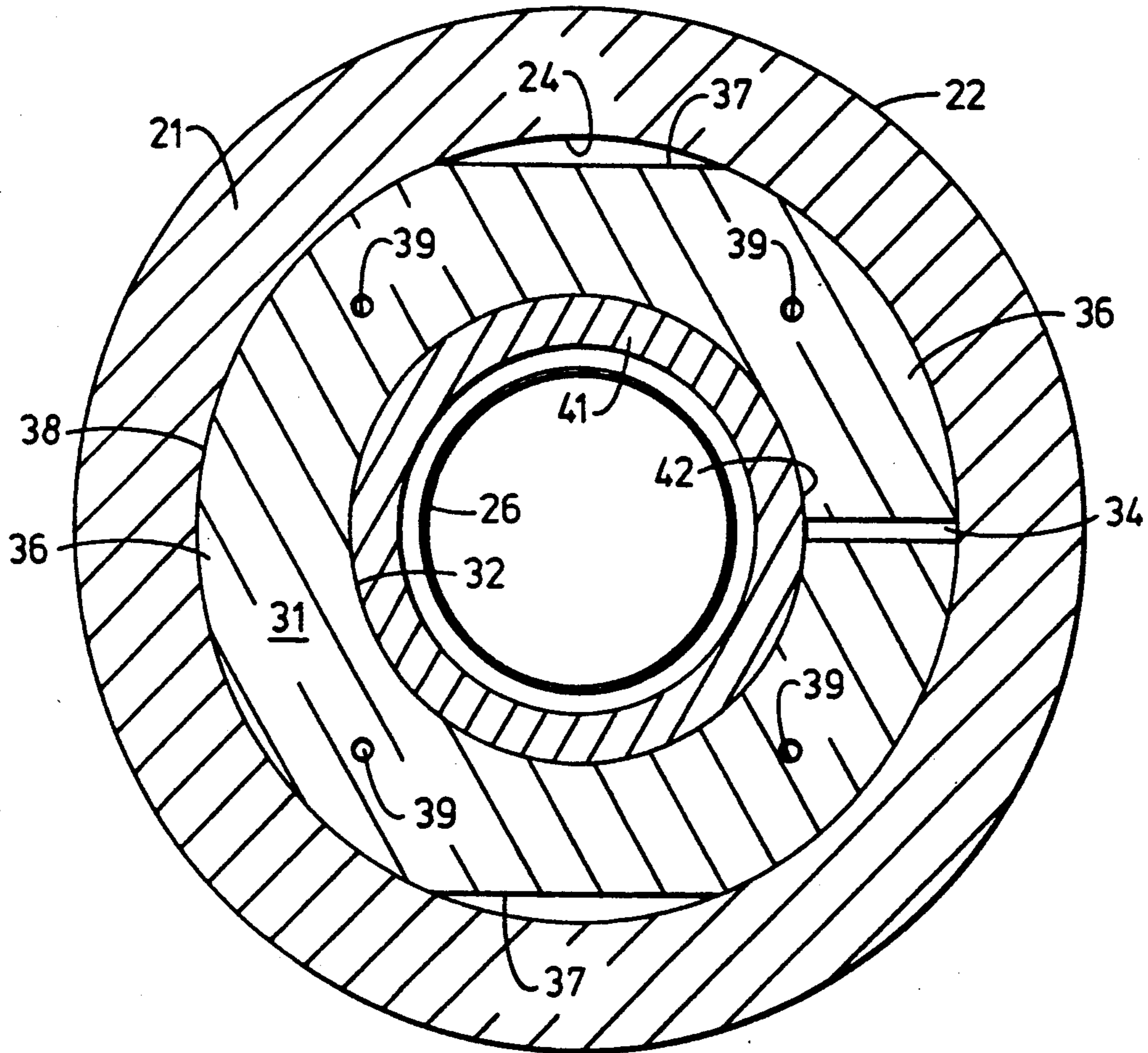
FIG. 2 (PRIOR ART)
