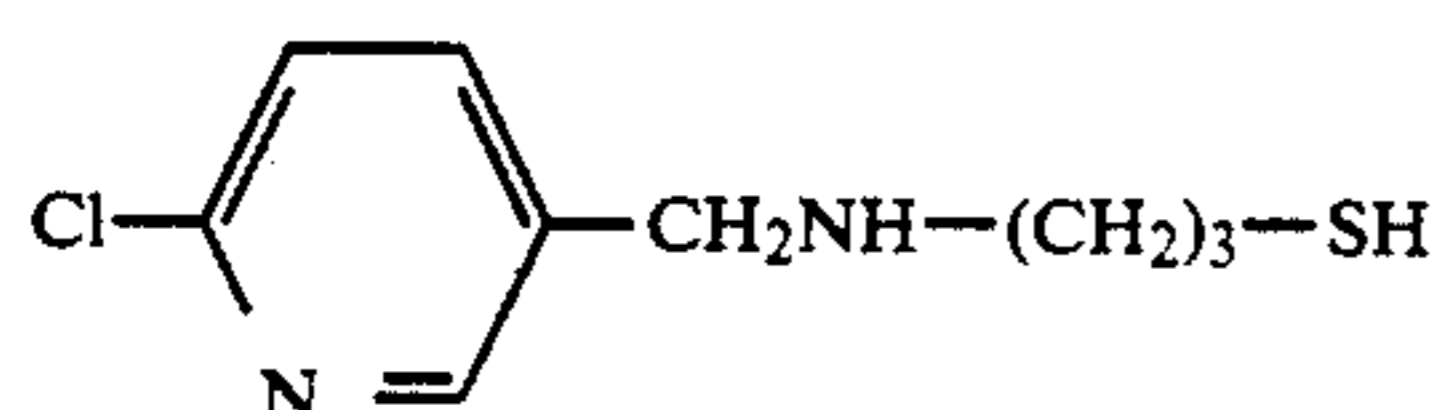
N-(2-chloro-5-pyridylmethyl)3-aminopropanethiol ( n_D^{22} : 1.5890)
