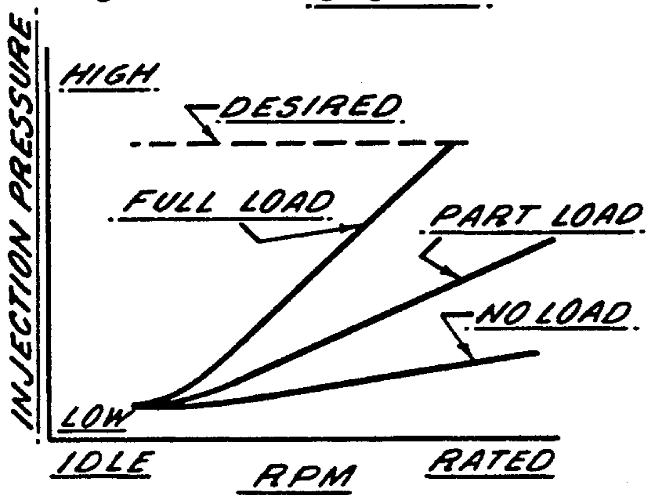
Fig. 9. CONVENTIONAL SYSTEM.
