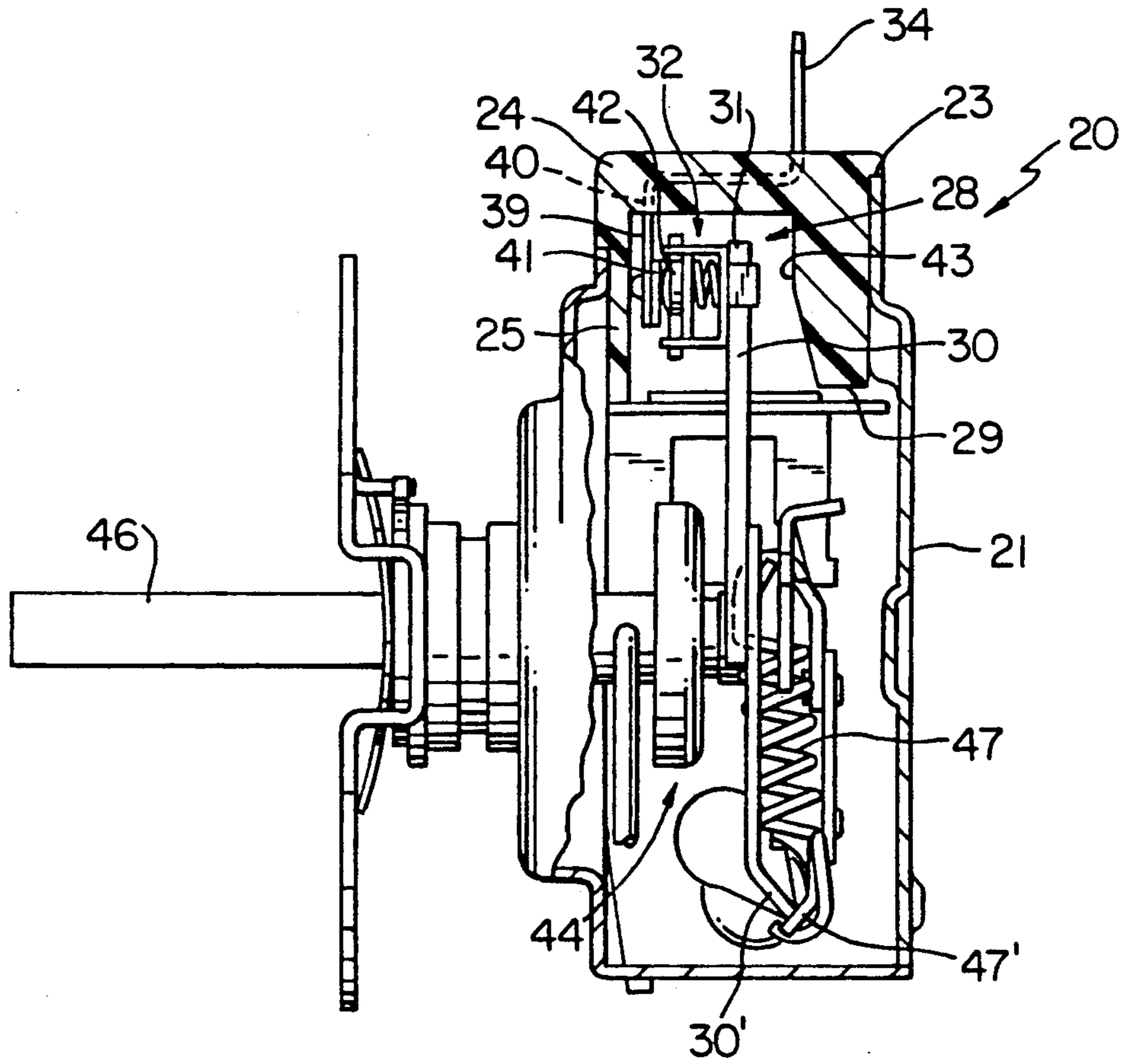
FIG. 2 PRIOR ART
