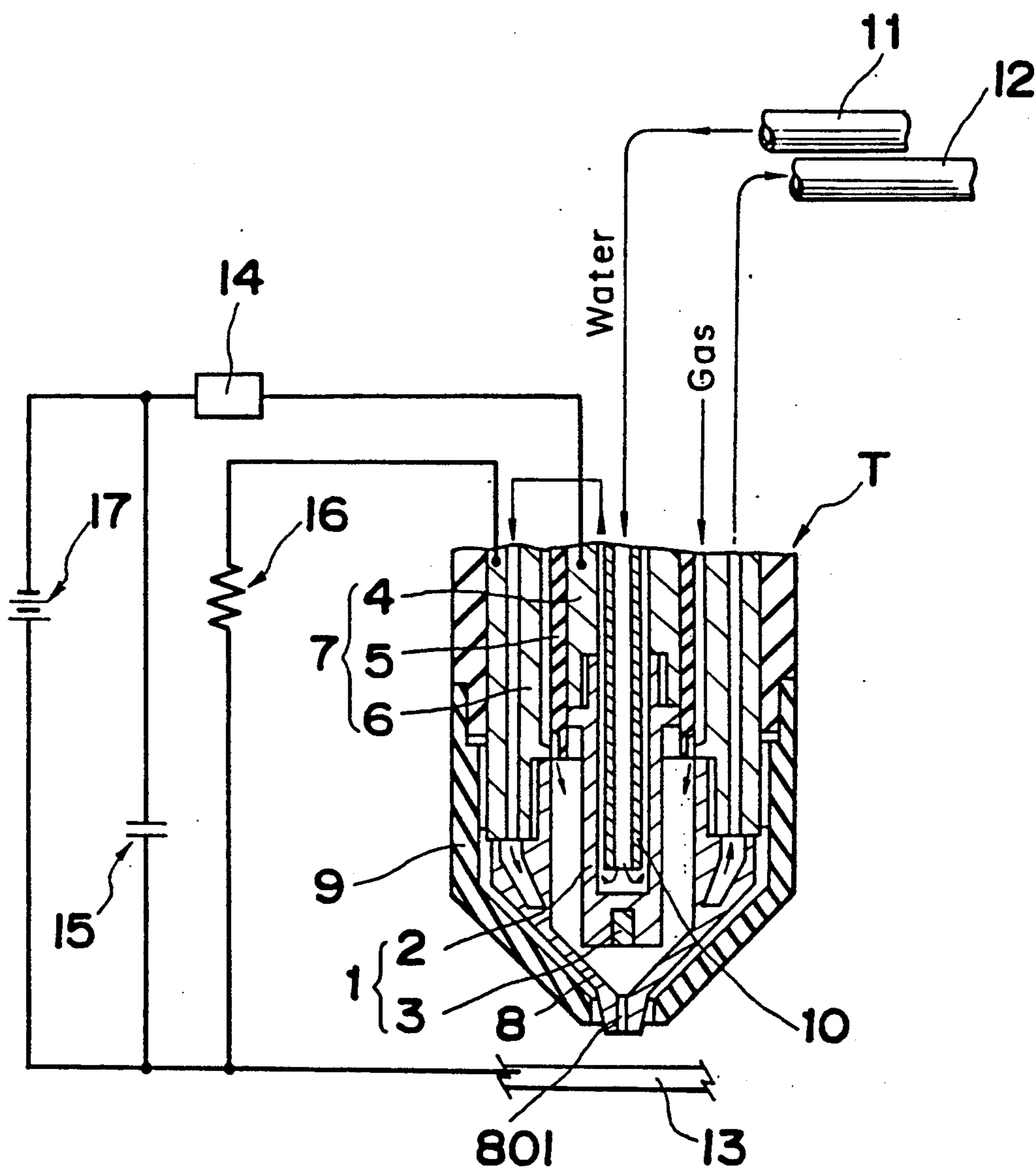
Fig. 7 PRIOR ART
