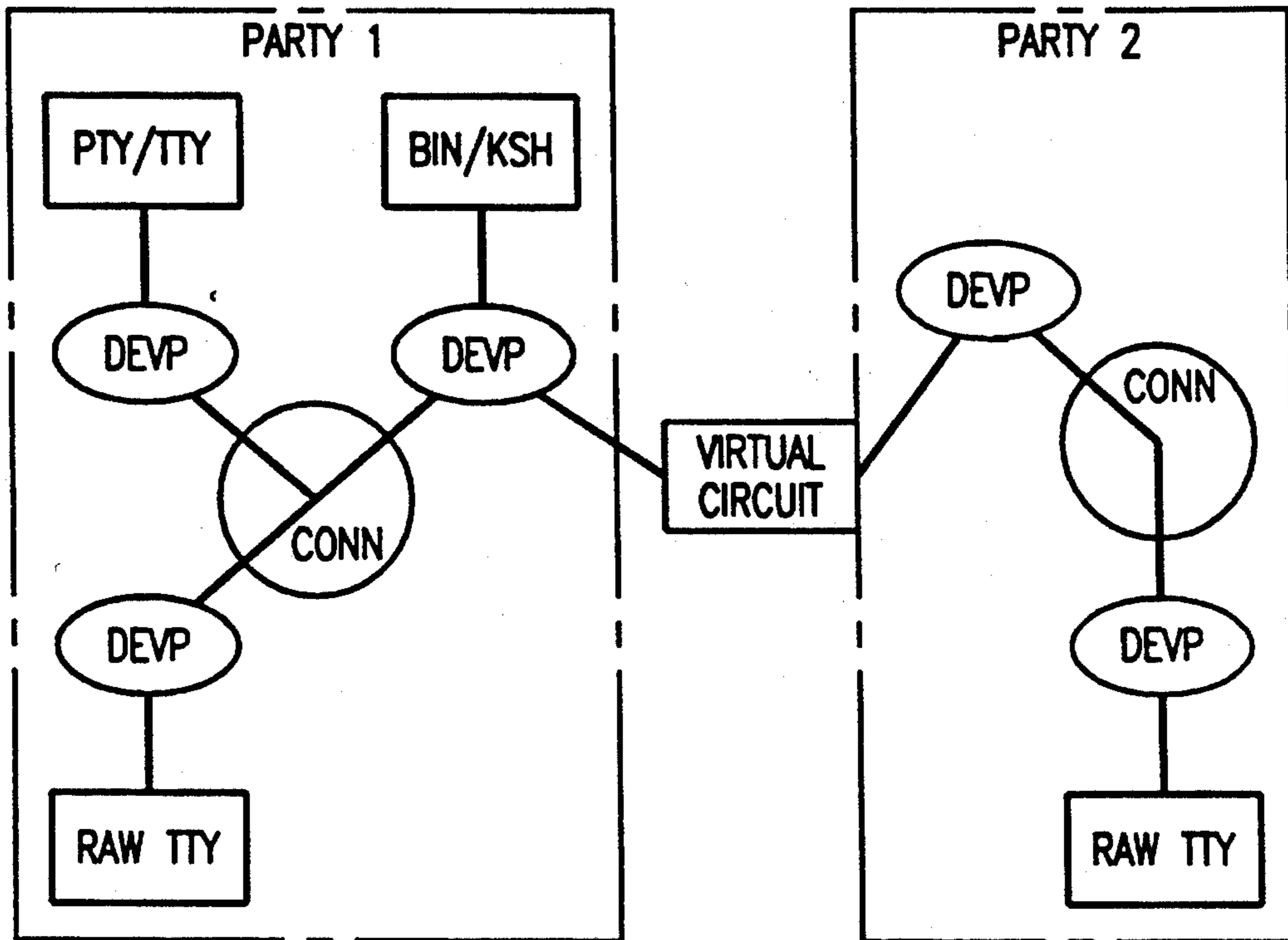
CONFIGURATION OF CHARACTER-BASED APPLICATION FIG. 14
