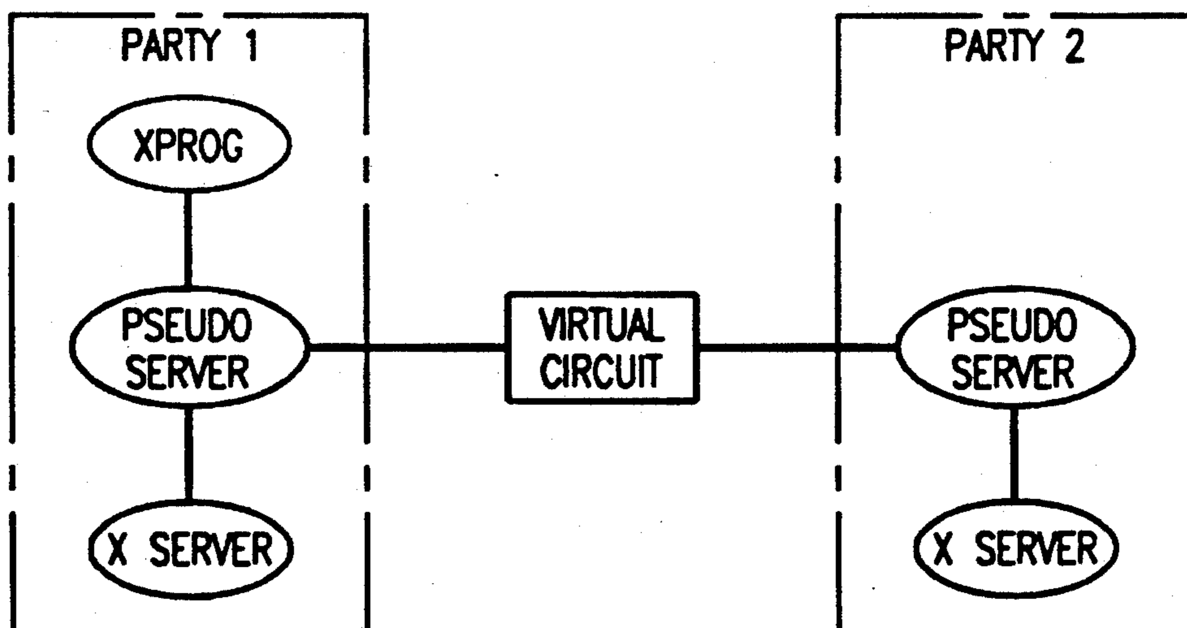
CONFIGURATION OF X WINDOW-BASED APPLICATION FIG. 15
