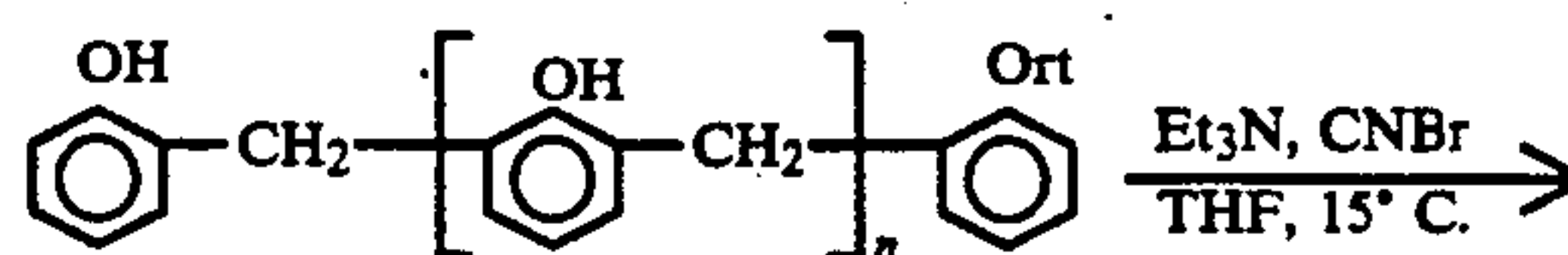
Phenolic backbone
