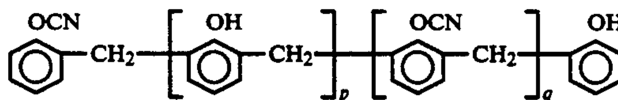
Phenolic Cyanate
