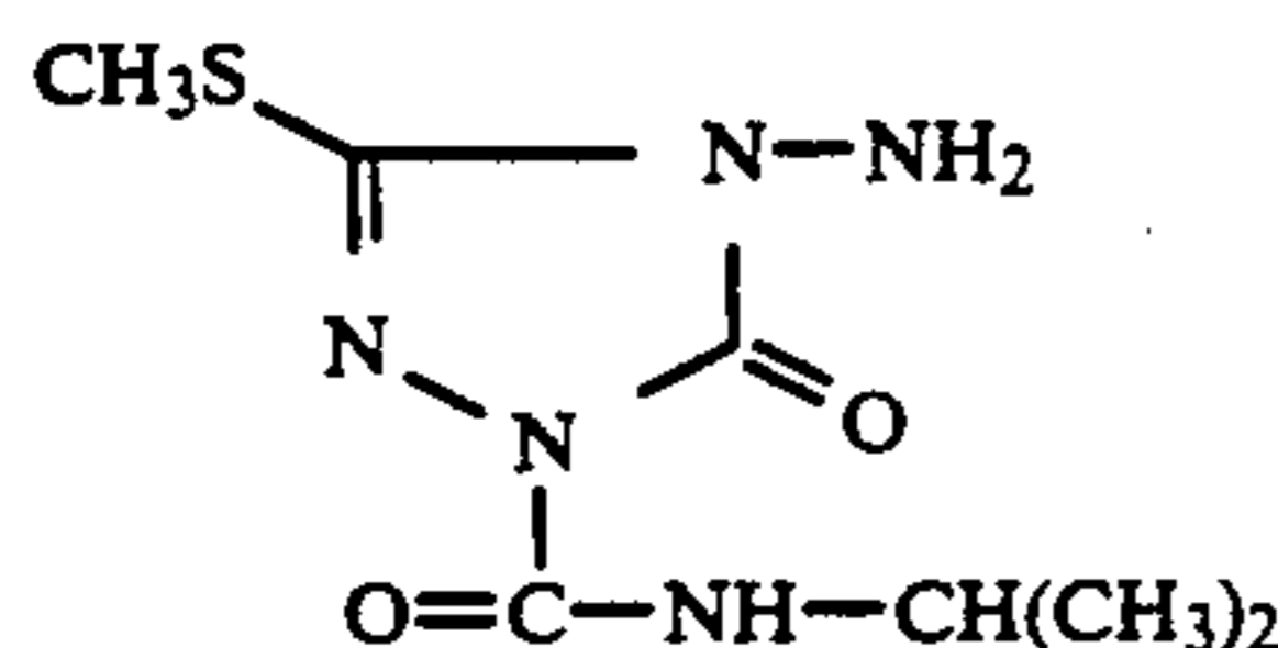
(C) 4-amino-1-(N-isopropylcarbamoyl)-3-methylthio-(1H,4H)-1,2,4-triazolin-5-one
