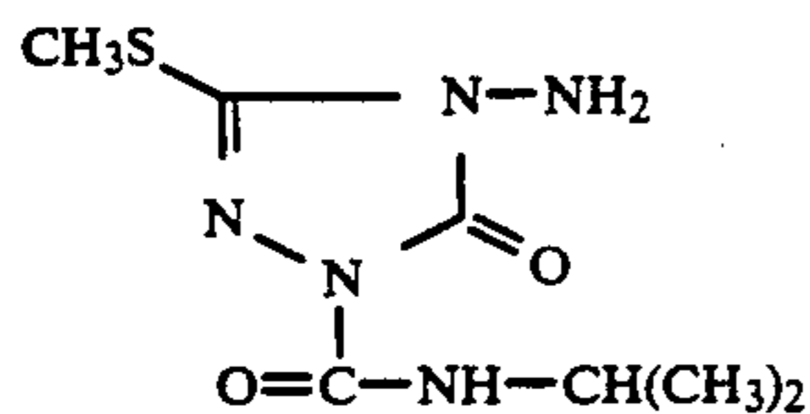
(C) 4-amino-1-(N-isopropylcarbamoyl)-3-methylthio-(1H,4H)-1,2,4-triazolin-5-one
