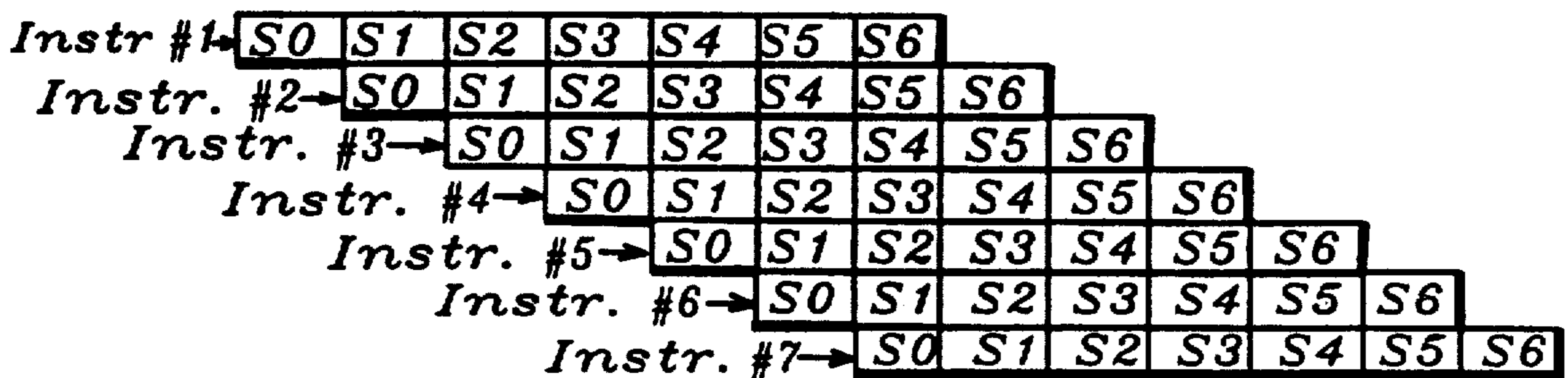
FIG 7 PIPELINE
