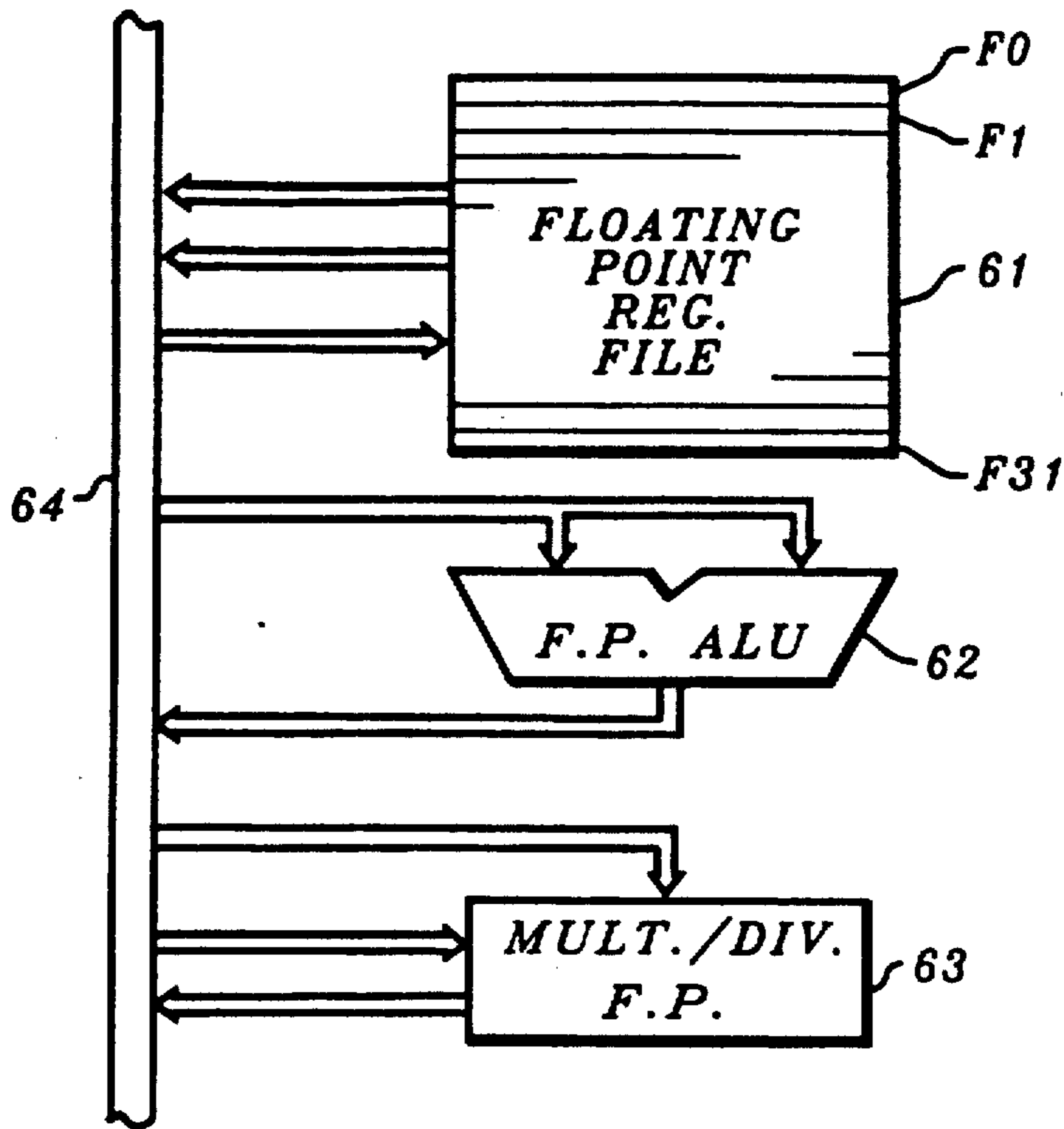
FIG 6 F-BOX
