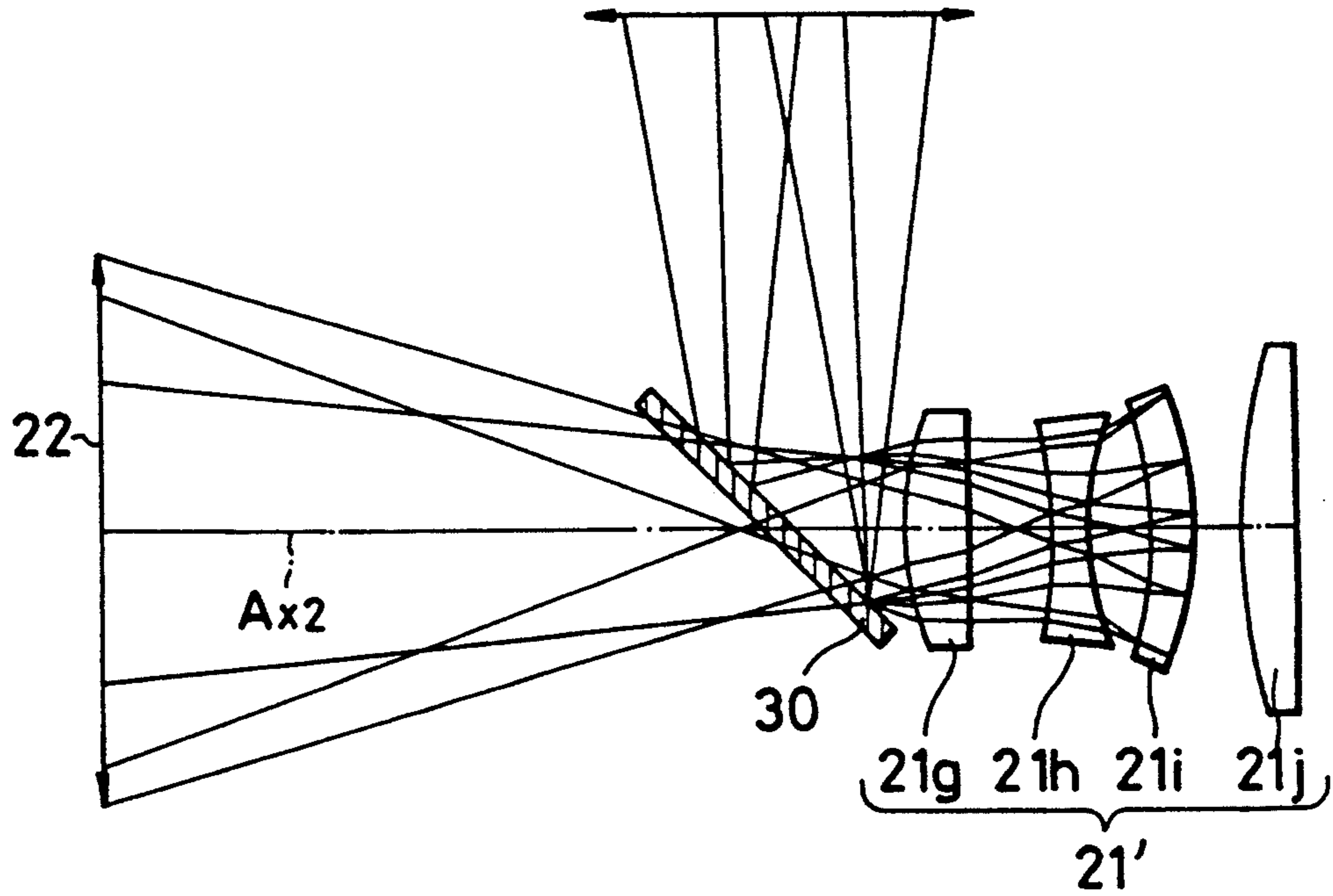
FIG. 25 PRIOR ART
