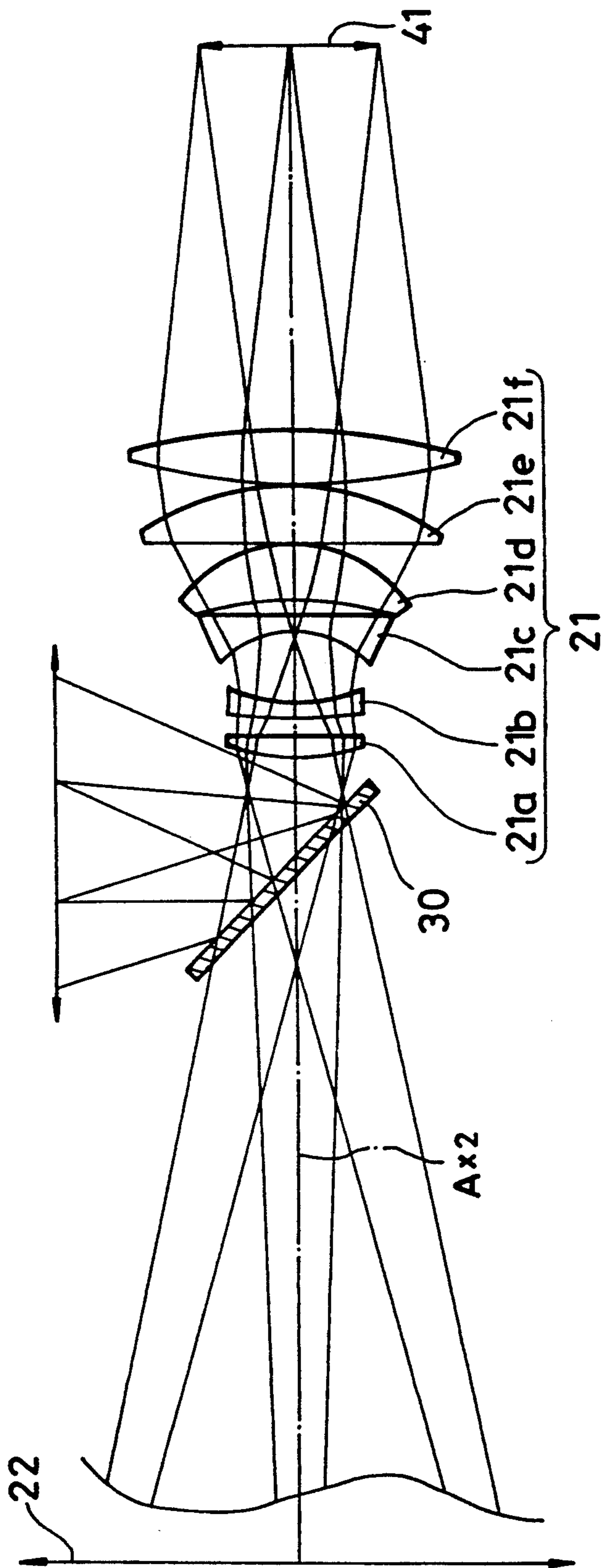
FIG. 21 PRIOR ART
