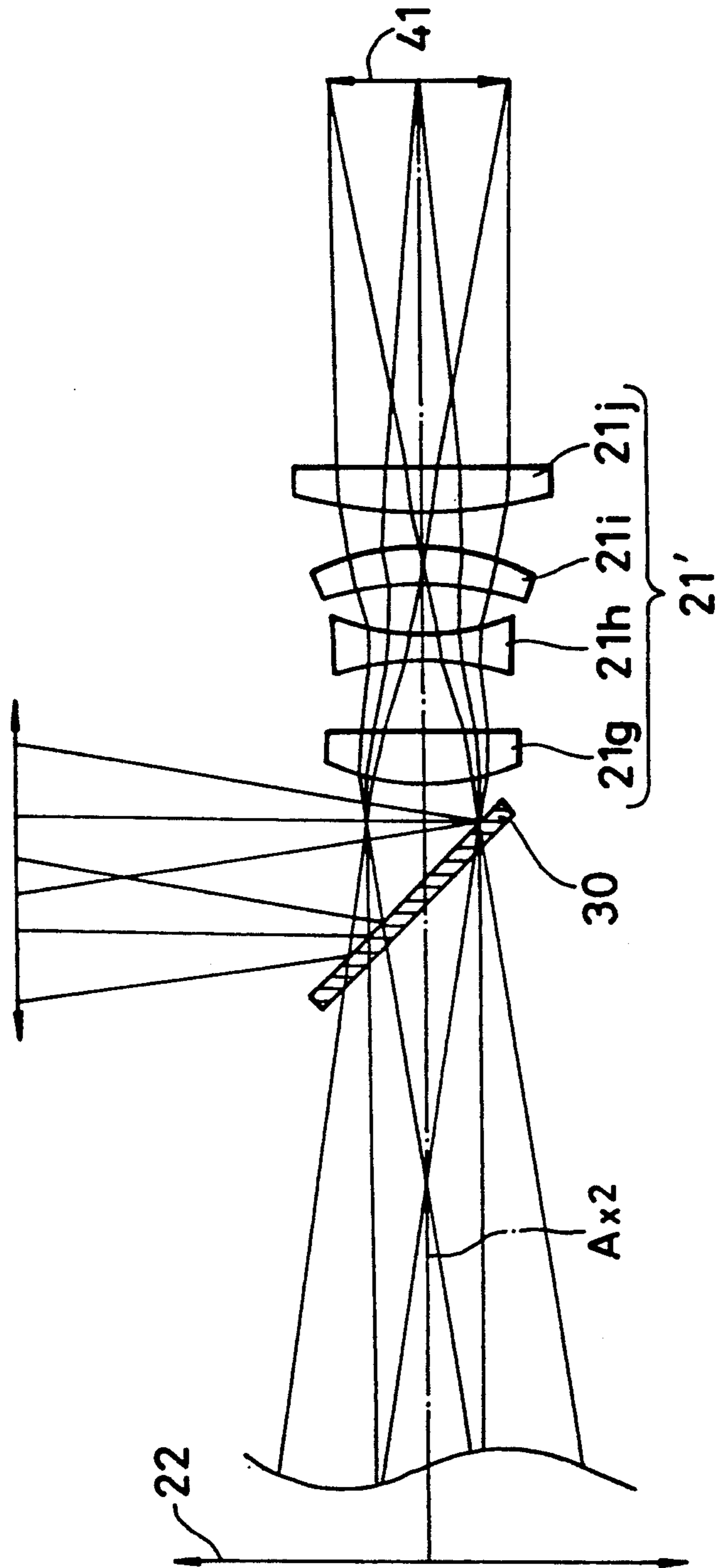
FIG. 24 PRIOR ART
