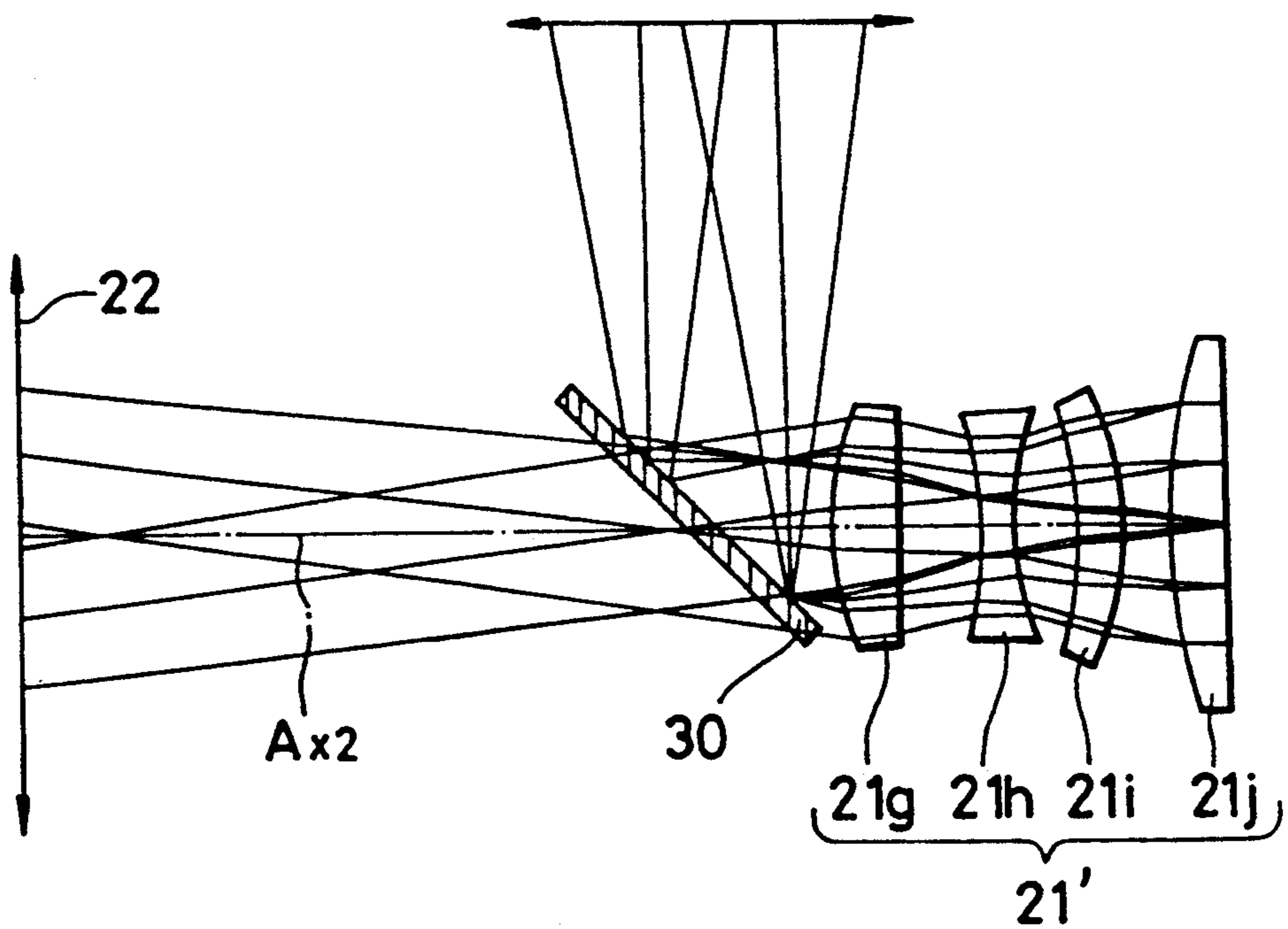
FIG. 26 PRIOR ART
