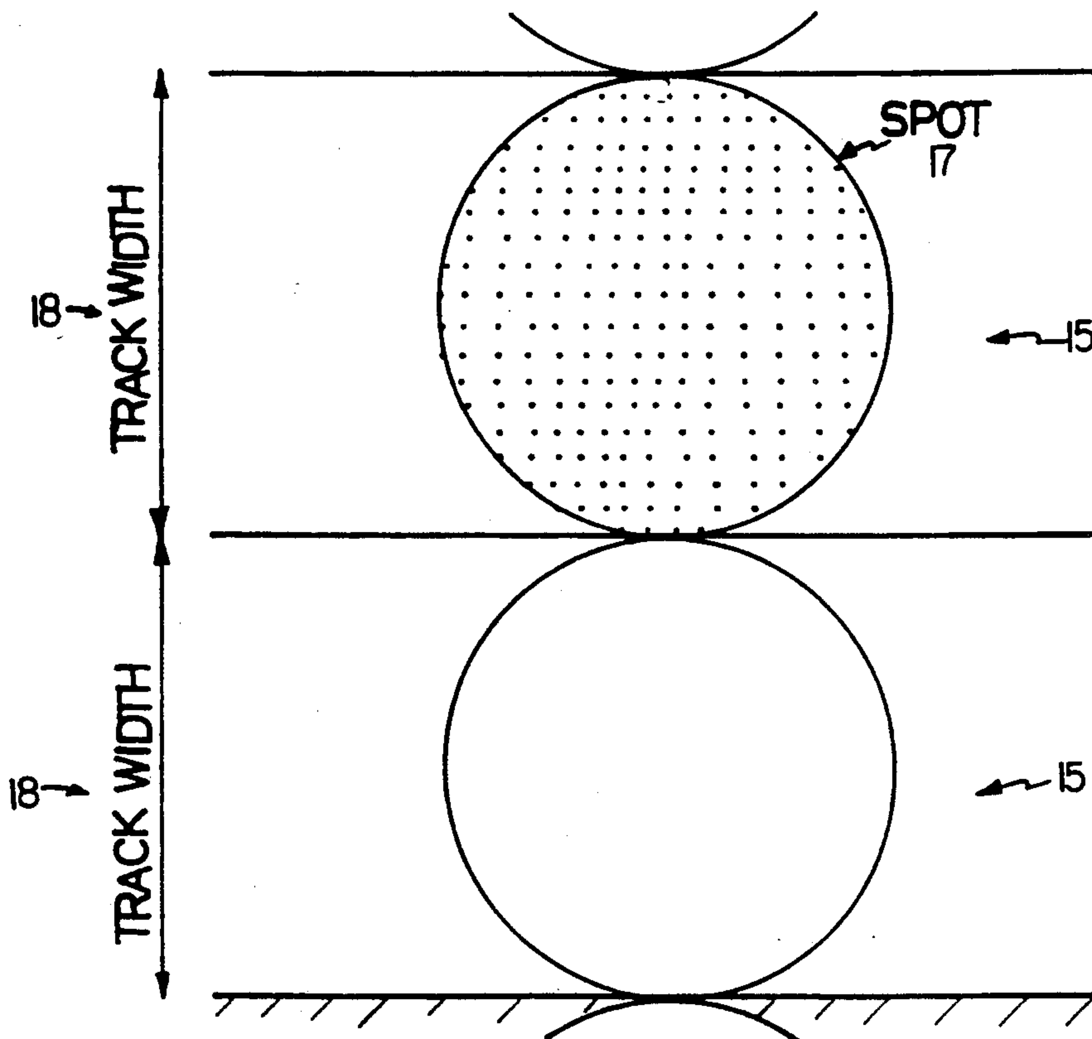
FIG. 3 (PRIOR ART)
