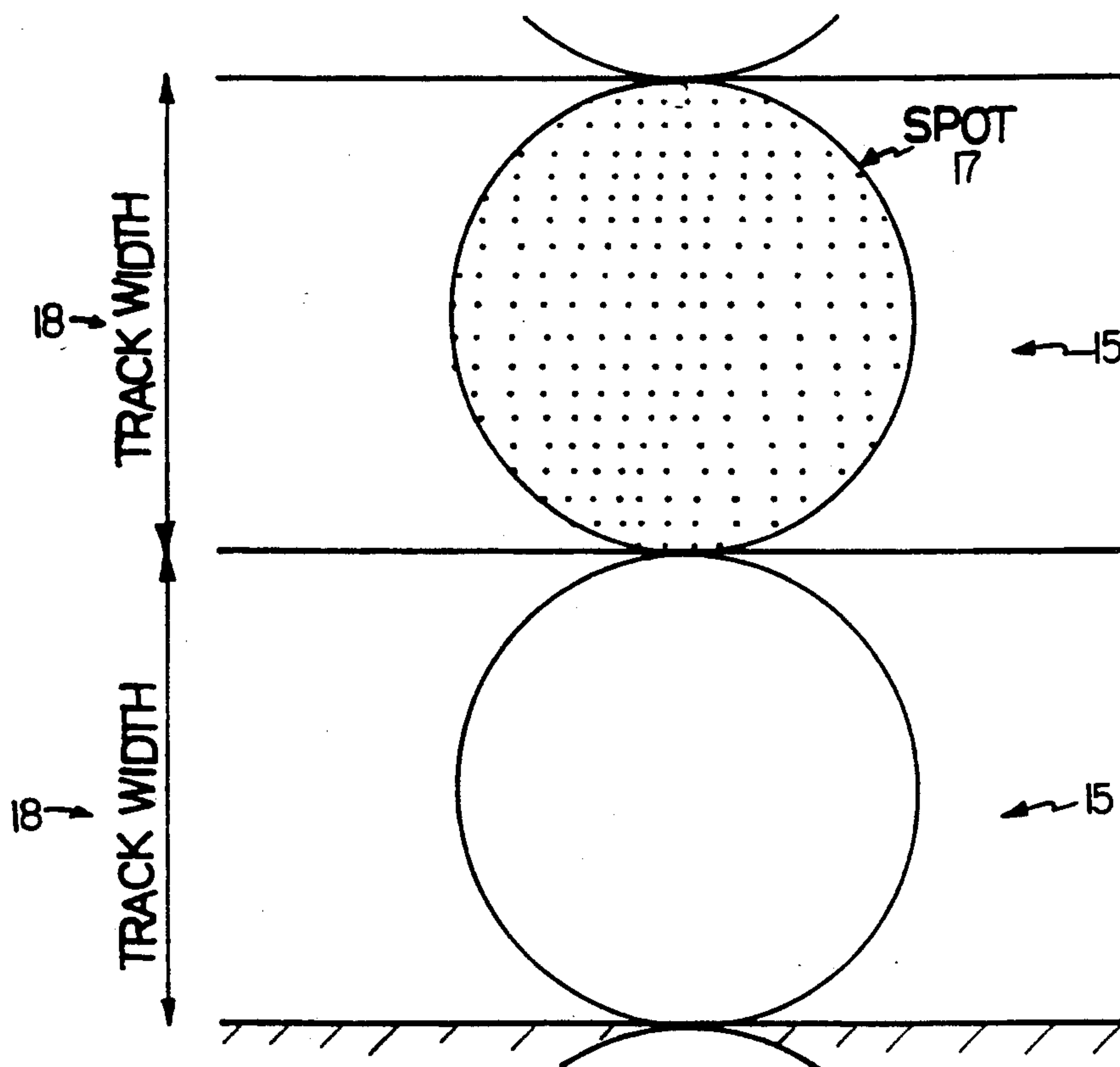
FIG. 3 (PRIOR ART)
