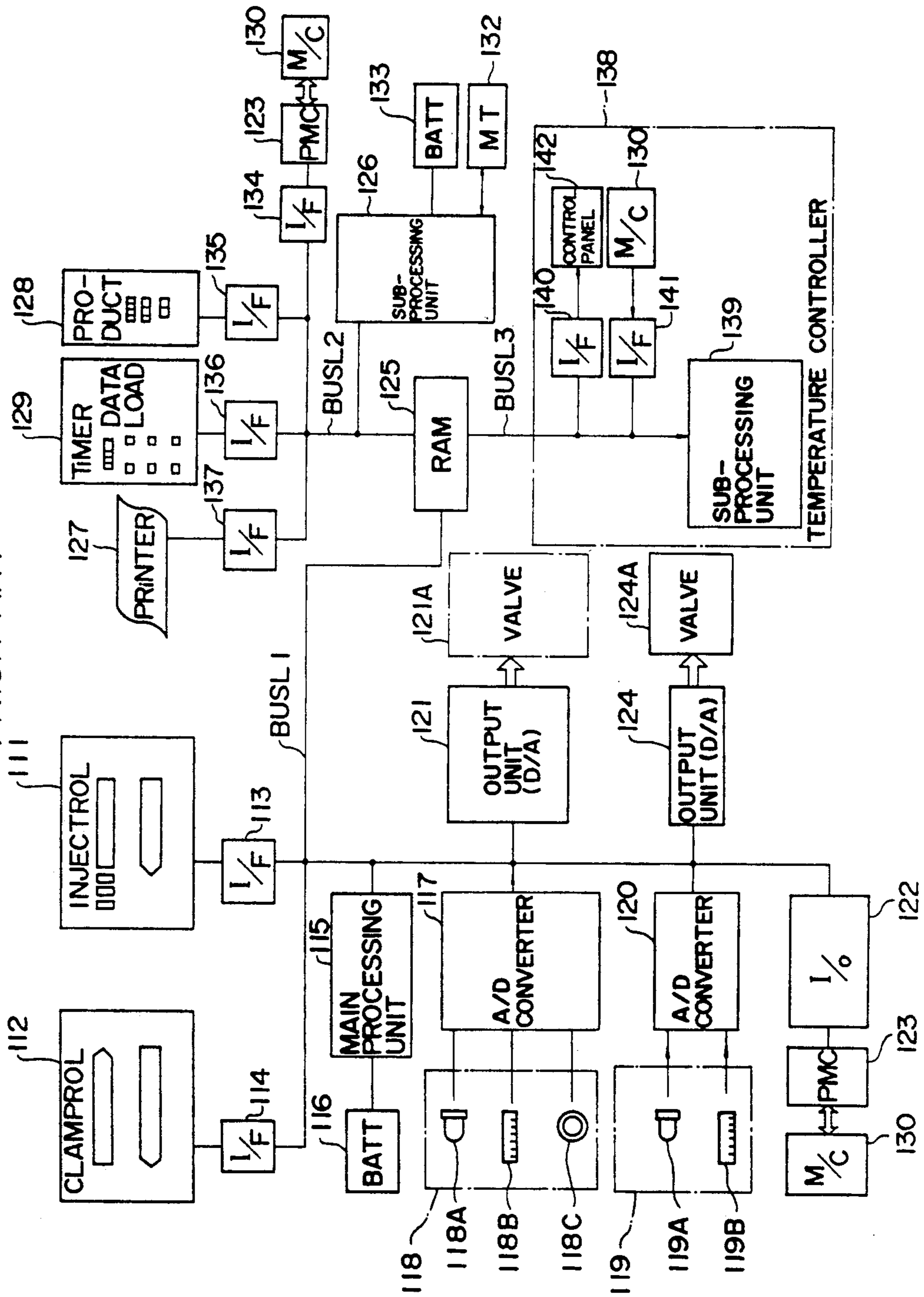
FIG. 9 PRIOR ART
