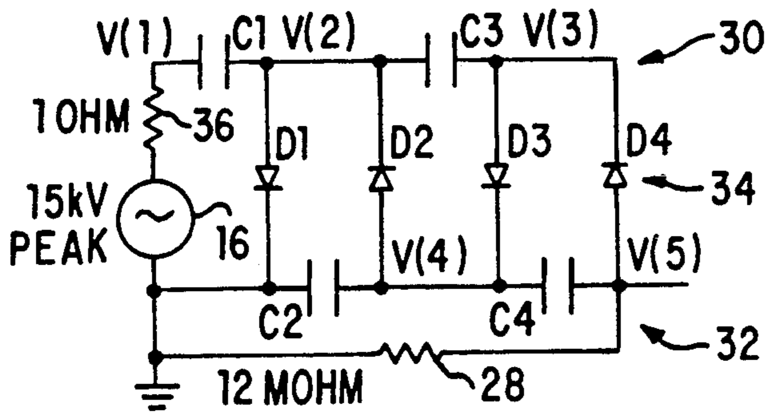
FIG. 2 PRIOR ART
