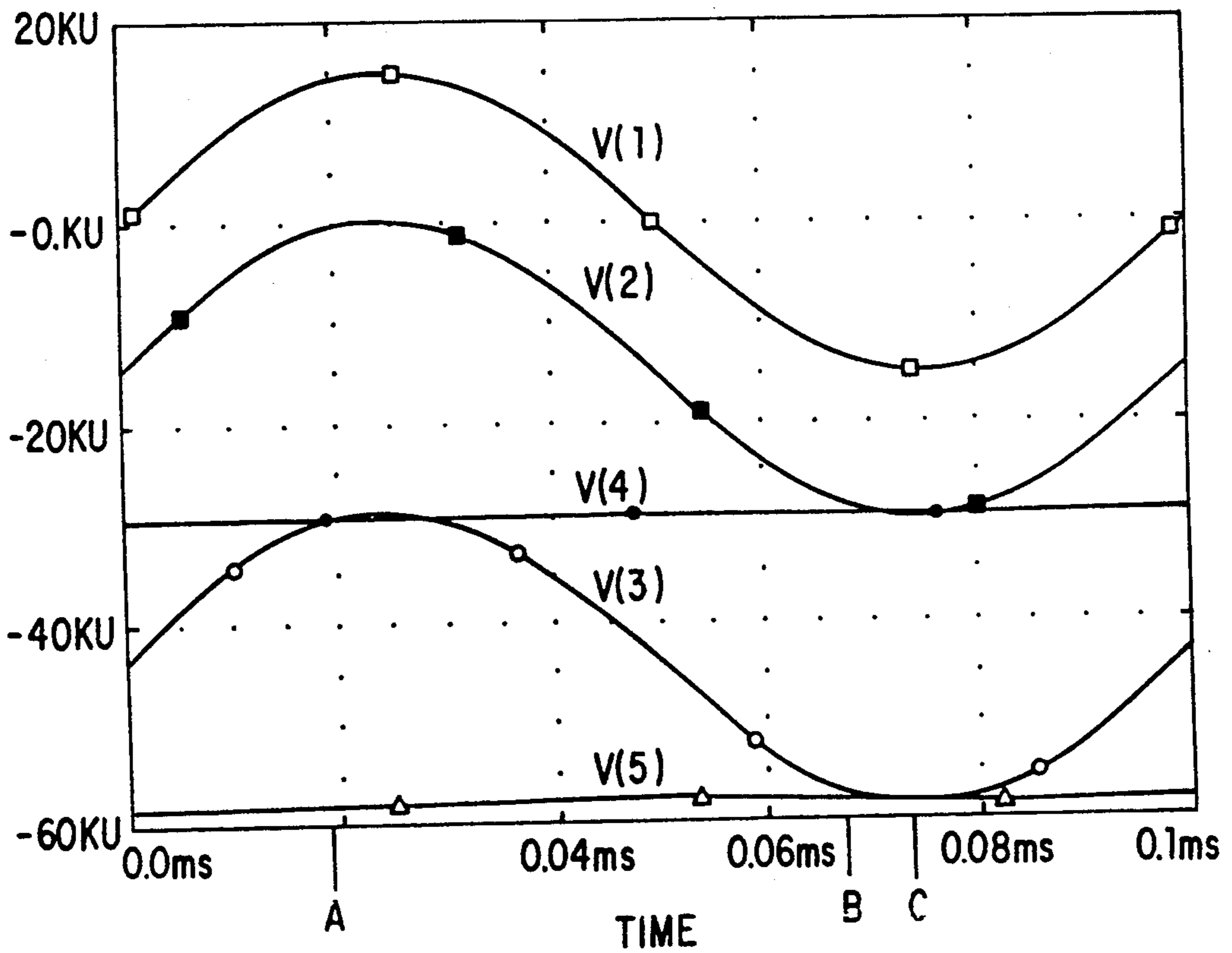
FIG. 3 PRIOR ART
